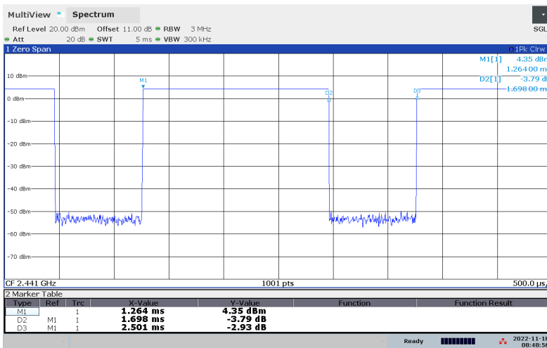
RF Burst, DH3
