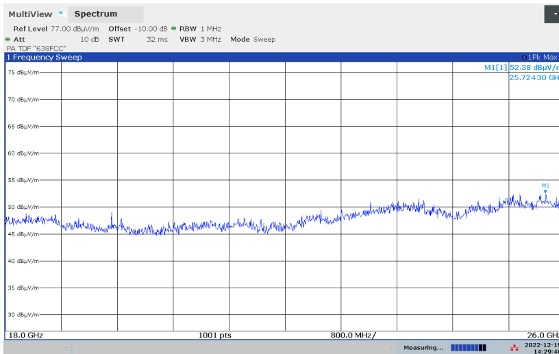
Pre-scan 18 - 26 GHz, 2441 MHz, \pi/4 -DQPSK, HP, @10cm
