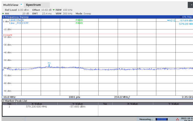
Conducted Emissions 10-2350 MHz, 2402 MHz, GFSK
