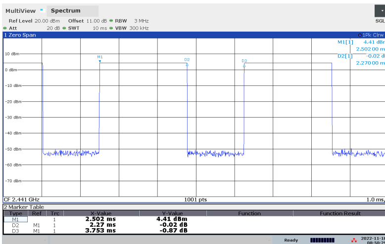
RF Burst DH5
