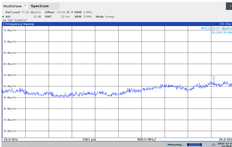
Pre-scan 18 - 26 GHz, 2441 MHz, GFSK, HP, @10cm
