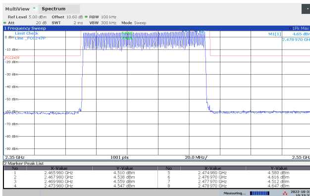
Conducted Emissions 2350-2550 MHz, Hopping, GFSK
