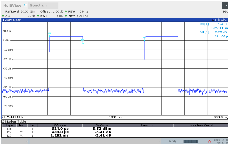
RF Burst, DH1
