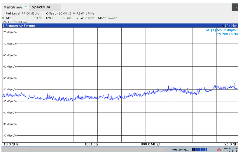
Pre-scan 18 - 26 GHz, 2441 MHz, 8-DPSK, HP, @10cm
