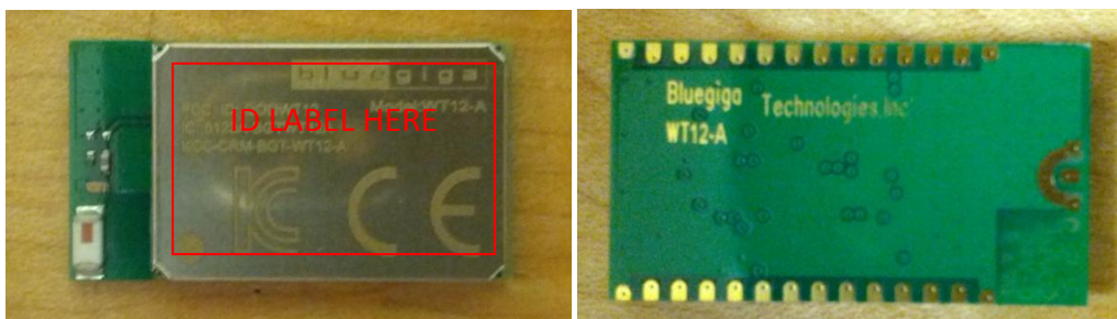
Figure 3 - WT12 Module. Top (left) and Bottom (right)
