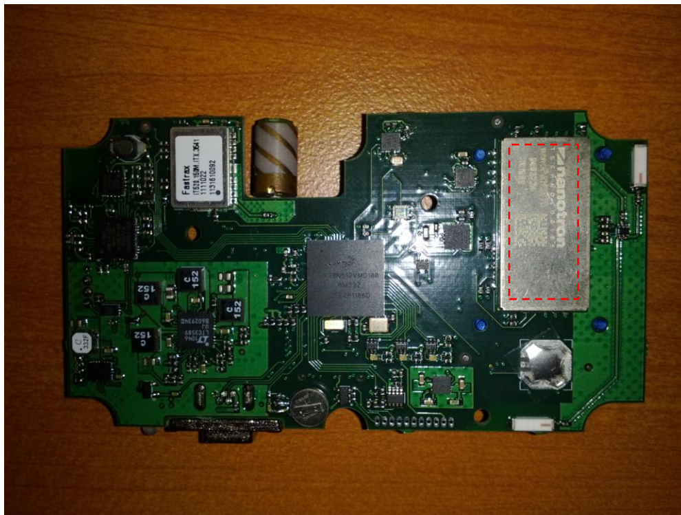
Figure 2 - TRX device showing label location for BXONNT5375-1000 module with dashed red line.
