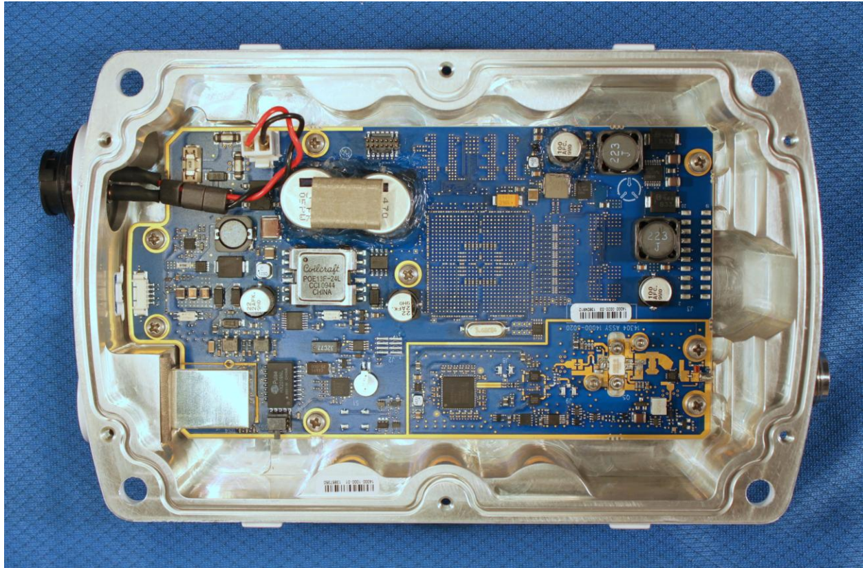
Figure 1: Internal View of PCB in Chassis
