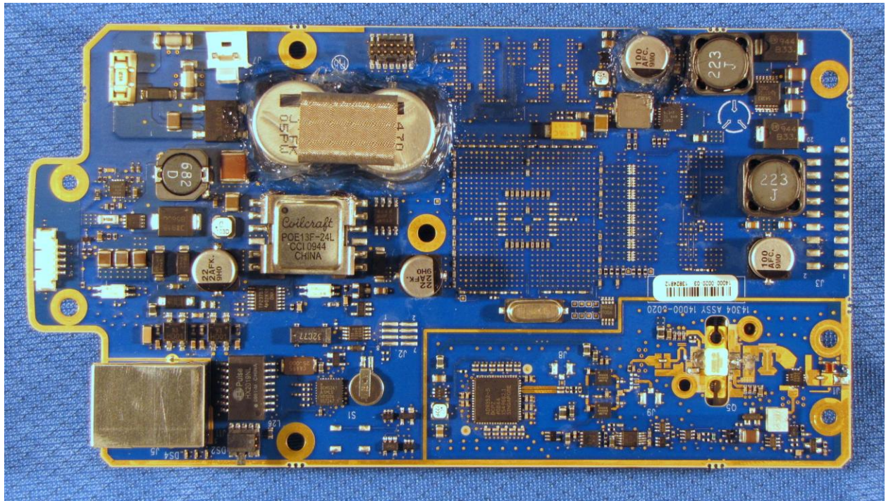
Figure 2: PCB Top Side of Board
