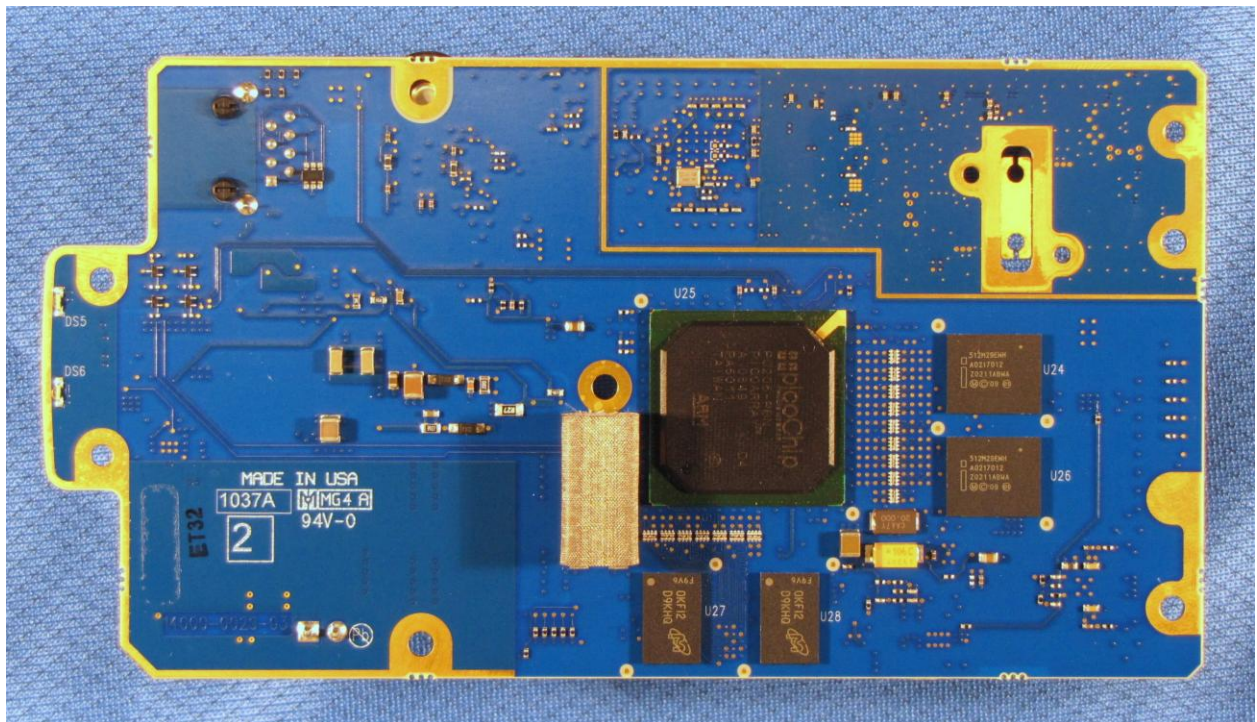
Figure 3: PCB Bottom Side of Board
