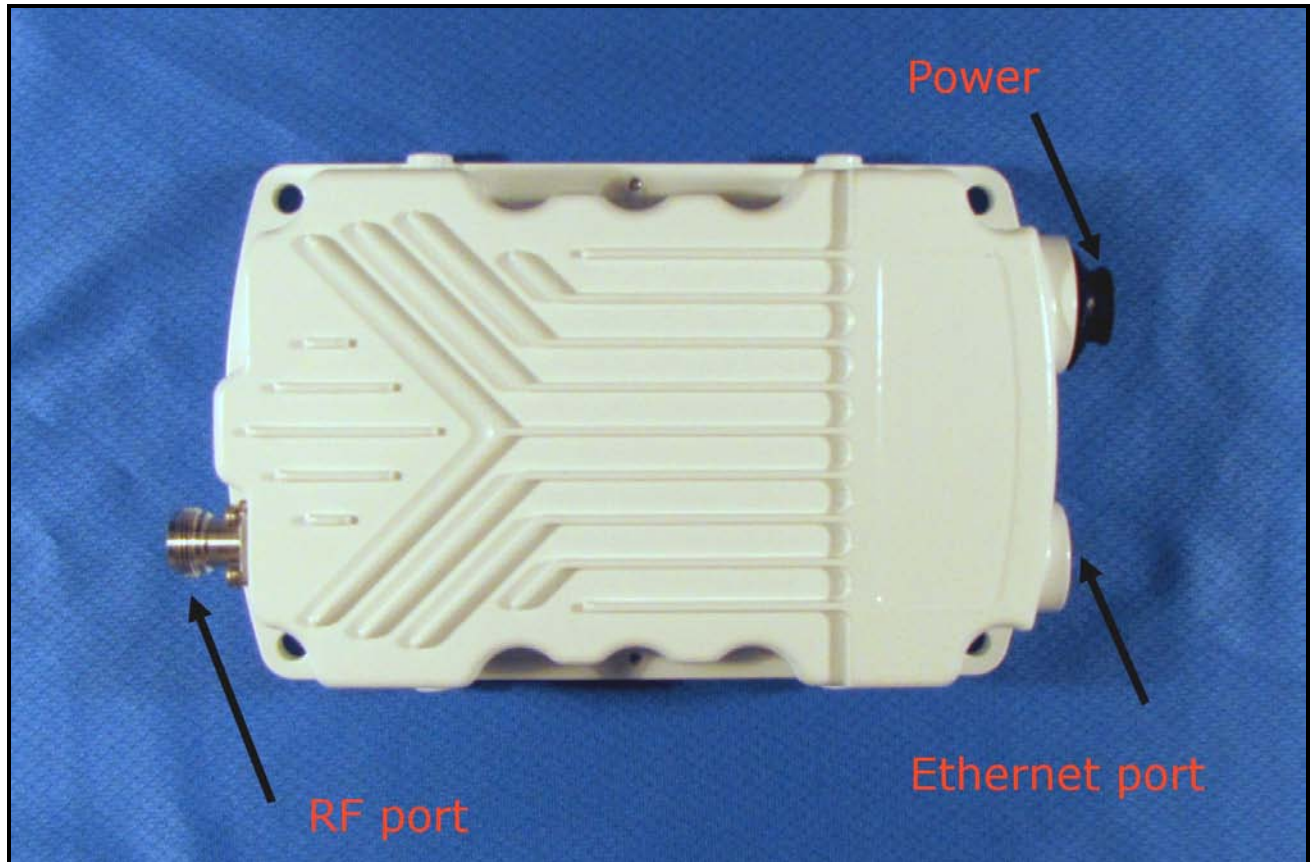
Photograph 6: Bottom, Ports Labeled
