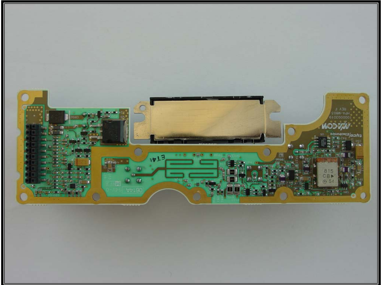
Photograph 4: Solder Side
