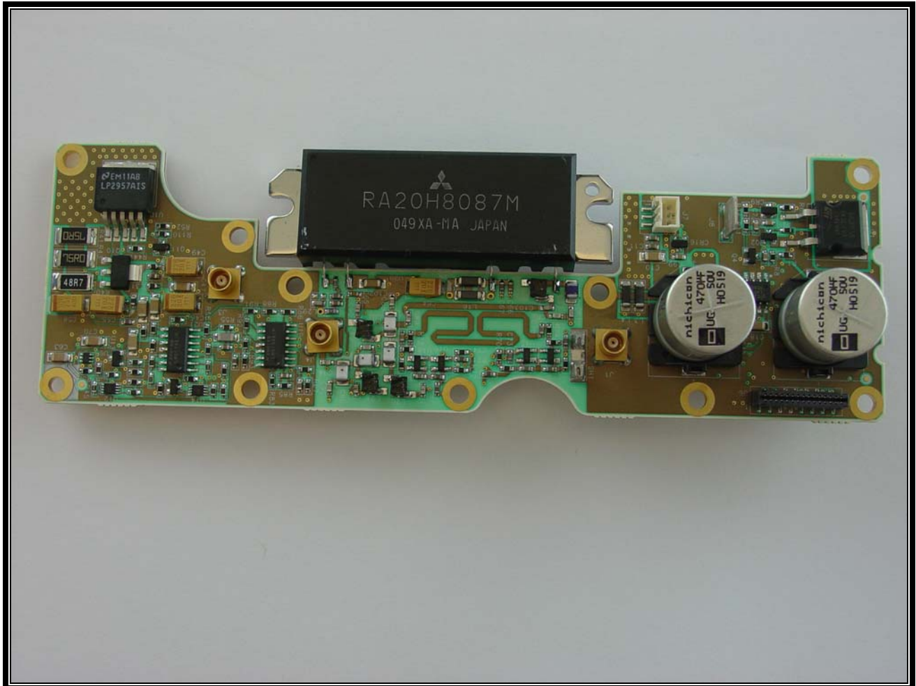
Photograph 3: Component Side
