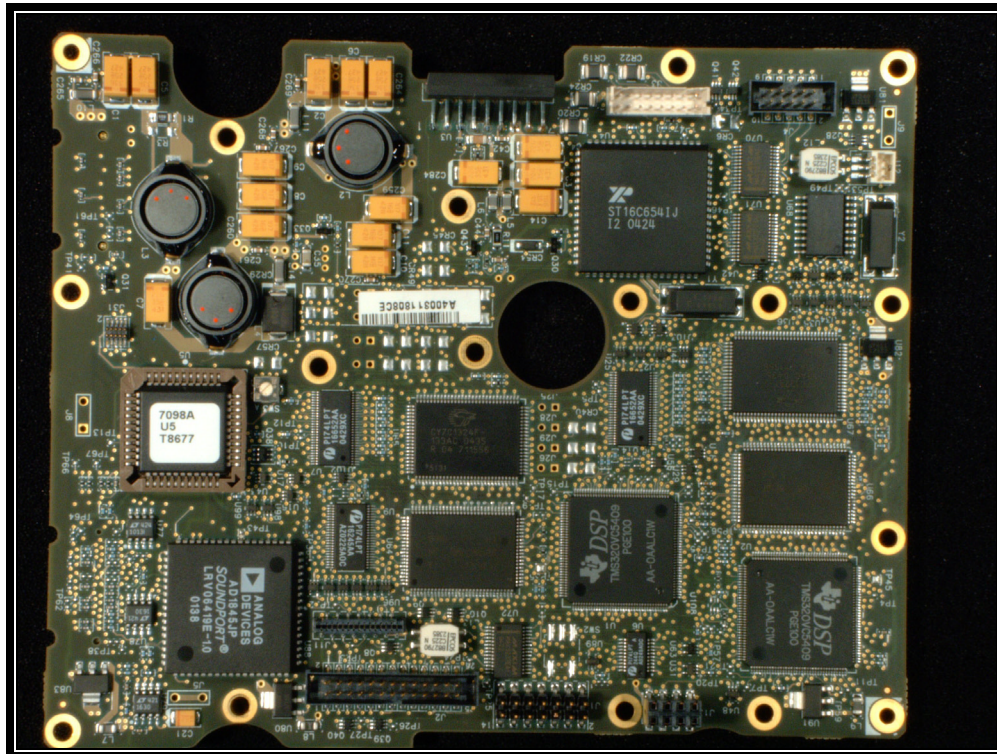
PHOTOGRAPH 14: PK PCB TOP VIEW
