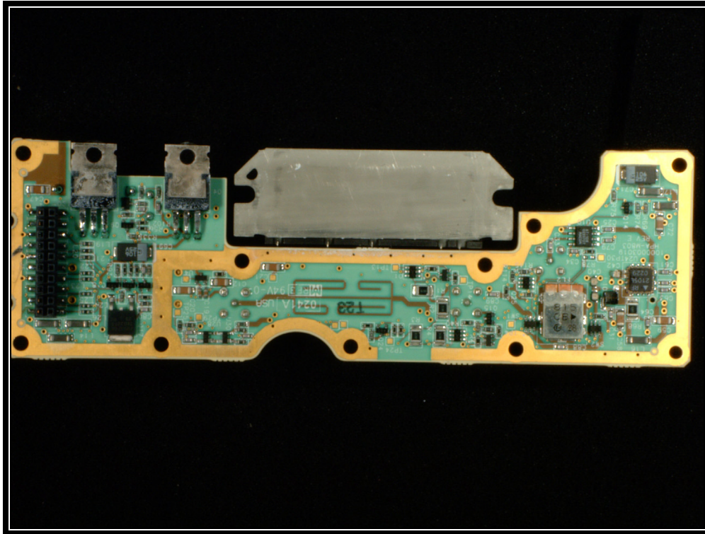
PHOTOGRAPH 13: HPA PCB BOTTOM VIEW
