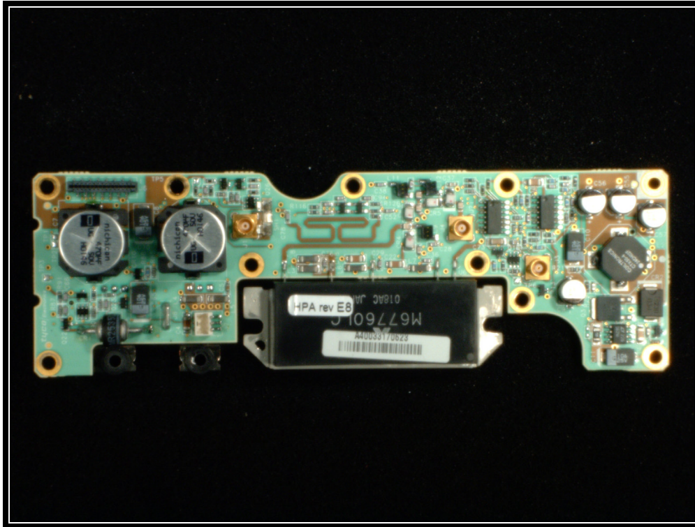
PHOTOGRAPH 12: HPA PCB TOP VIEW
