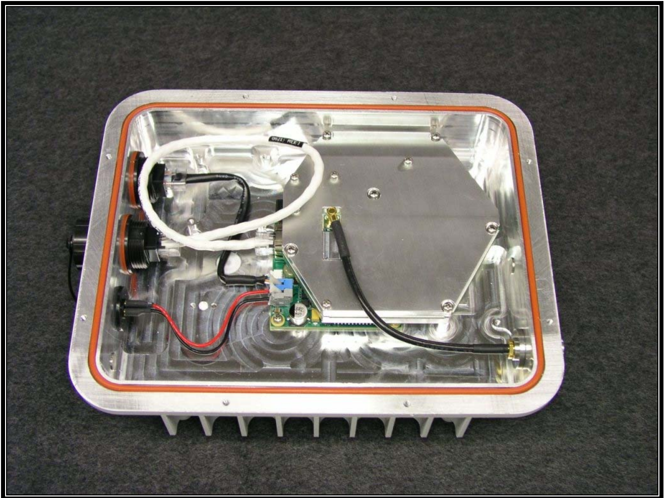
Photograph 15: Open Chassis – AC Version
