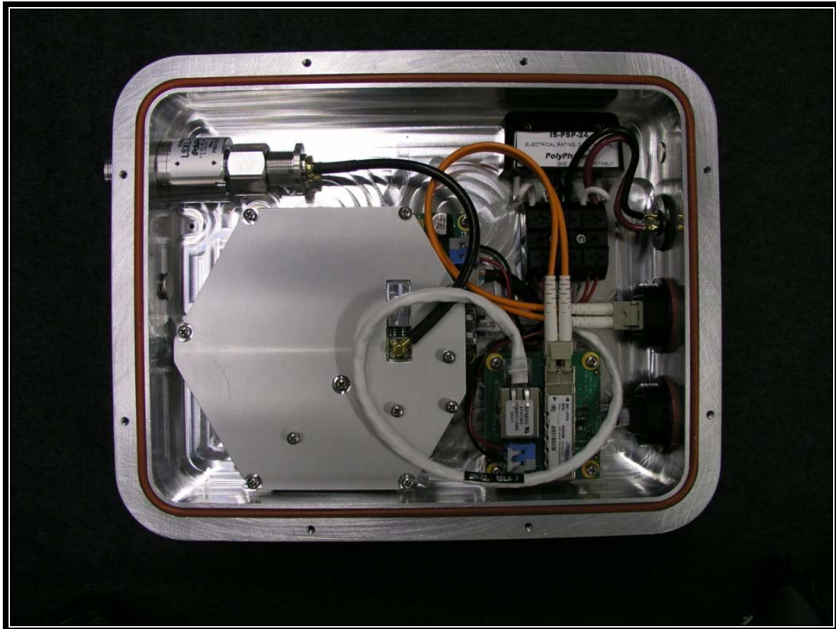
Photograph 14: Open Chassis - Hardened Version
