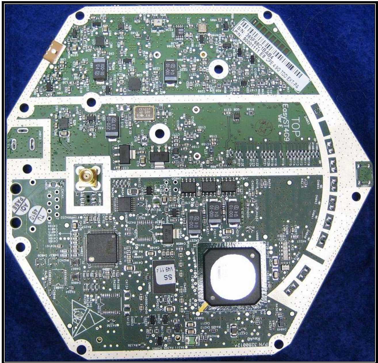
Photograph 16: PCB XCVR Top View
