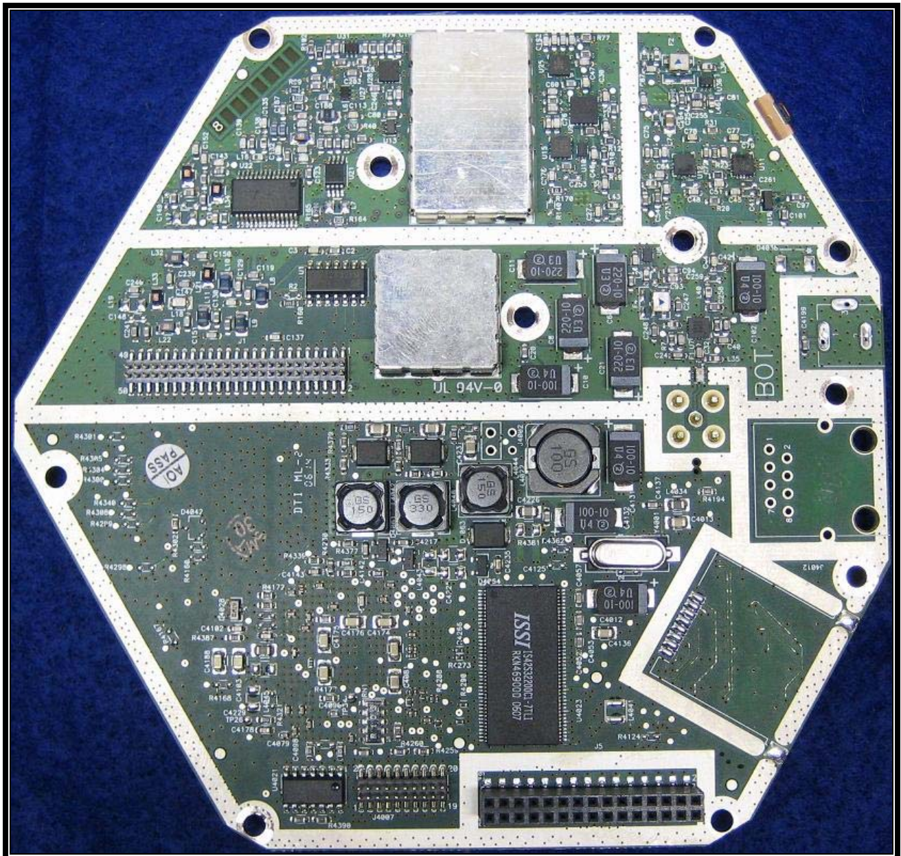
Photograph 17: PCB XCVR Bottom View
