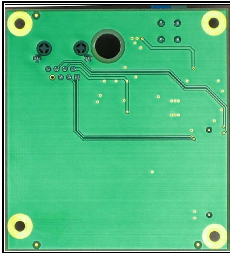
Photograph 19: PCB PWR&COM Bottom View
