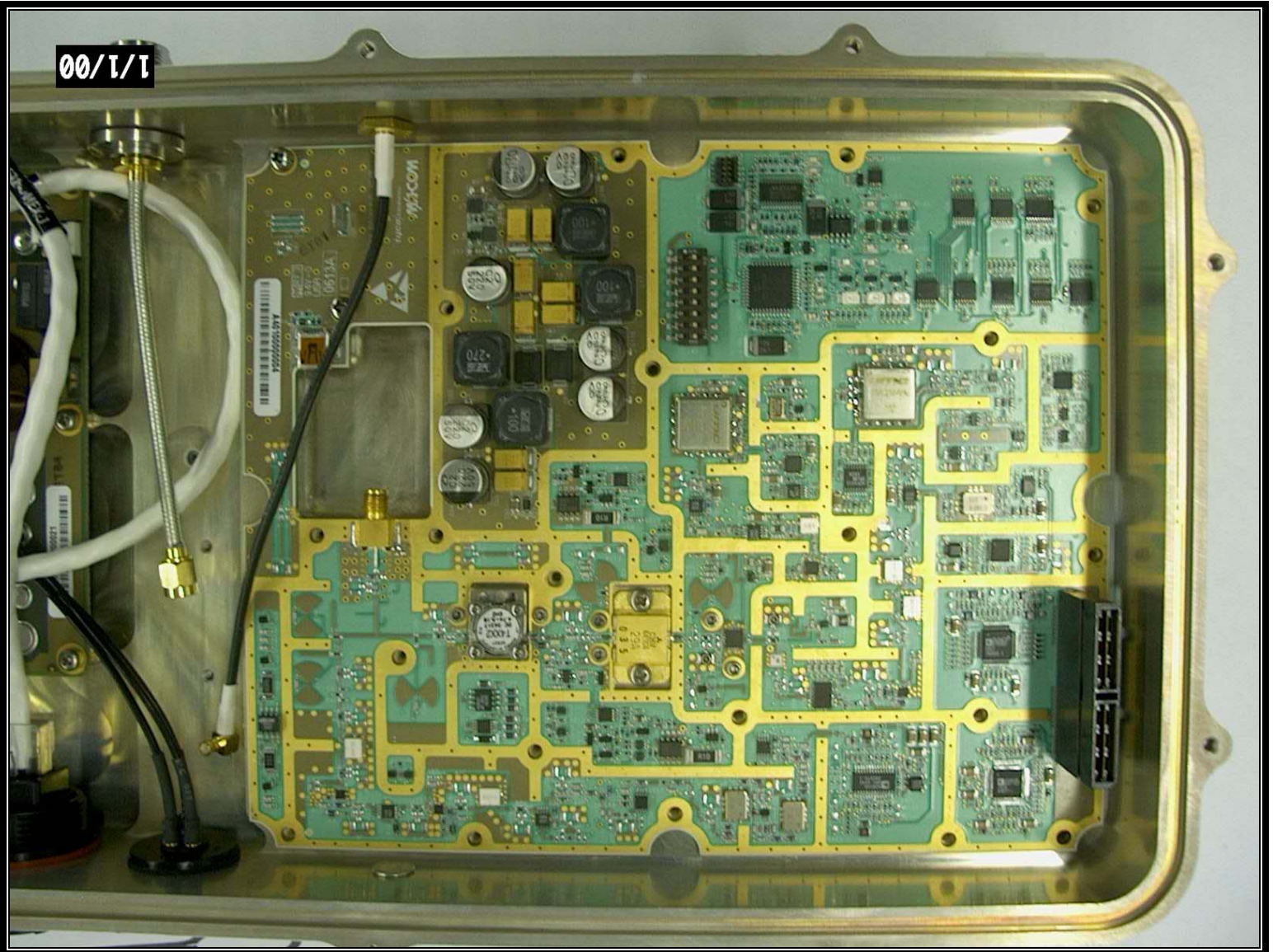
XCVR Chassis Without Cover
