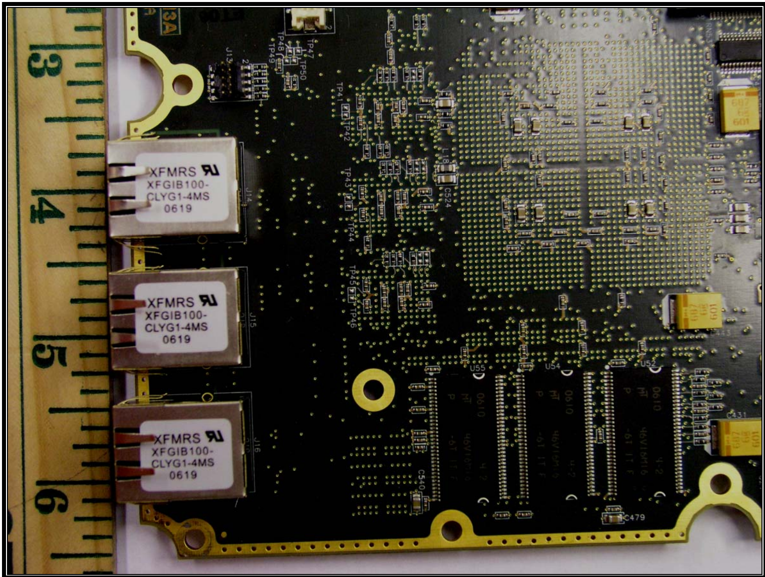
Digital Bottom 2
