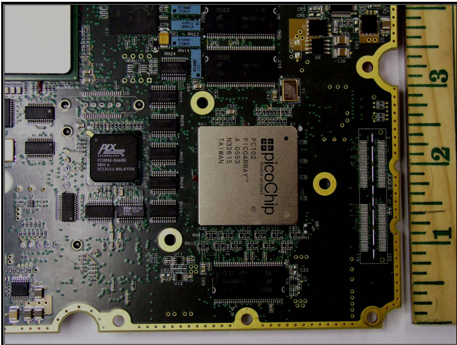
Digital Top 1
