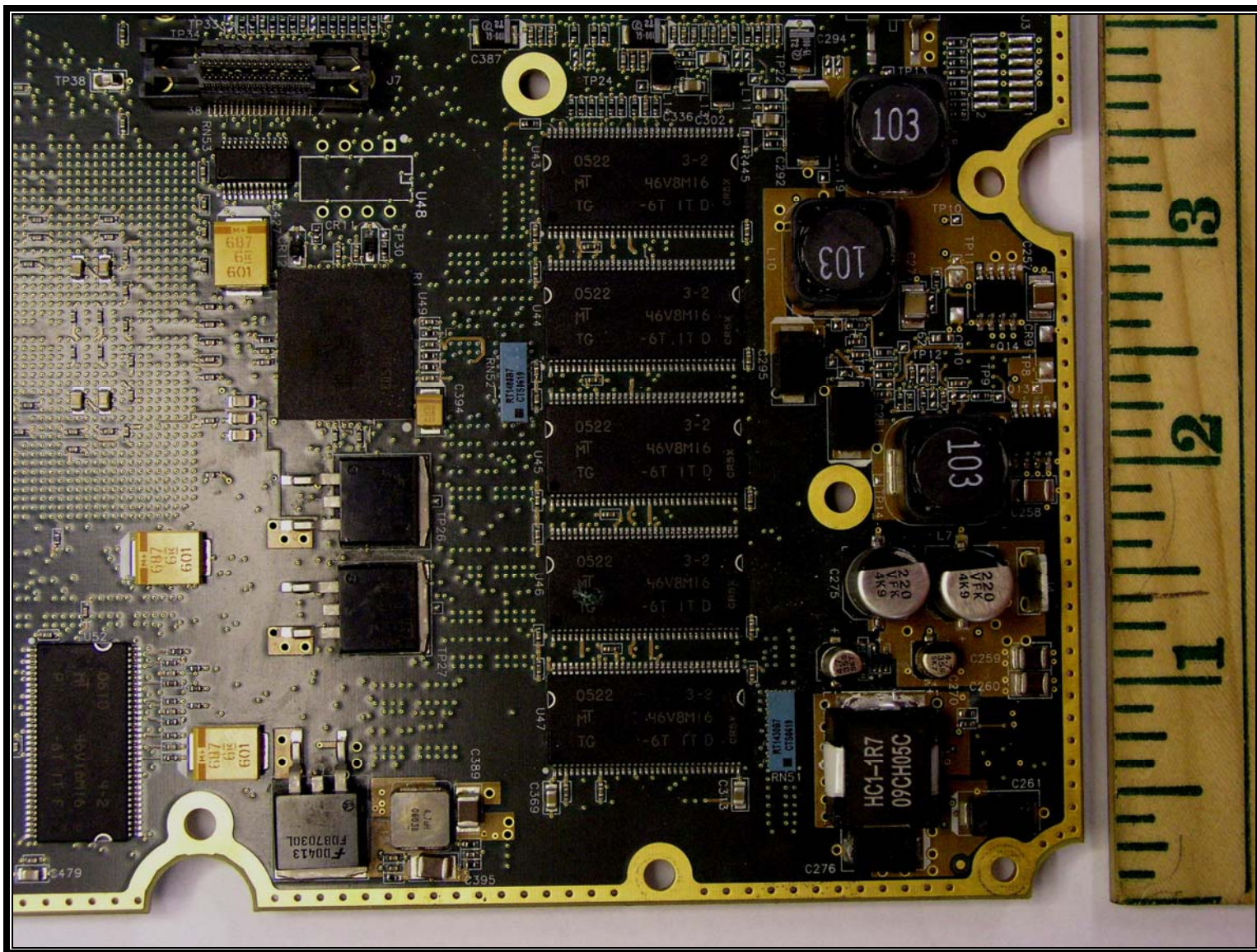
Digital Bottom 1
