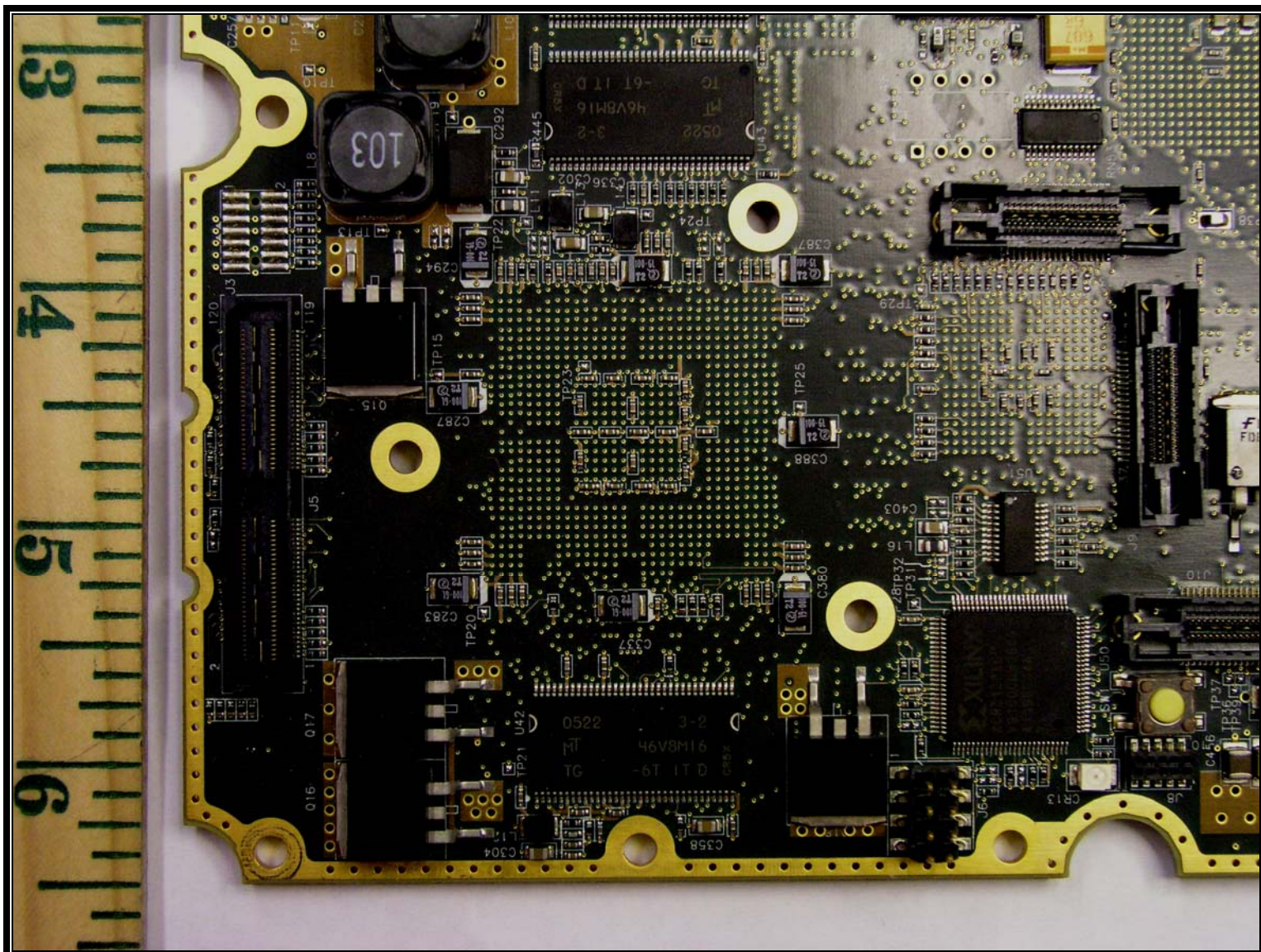
Digital Bottom 3
