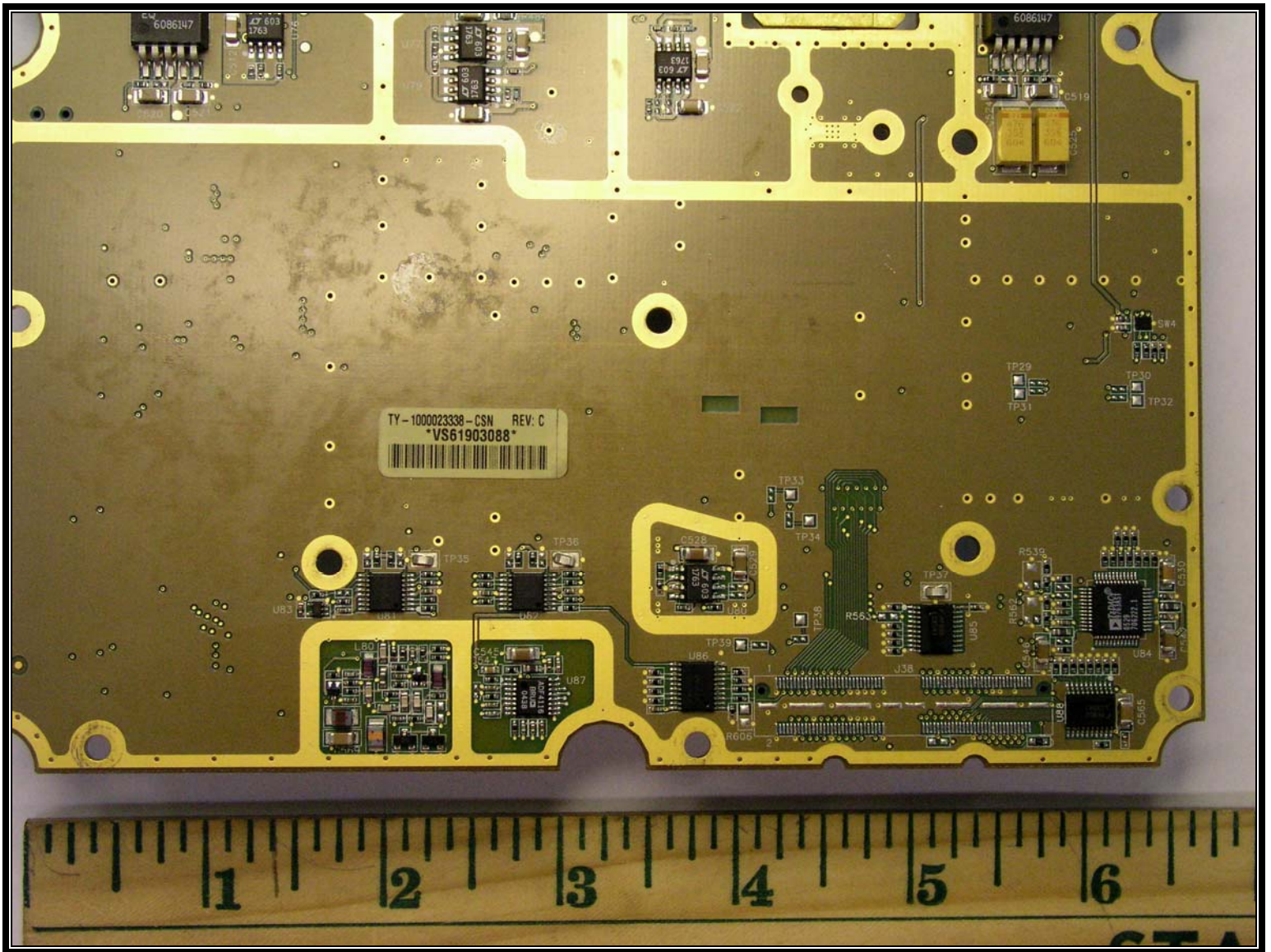
XCVR Bottom 2
