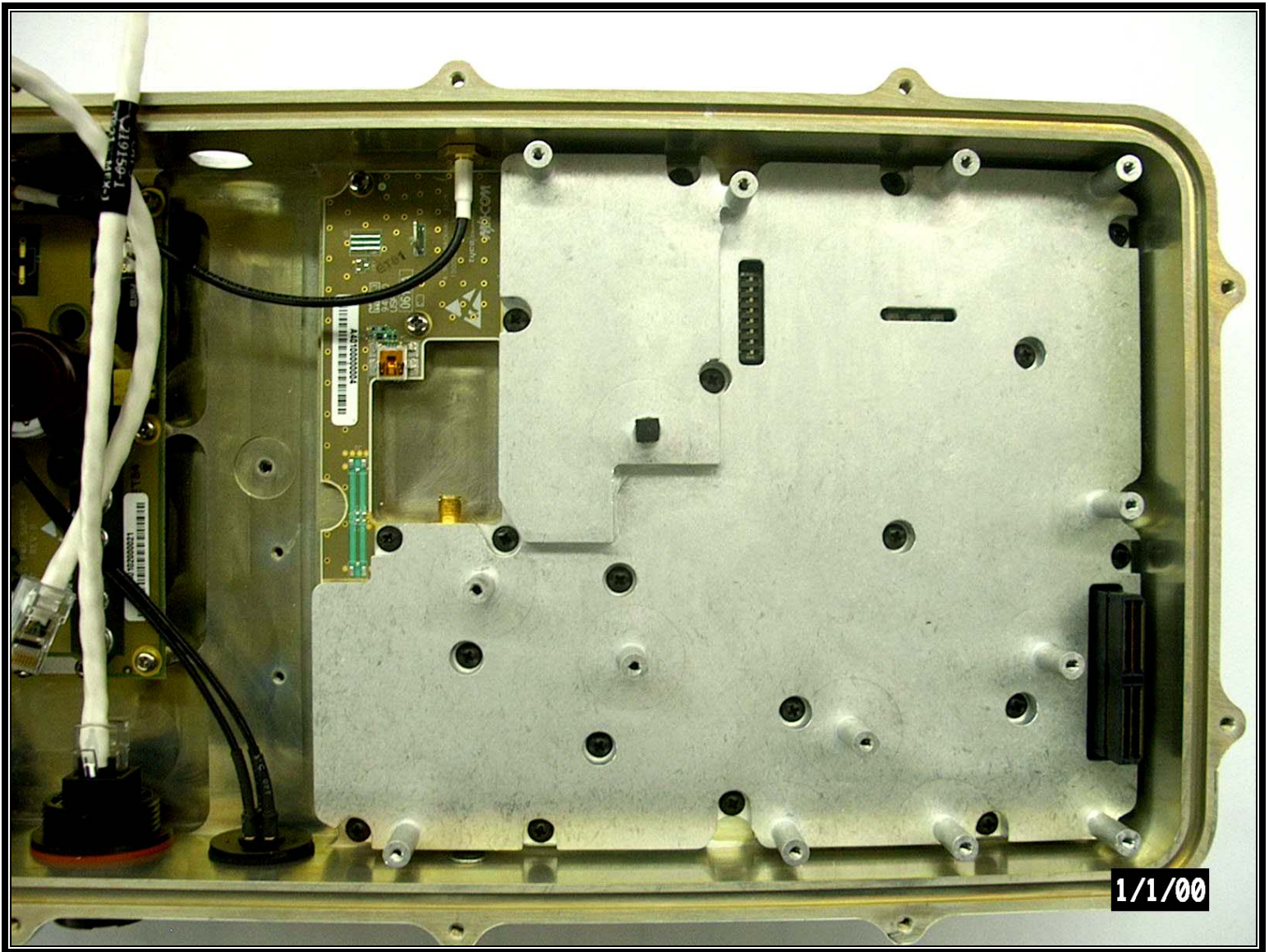
XCVR Chassis With Cover
