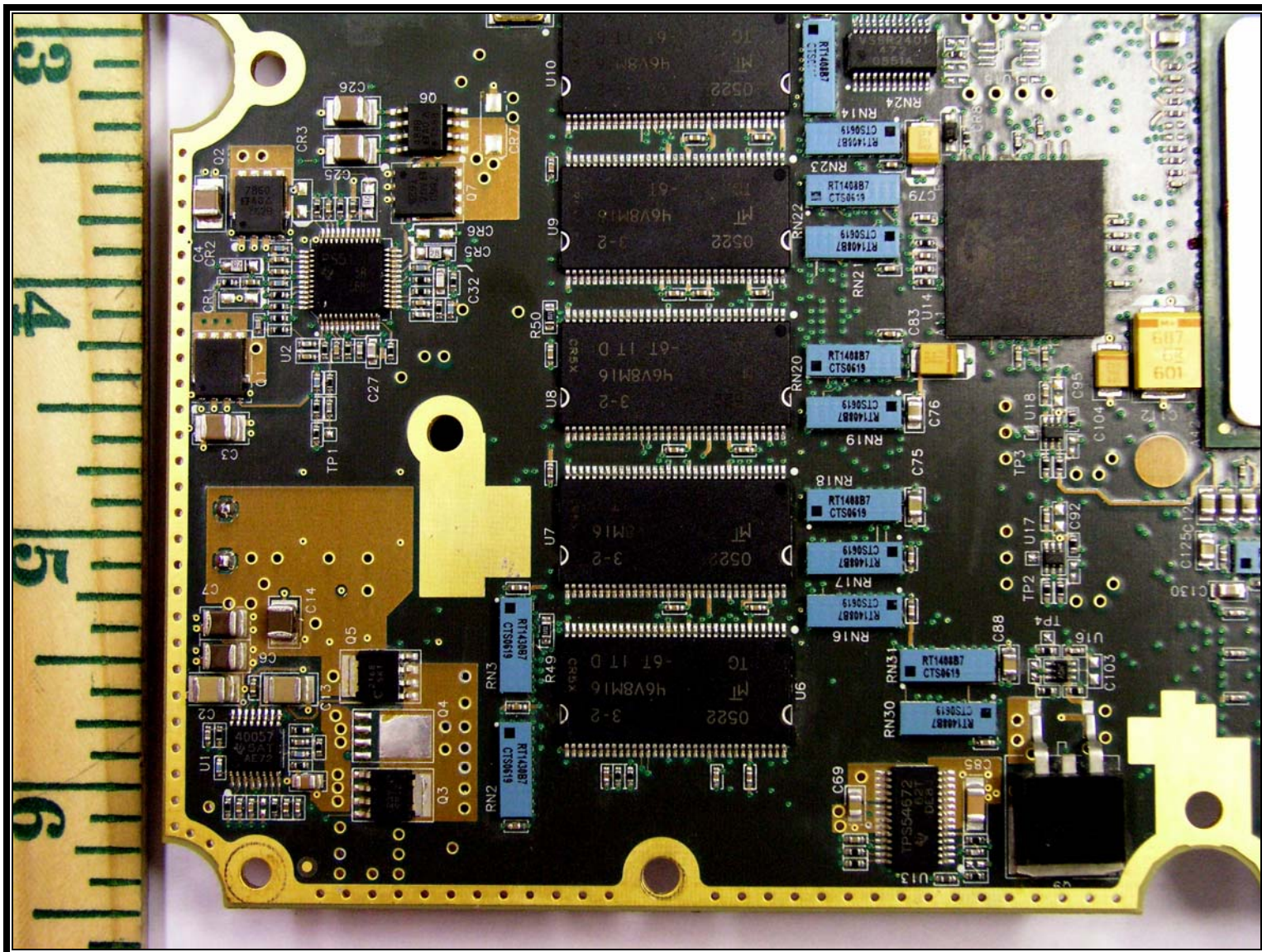
Digital Top 2
