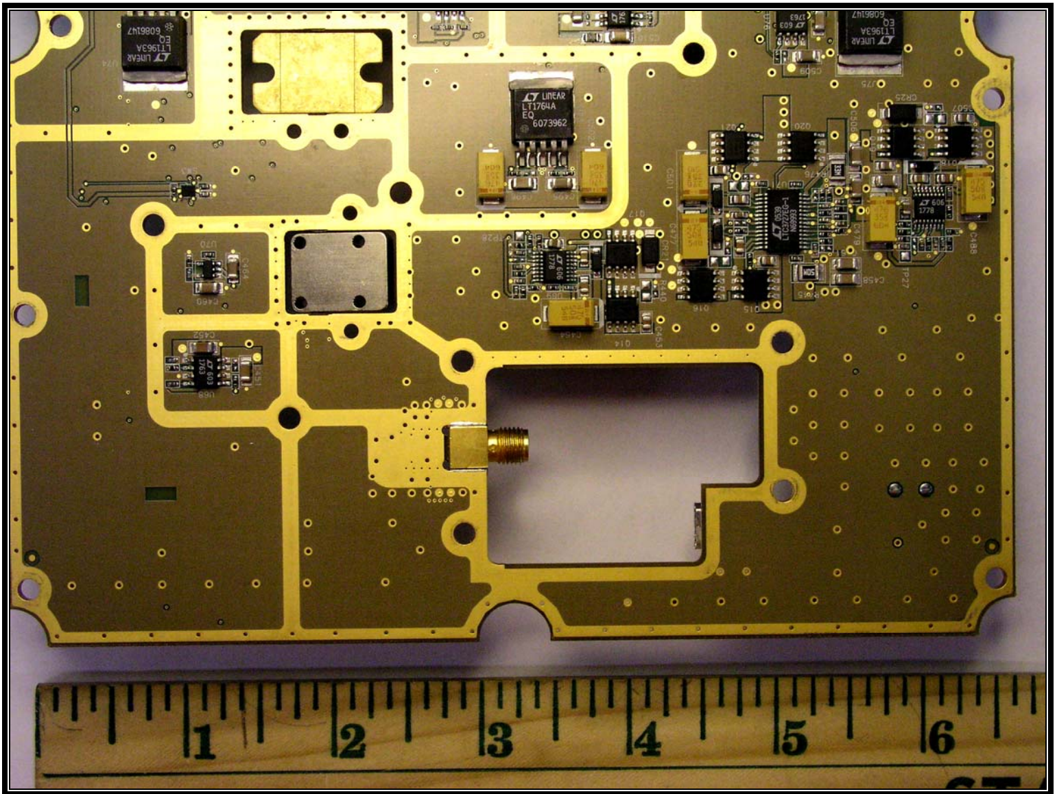
XCVR Bottom 1
