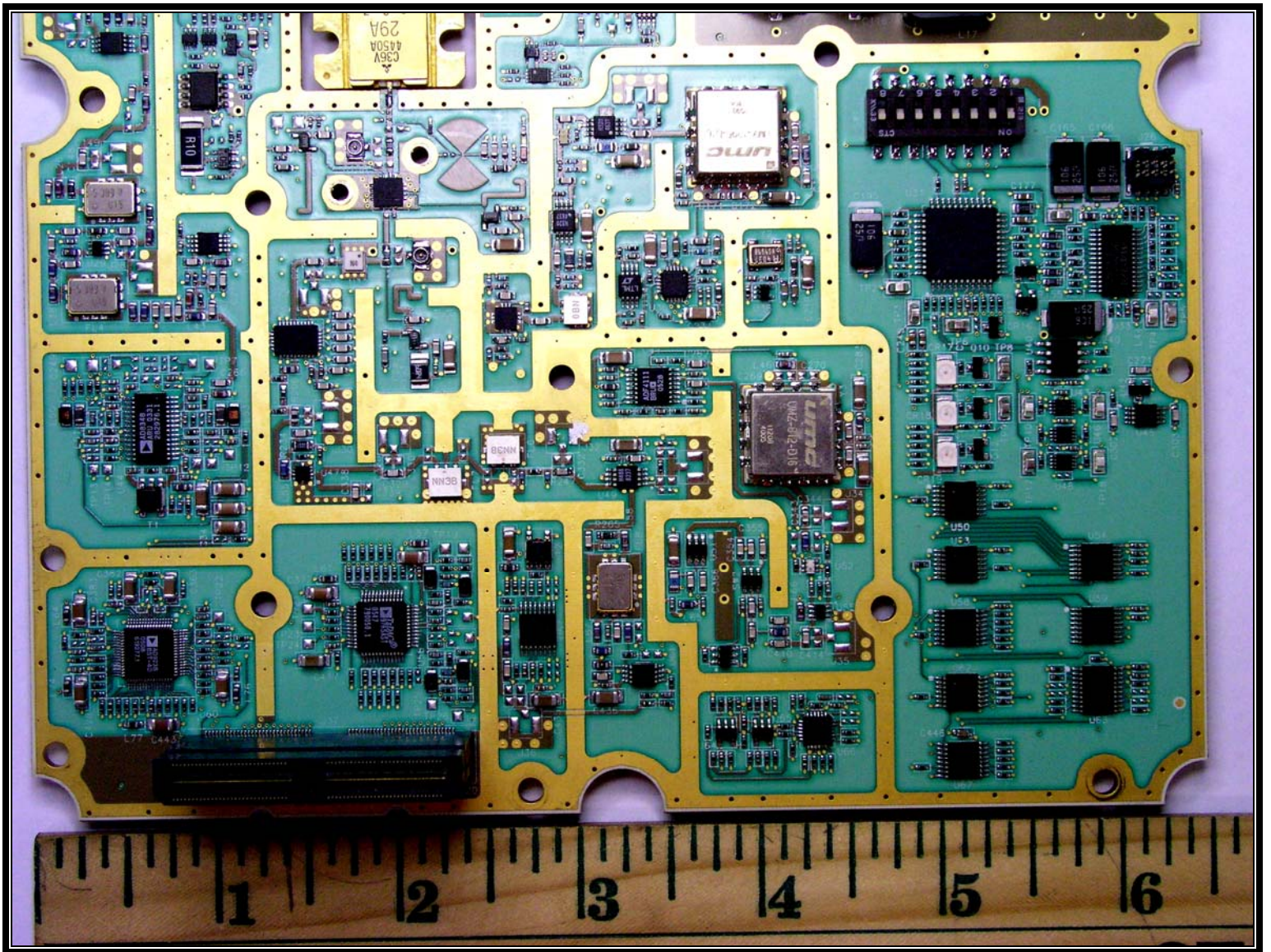
XCVR Top 2
