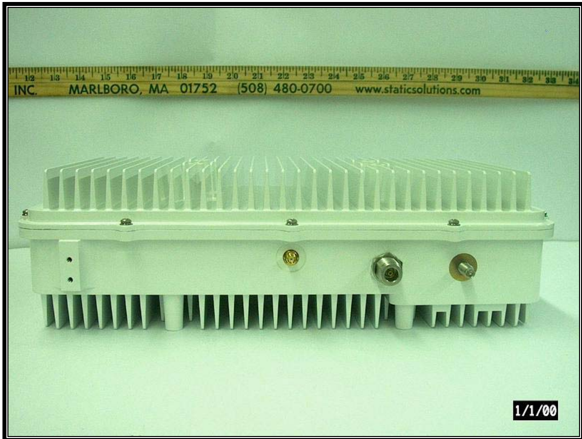
Photograph 6: Chassis Front
