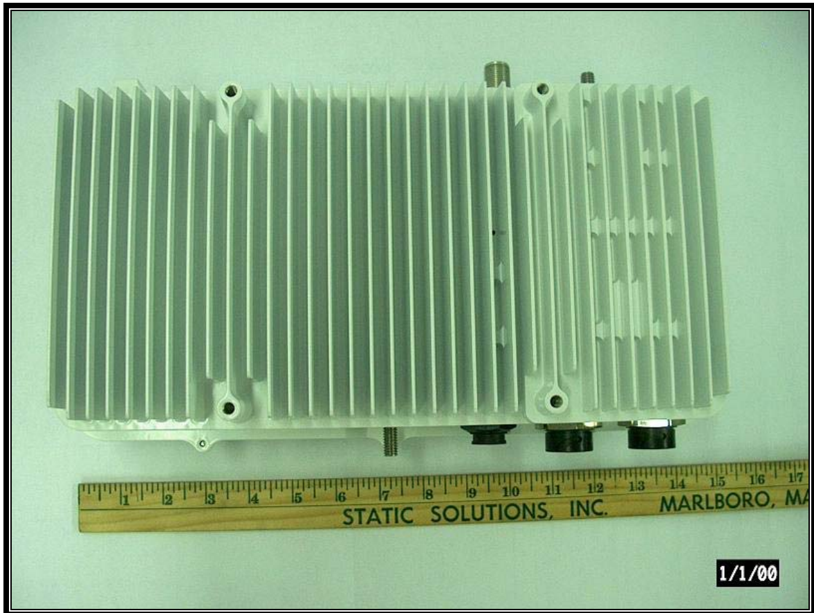
Photograph 5: Chassis Bottom
