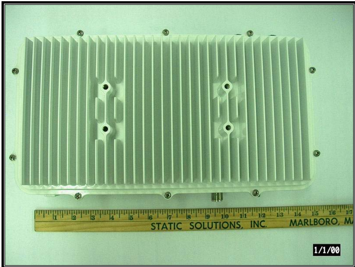
Photograph 4: Chassis Top
