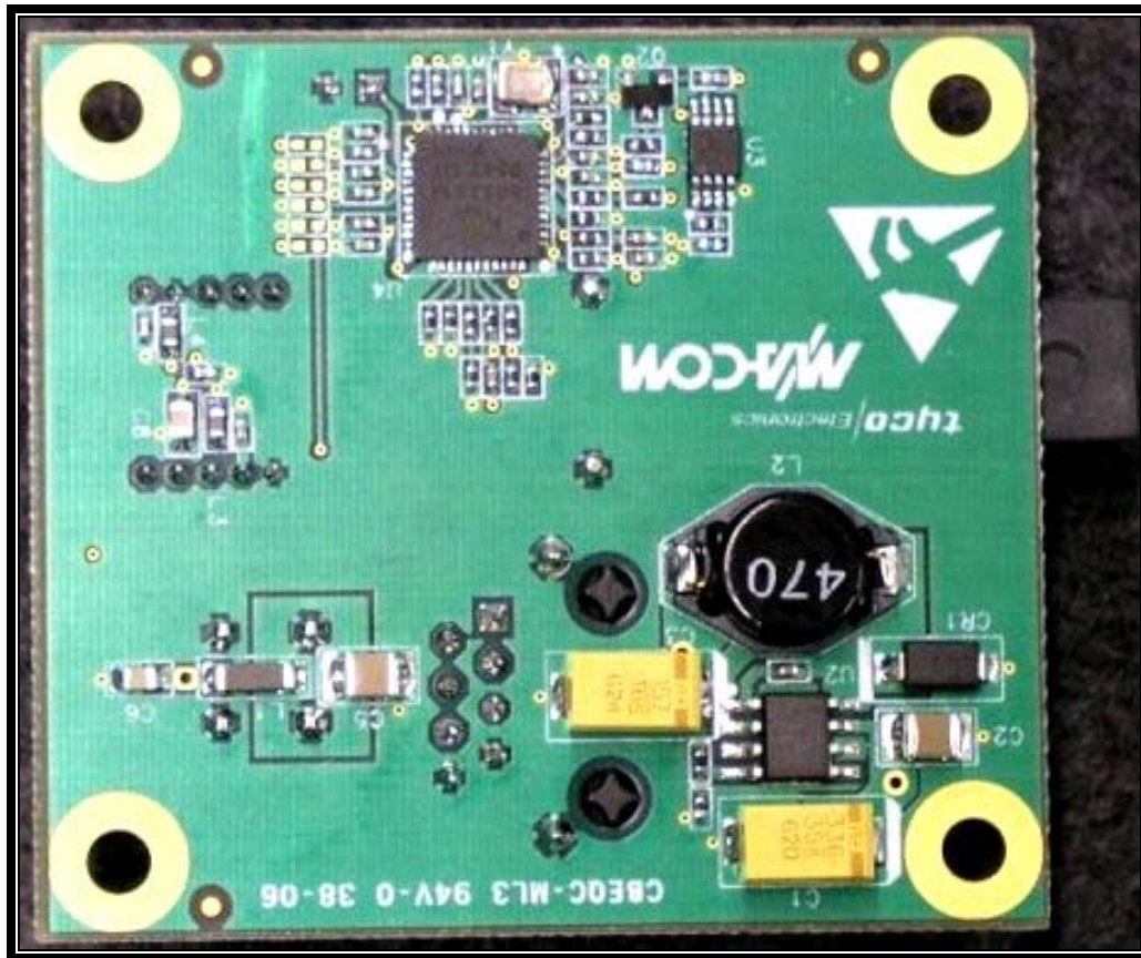
Photograph 15: PCB Fiber Bottom
