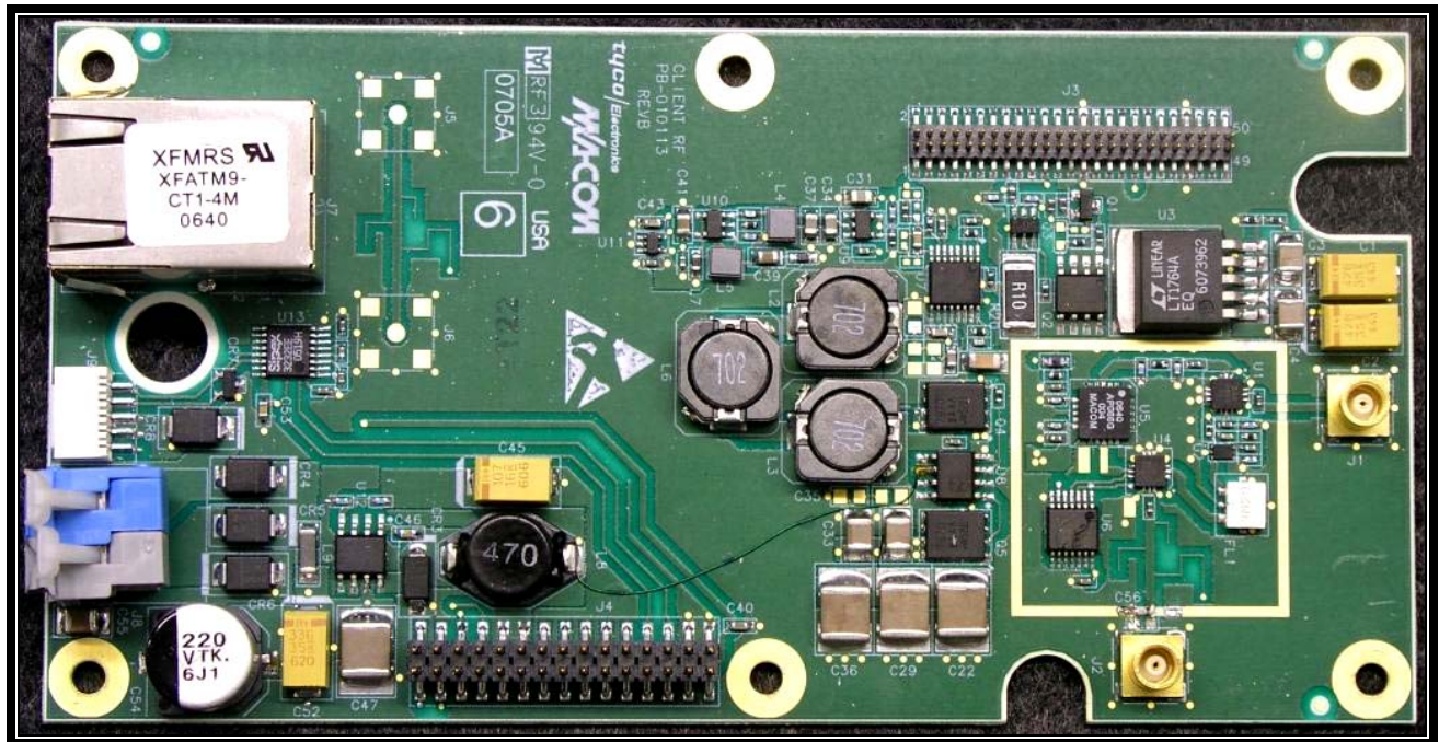
Photograph 16: PCB Front End Top
