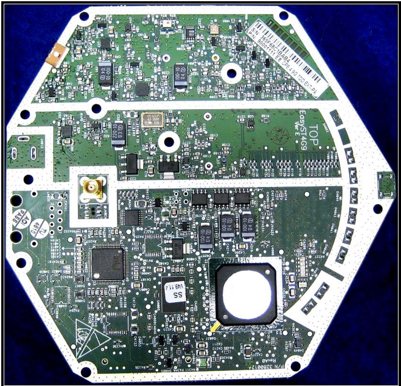
Photograph 18: PCB XCVR Top
