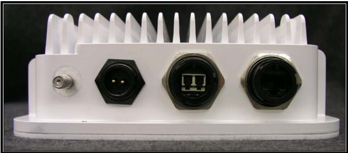
Photograph 10: Hardened Version – Connectors
