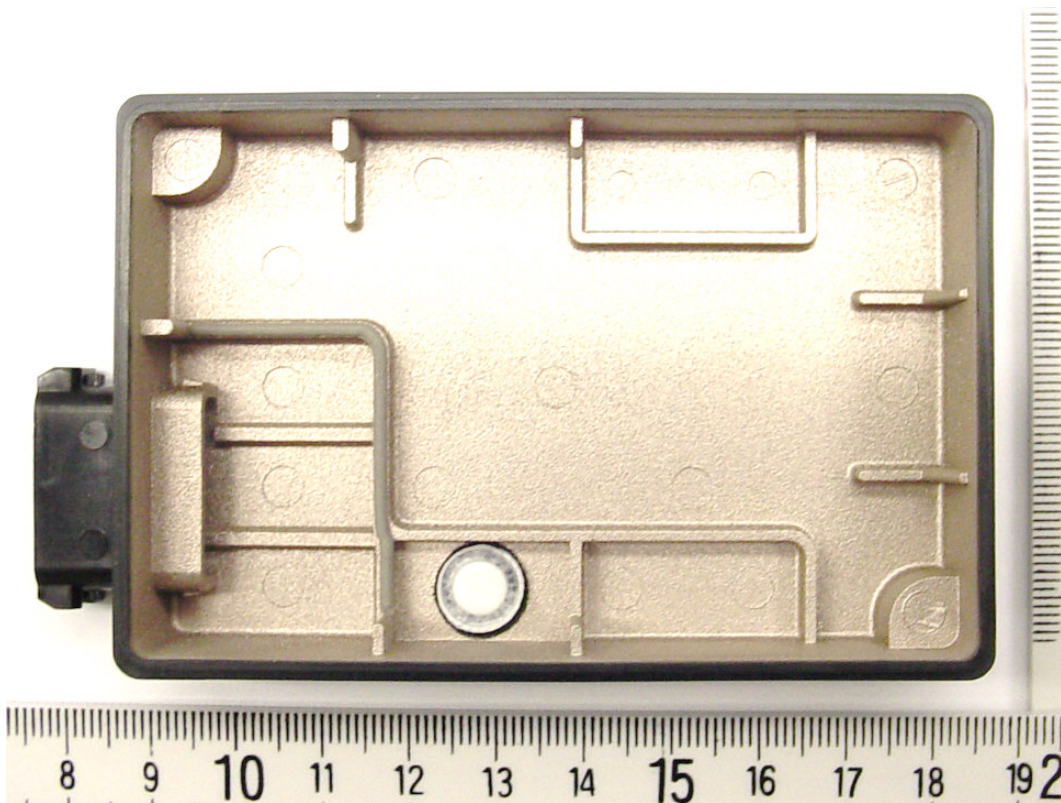
Photograph 7: Internal View of the EUT; Housing
