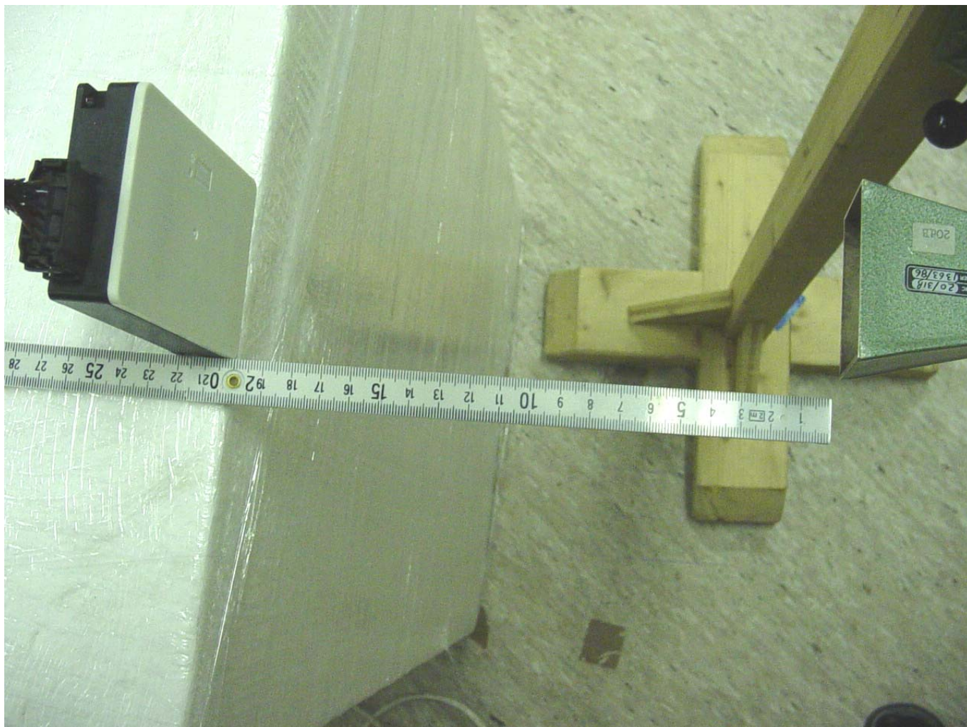
Photograph 5: RF Exposure Measurement at 20 cm Distance
