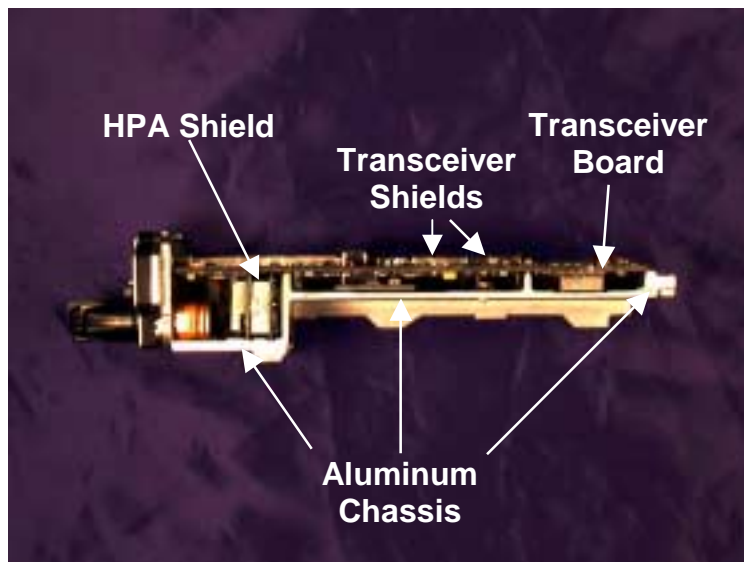
Figure A2-2 - BV8P-801T Cross-Section Photograph (Keypad and PK Board Removed)
