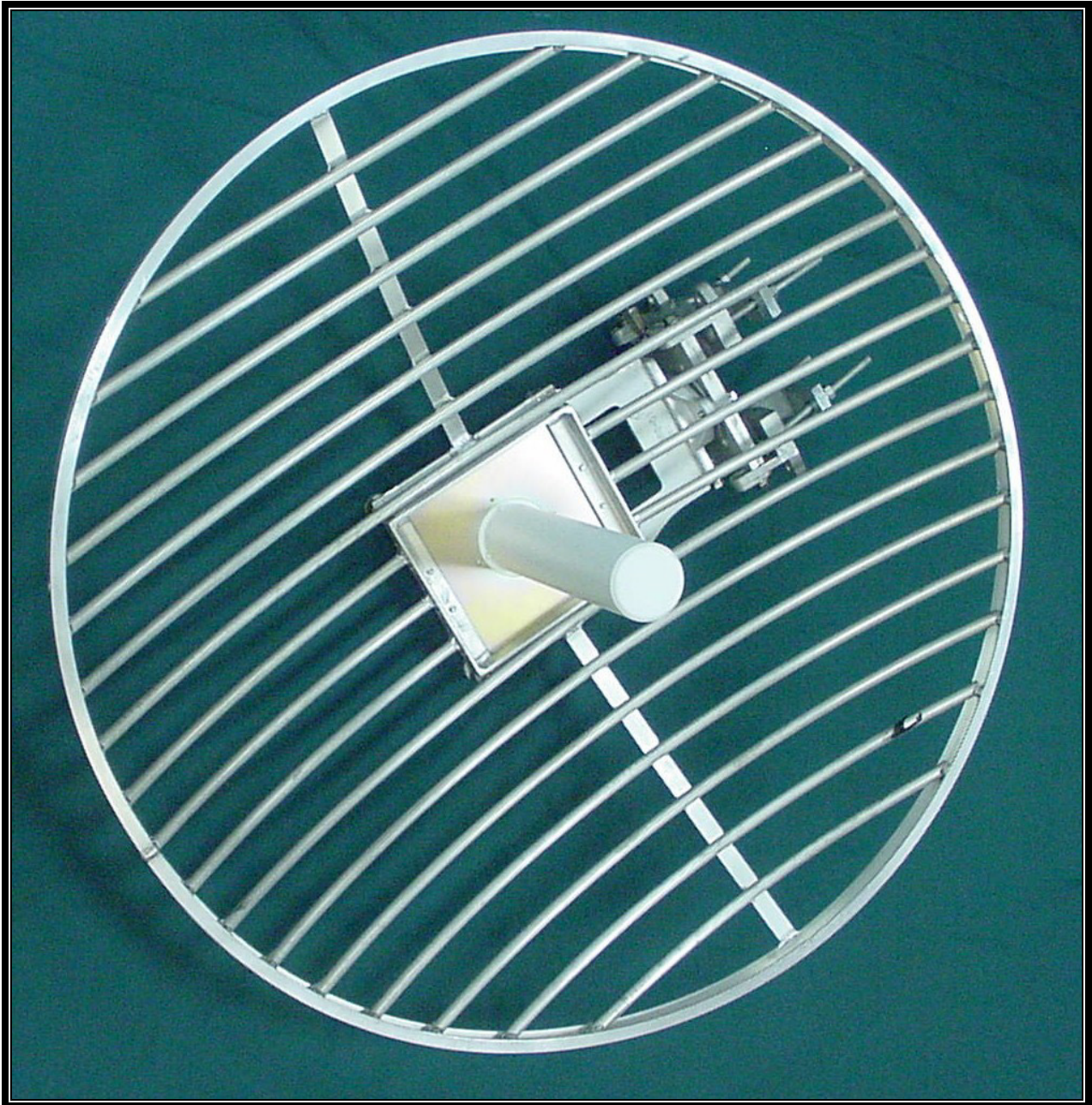
PHOTOGRAPH 12: GRID PARABOLIC ANTENNA FRONT VIEW
