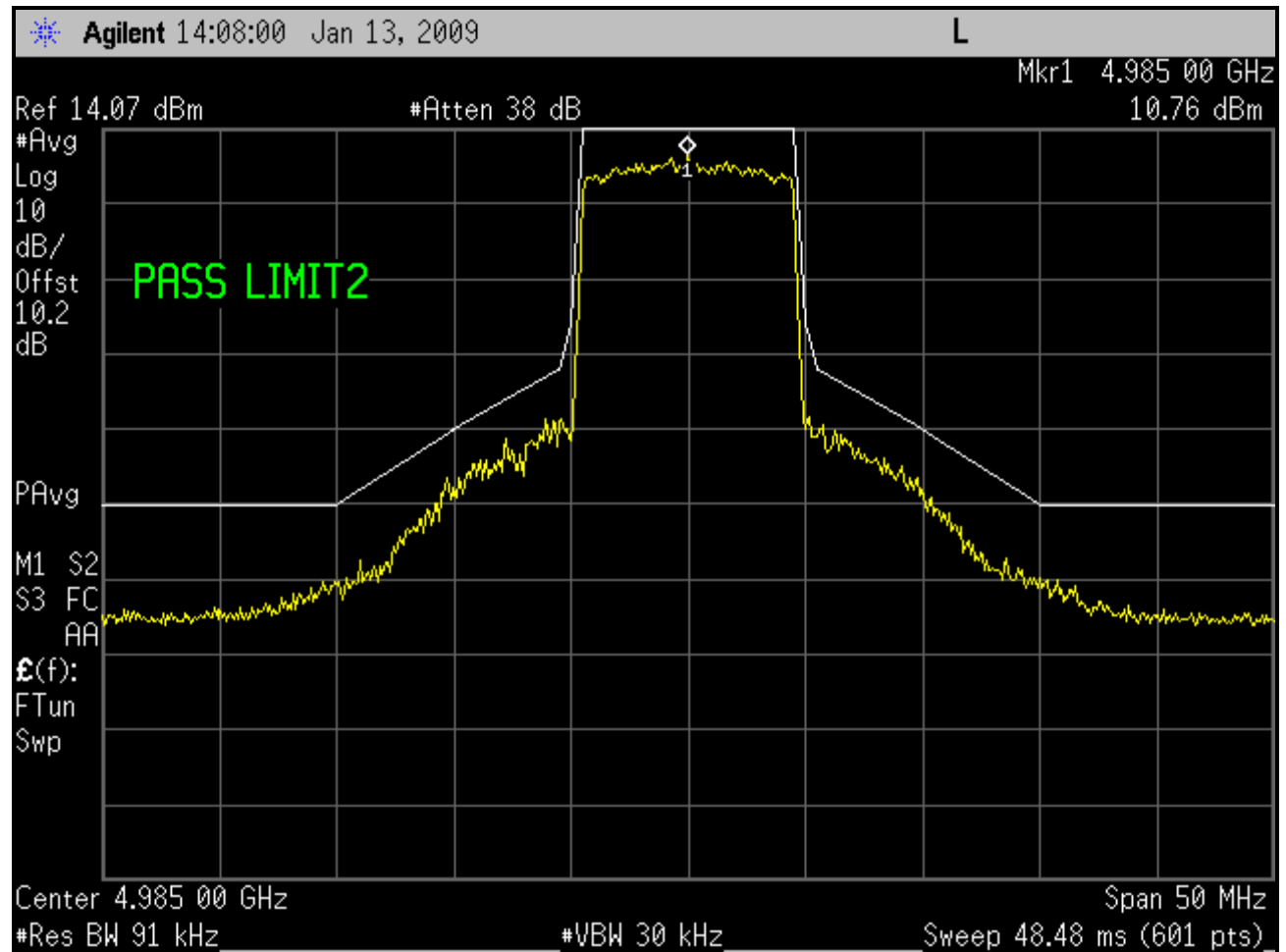
Plot 6-12: Emissions Mask M; Channel 5 - 4985 MHz (10 MHz BW; BS)
