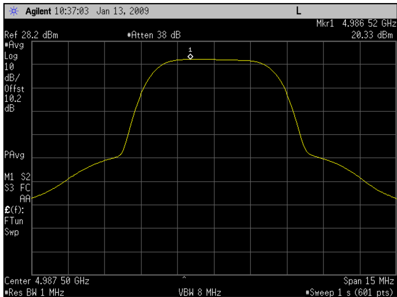
Plot 5-3: Peak Power Spectral Density; Channel 10 - 4987.5 MHz (BS)
