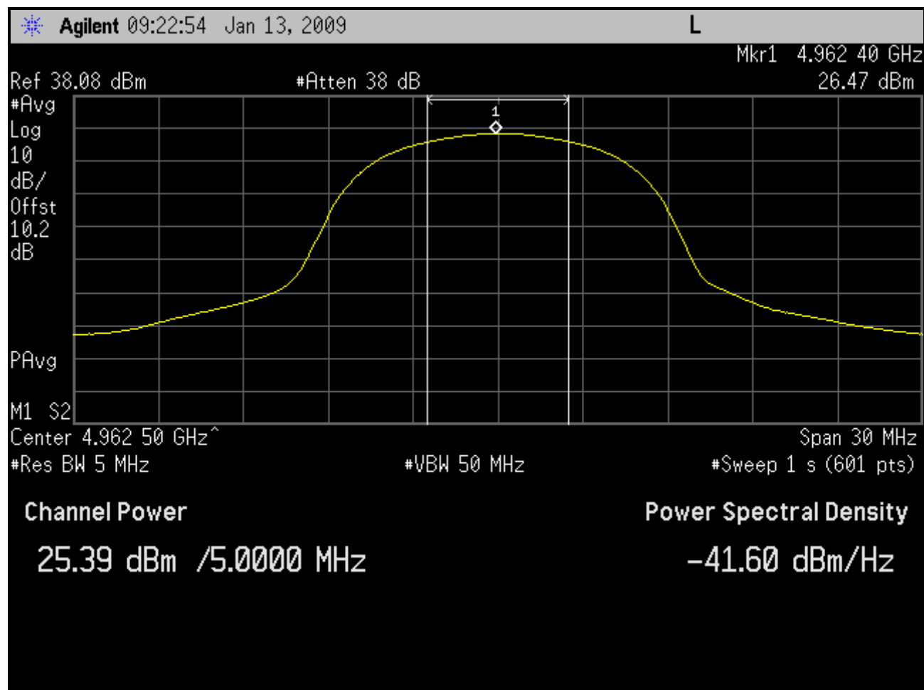
Plot 4-8: Channel Power Output; Channel 5 - 4962.5 MHz (SS)
