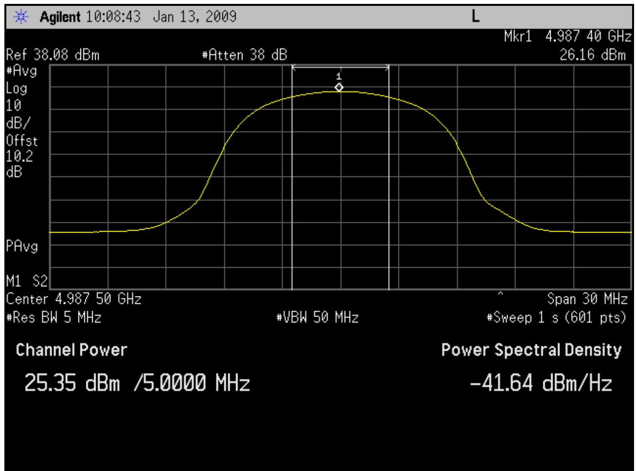
Plot 4-3: Channel Power Output; Channel 10 - 4987.5 MHz (BS)
