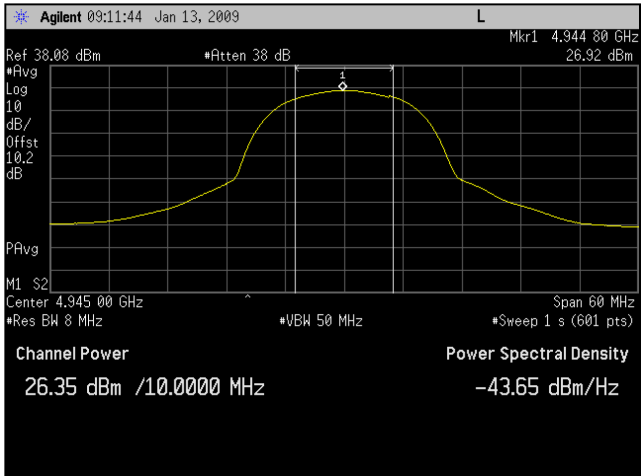
Plot 4-10: Channel Power Output; Channel 1 - 4945 MHz (SS)
