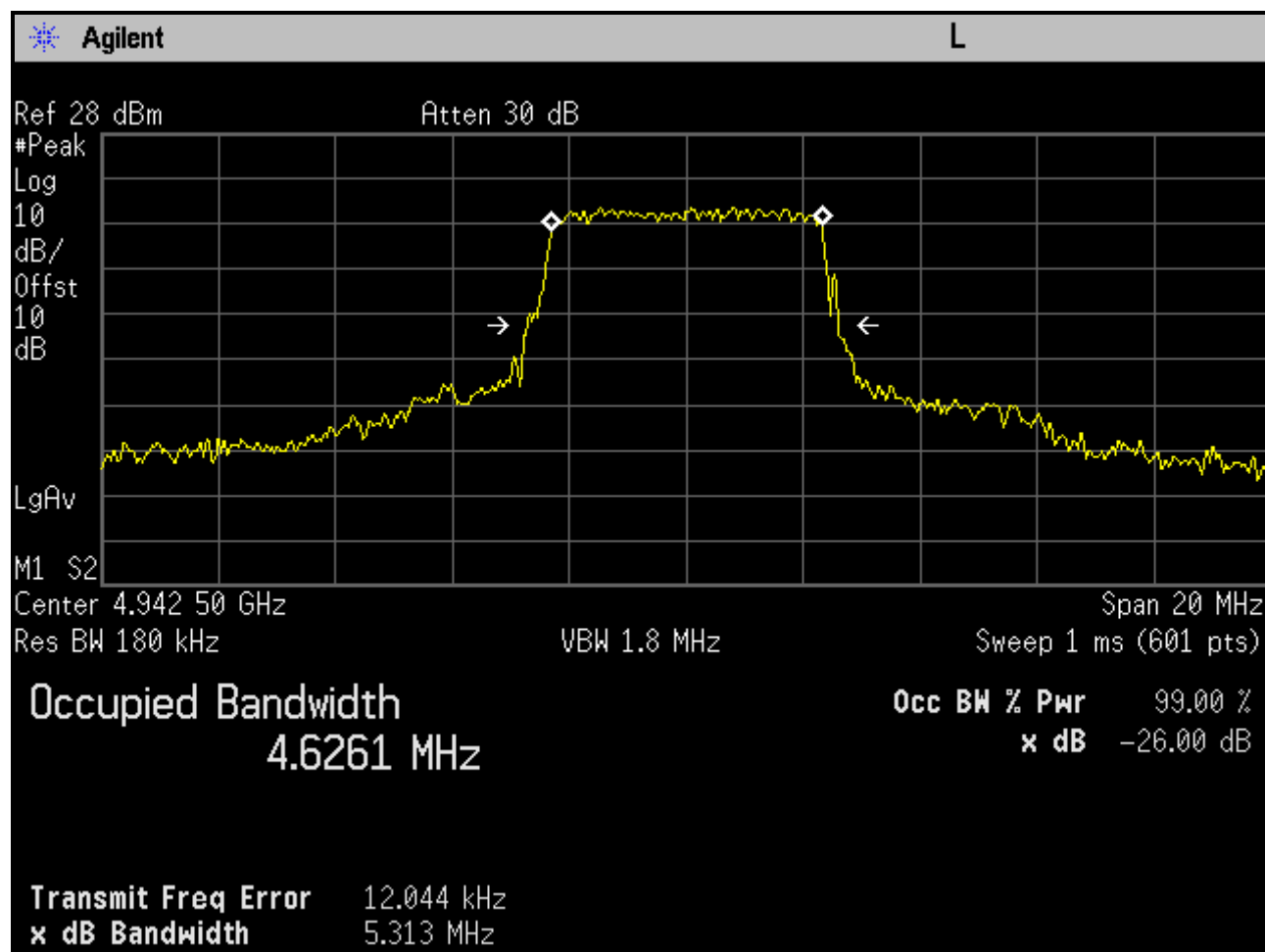
Plot 6-13: Occupied Bandwidth; Channel 1 - 4942.5 MHz (5 MHz BW; SS)
