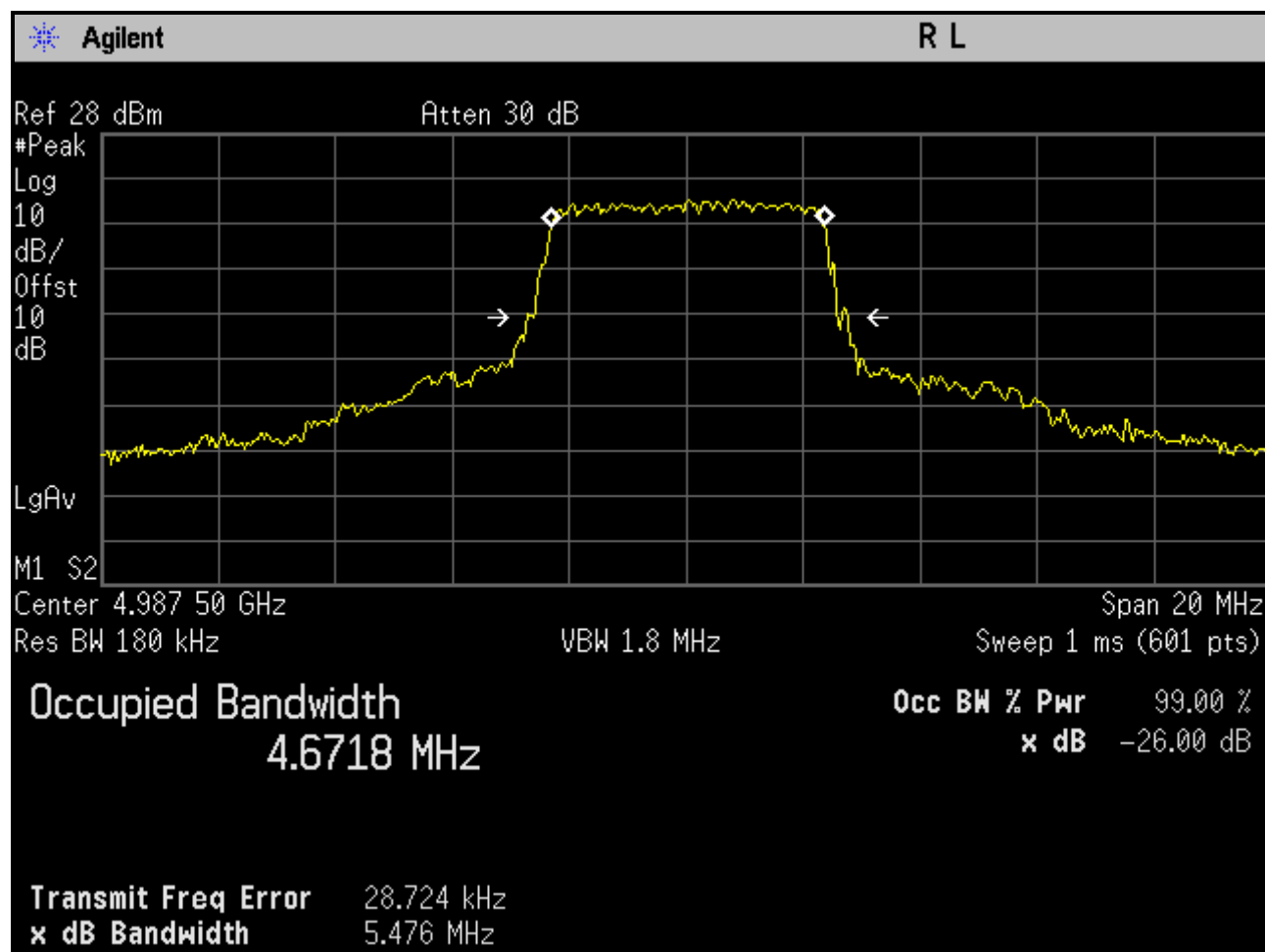
Plot 6-17: Occupied Bandwidth; Channel 10 - 4987.5 MHz (5 MHz BW; SS)
