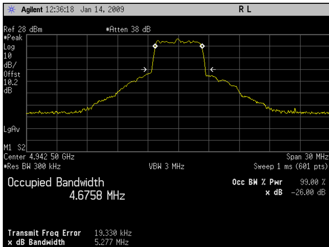
Plot 6-1: Occupied Bandwidth; Channel 1 - 4942.5 MHz (5 MHz BW; BS)
