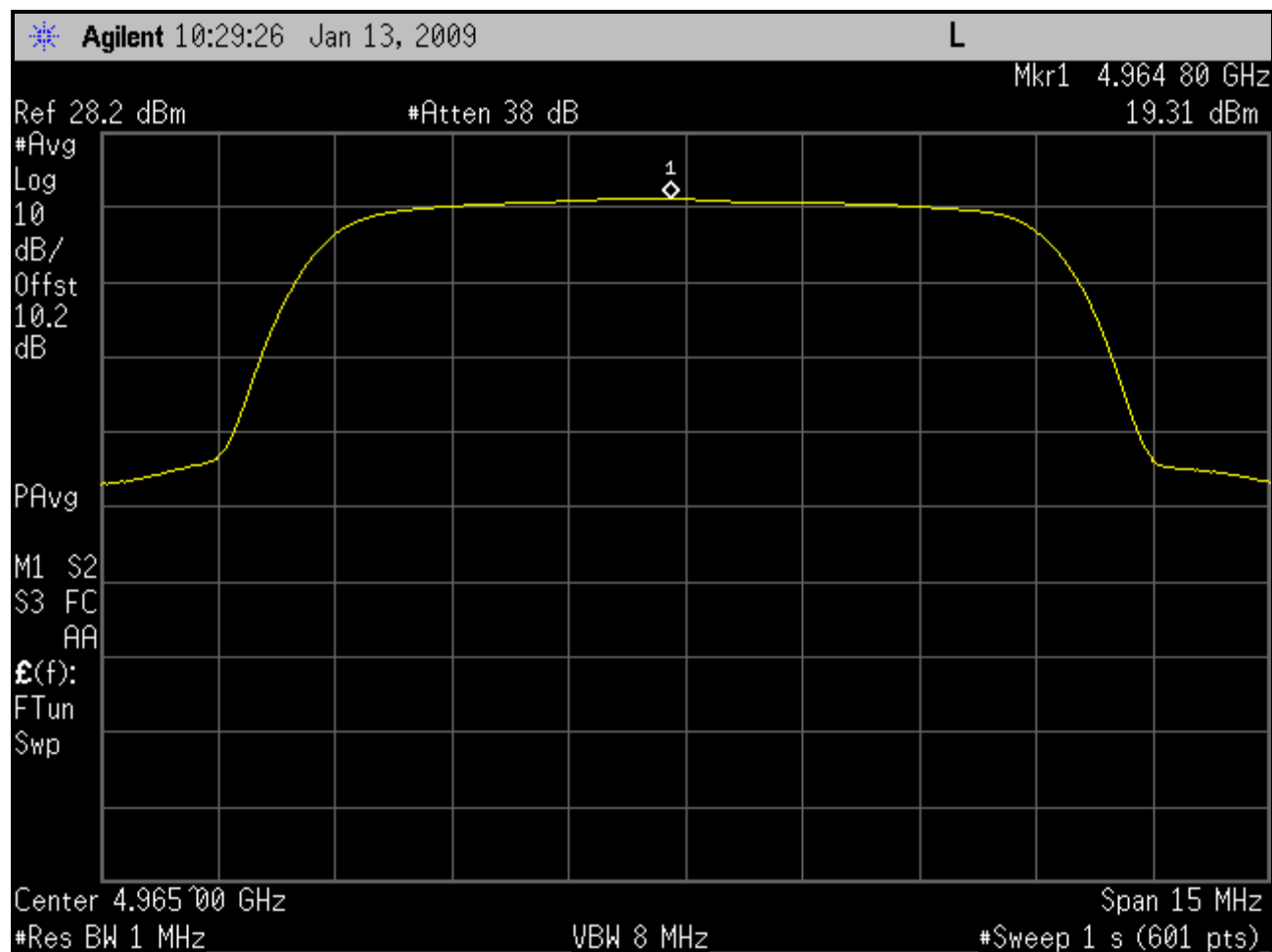
Plot 5-5: Peak Power Spectral Density; Channel 3 - 4965 MHz (BS)
