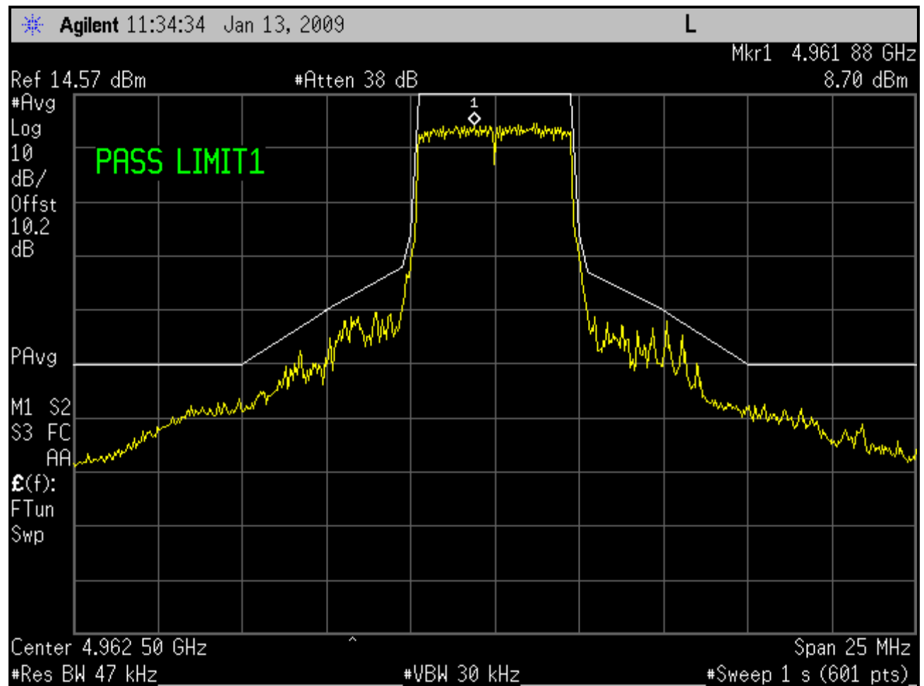
Plot 6-16: Emissions Mask M; Channel 5 - 4962.5 MHz (5 MHz BW; SS)
