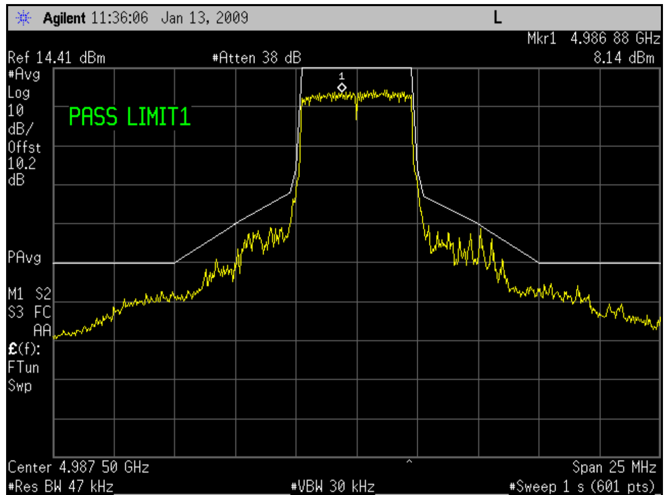
Plot 6-18: Emissions Mask M; Channel 10 - 4987.5 MHz (5 MHz BW; SS)
