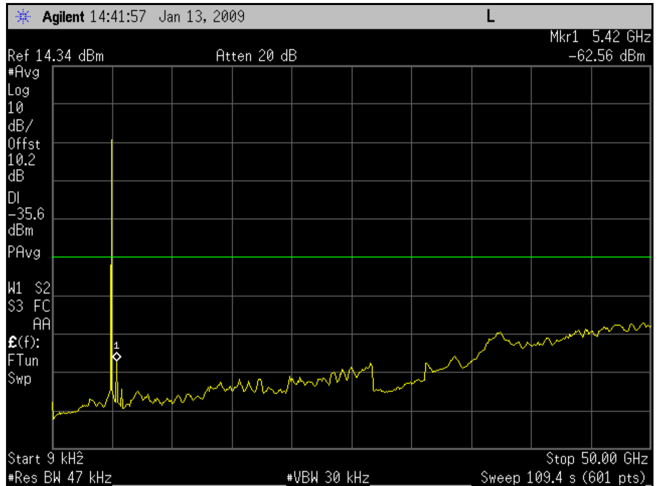
Plot 6-29: Conducted Spurious Emissions; Channel 3 – 4965 MHz (10 MHz BW; Full Band; BS)
