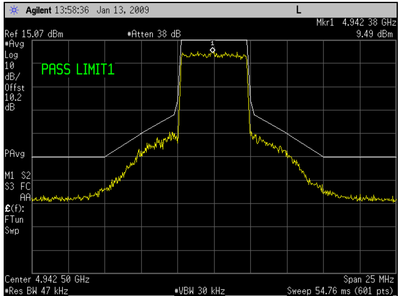
Plot 6-2: Emissions Mask M; Channel 1- 4942.5 MHz (5 MHz BW; BS)
