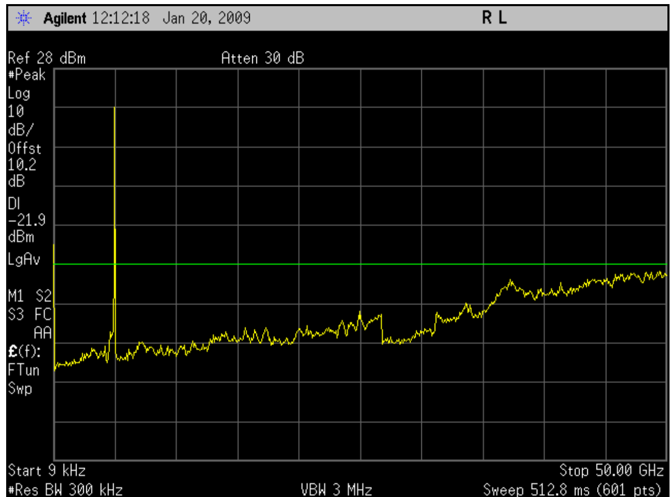
Plot 6-35: Conducted Spurious Emissions; Channel 3 – 4965 MHz (10 MHz BW; Full Band; SS)
