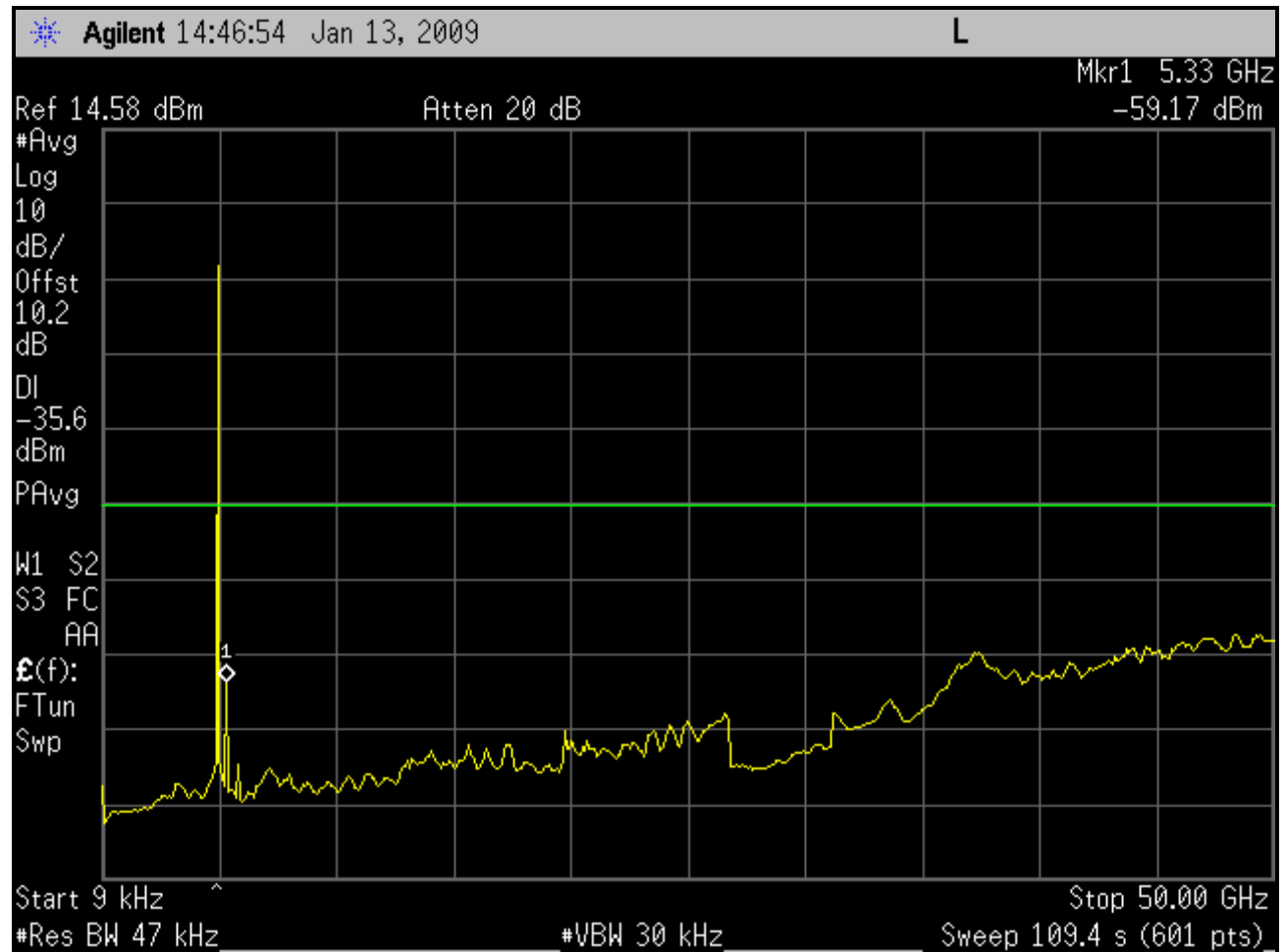
Plot 6-28: Conducted Spurious Emissions; Channel 1 – 4945 MHz (10 MHz BW; Full Band; BS)
