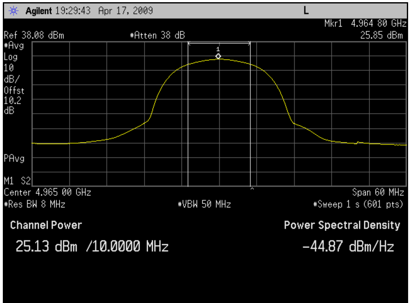
Plot 4-11: Channel Power Output; Channel 3 - 4965 MHz (SS)
