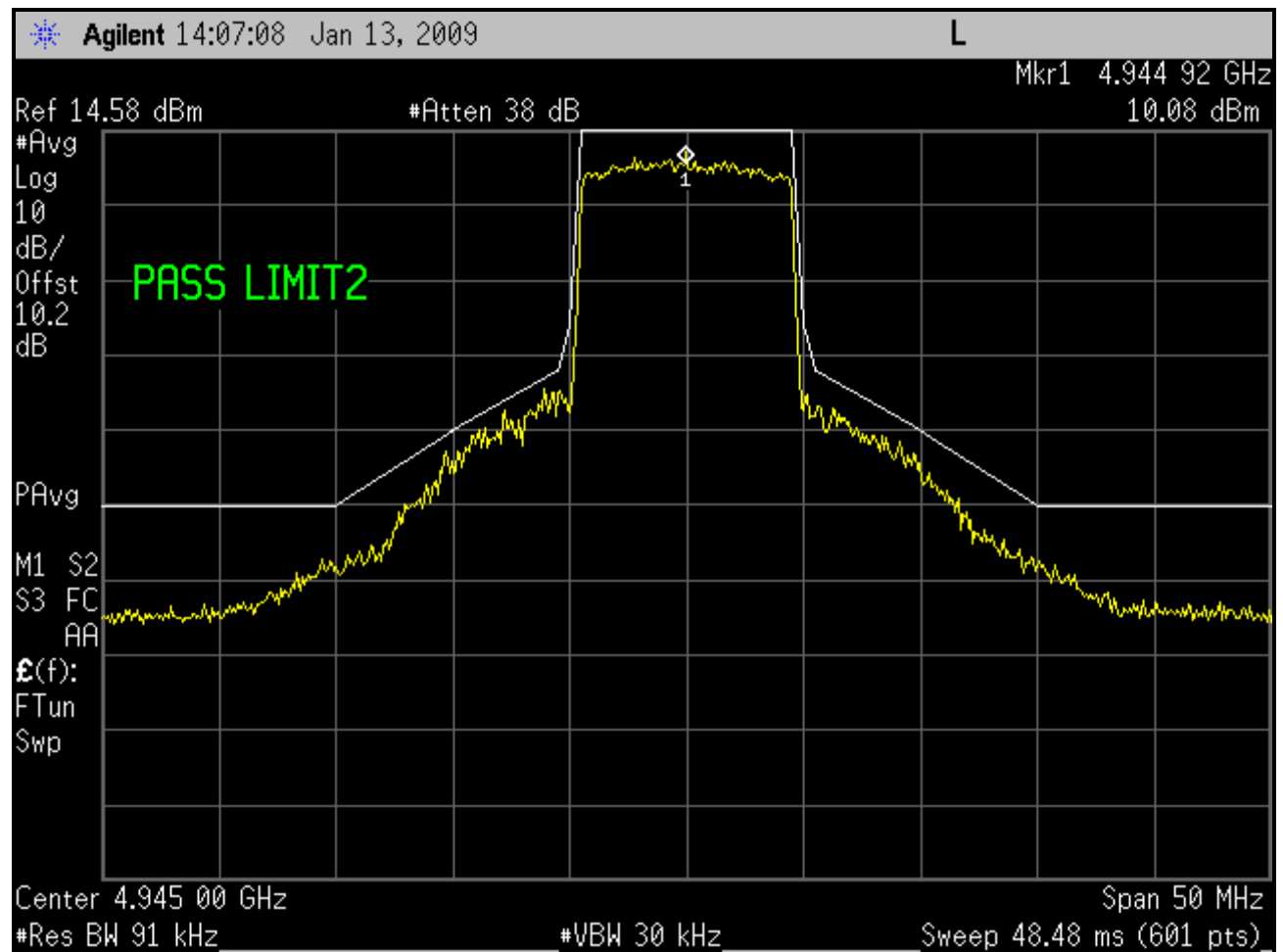
Plot 6-8: Emissions Mask M; Channel 1 - 4945 MHz (10 MHz BW; BS)
