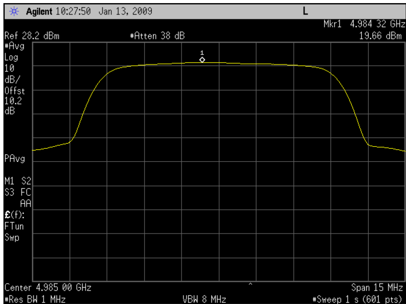
Plot 5-6: Peak Power Spectral Density; Channel 5 - 4985 MHz (BS)
