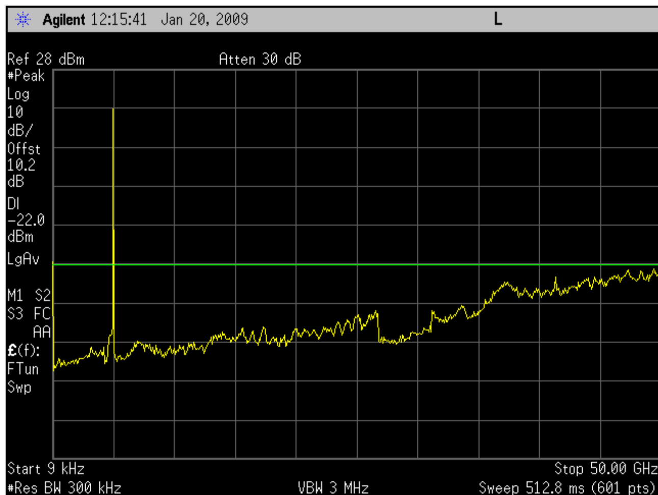
Plot 6-32: Conducted Spurious Emissions; Channel 5 – 4962.5 MHz (5 MHz BW; Full Band; SS)
