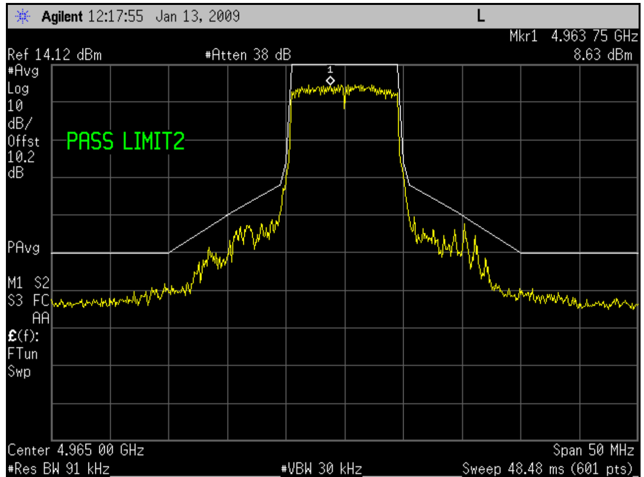
Plot 6-22: Emissions Mask M; Channel 3 - 4965 MHz (10 MHz BW; SS)
