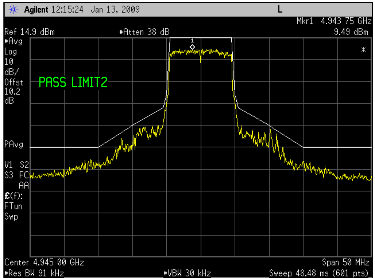
Plot 6-20: Emissions Mask M; Channel 1 - 4945 MHz (10 MHz BW; SS)
