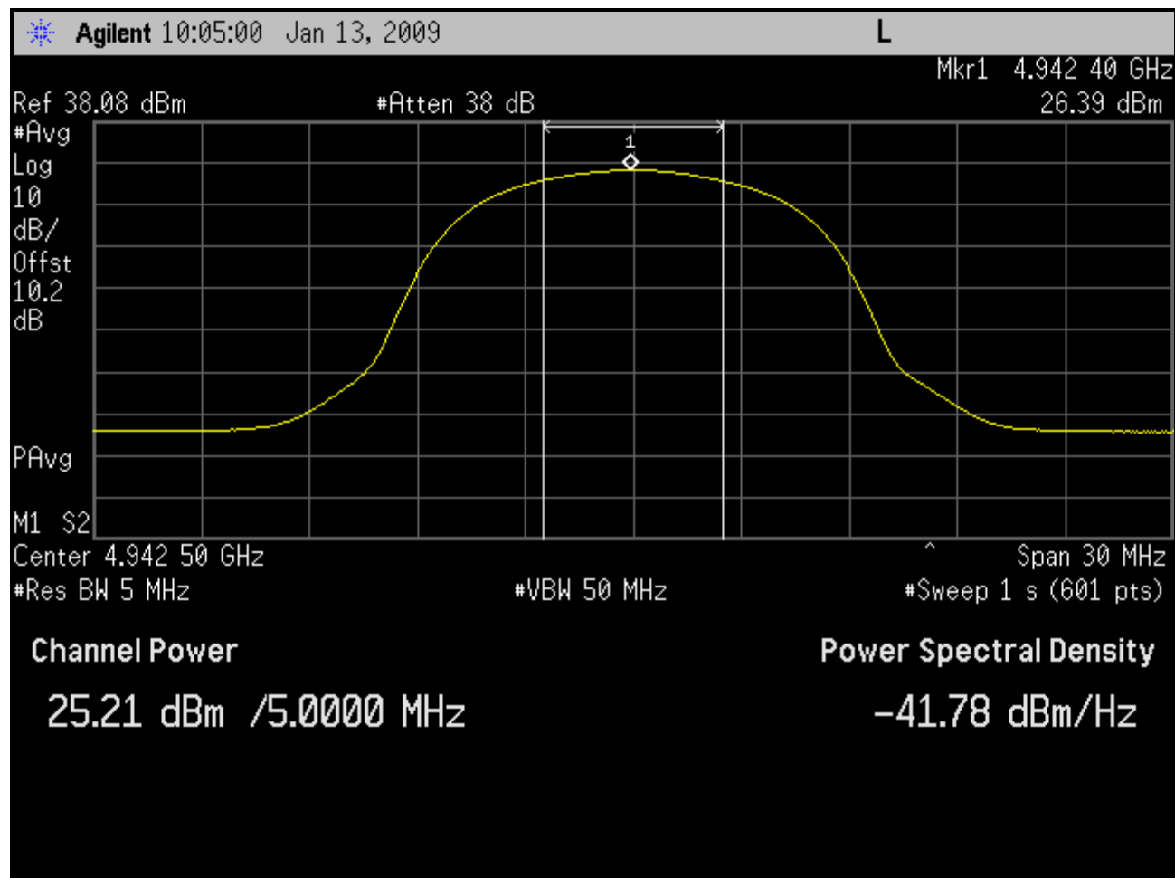
Plot 4-1: Channel Power Output; Channel 1 - 4942.5 MHz (BS)
