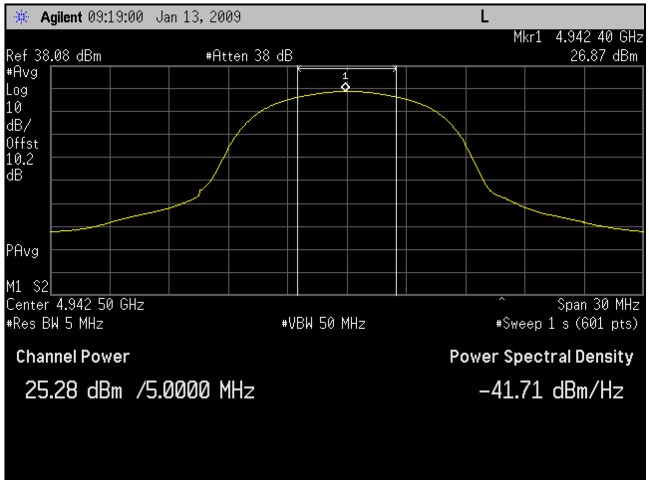
Plot 4-7: Channel Power Output; Channel 1 - 4942.5 MHz (SS)
