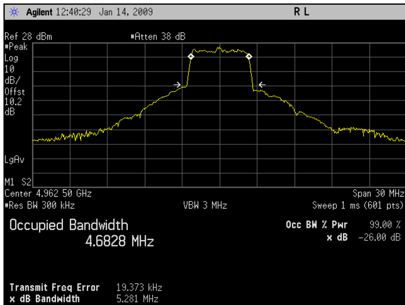
Plot 6-3: Occupied Bandwidth; Channel 5 - 4962.5 MHz (5 MHz BW; BS)
