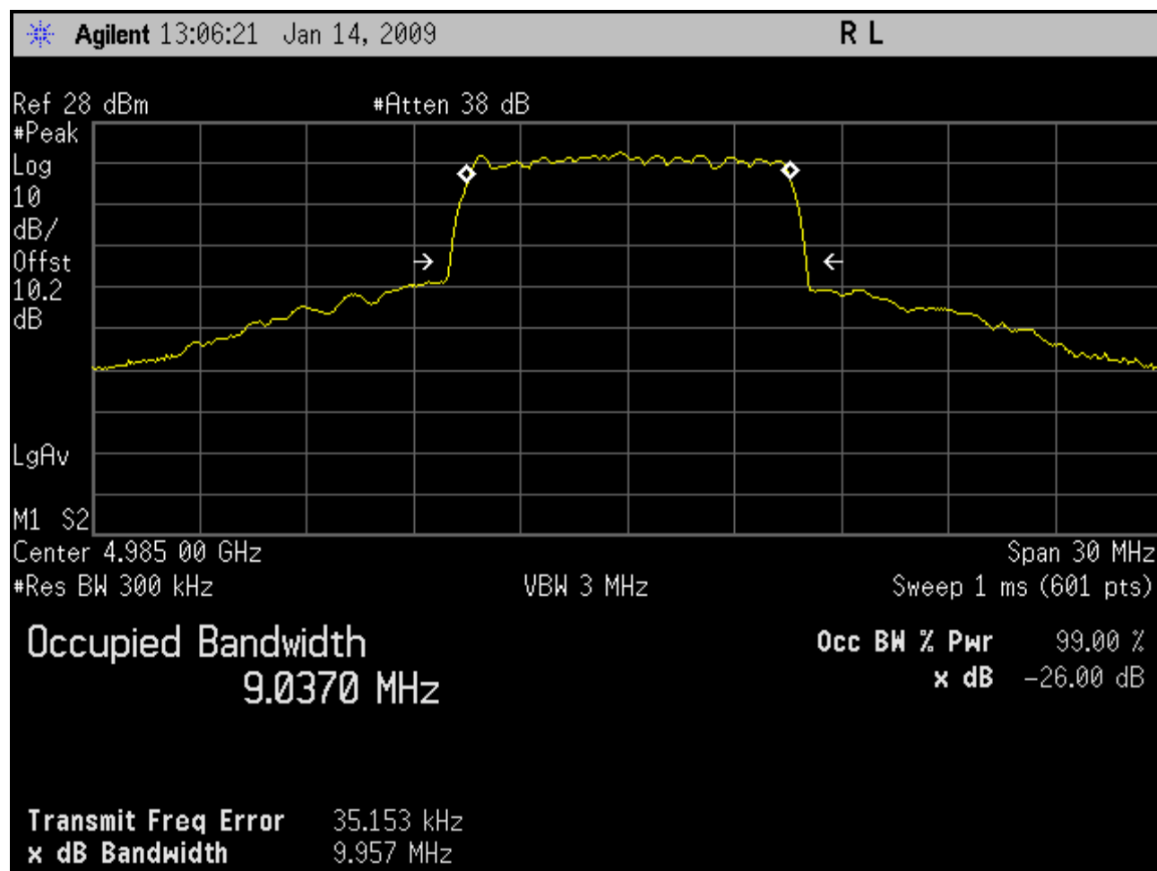
Plot 6-11: Occupied Bandwidth; Channel 5 - 4985 MHz (10 MHz BW; BS)
