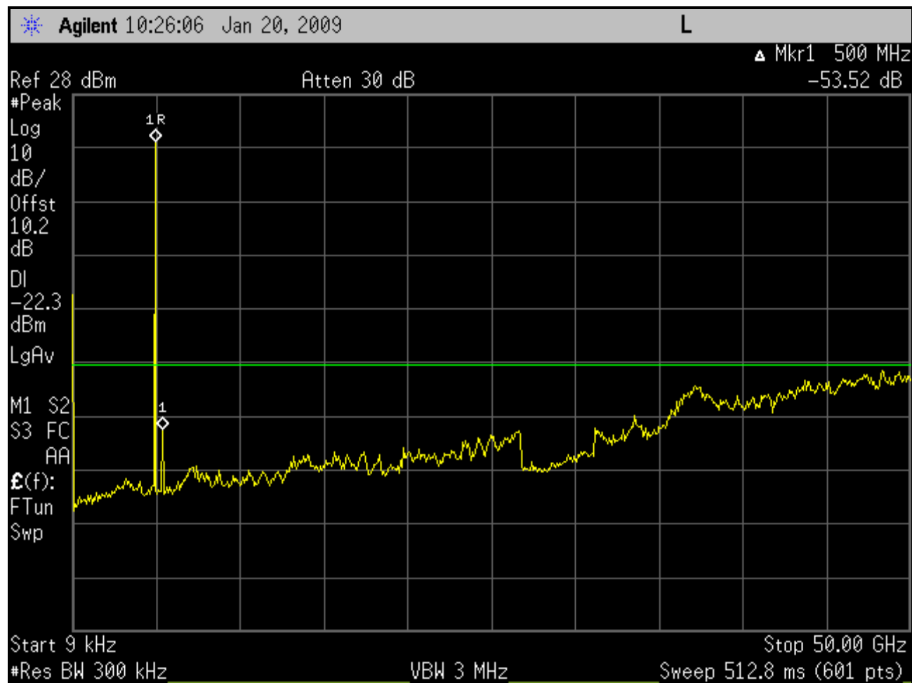
Plot 6-25: Conducted Spurious Emissions; Channel 1 – 4942.5 MHz (5 MHz BW; Full Band; BS)
