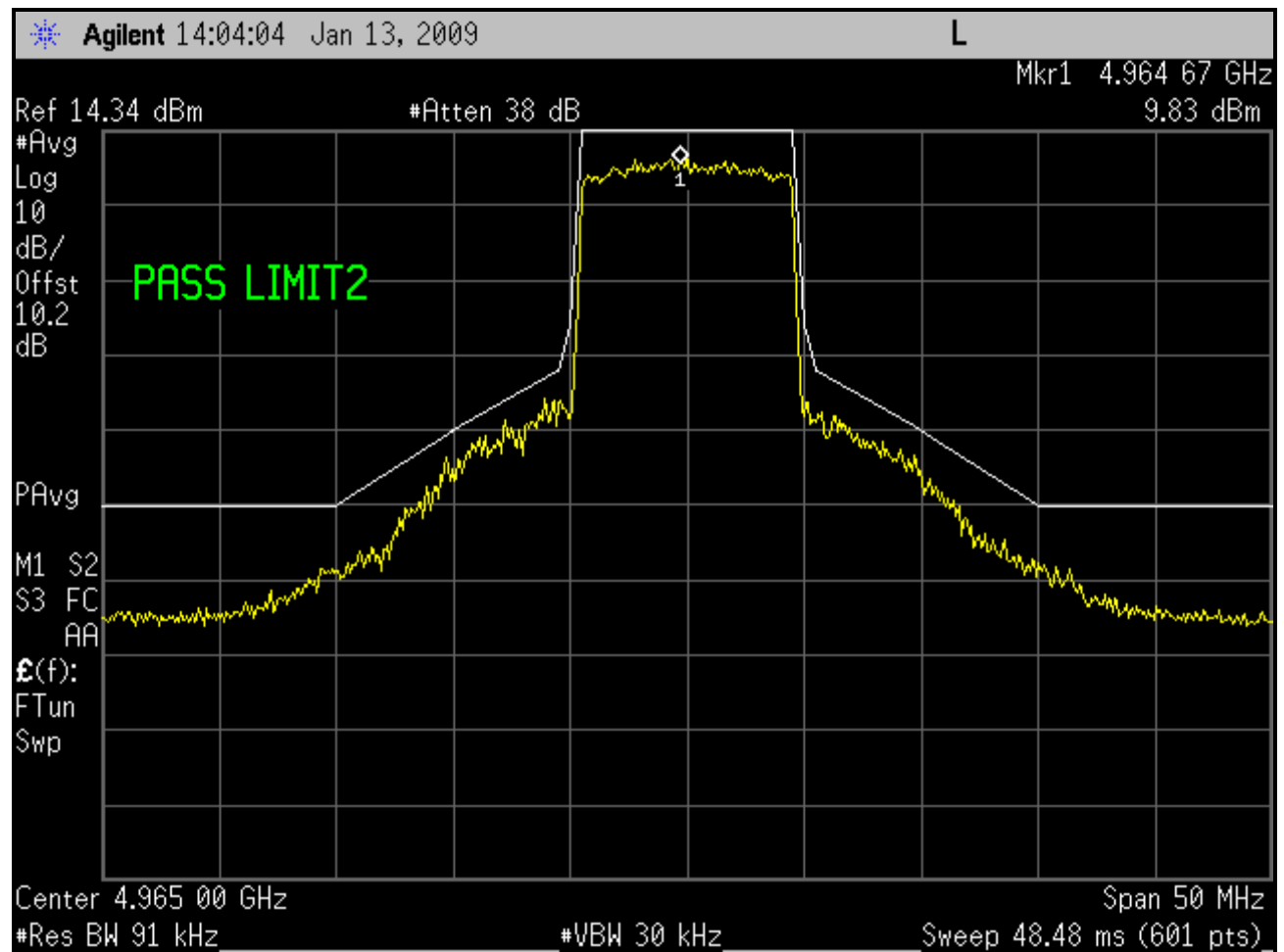
Plot 6-10: Emissions Mask M; Channel 3 - 4965 MHz (10 MHz BW; BS)
