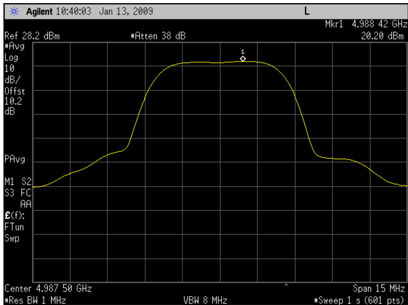
Plot 5-9: Peak Power Spectral Density; Channel 10 - 4987.5 MHz (SS)
