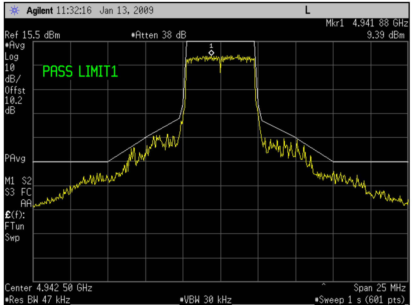
Plot 6-14: Emissions Mask M; Channel 1- 4942.5 MHz (5 MHz BW; SS)
