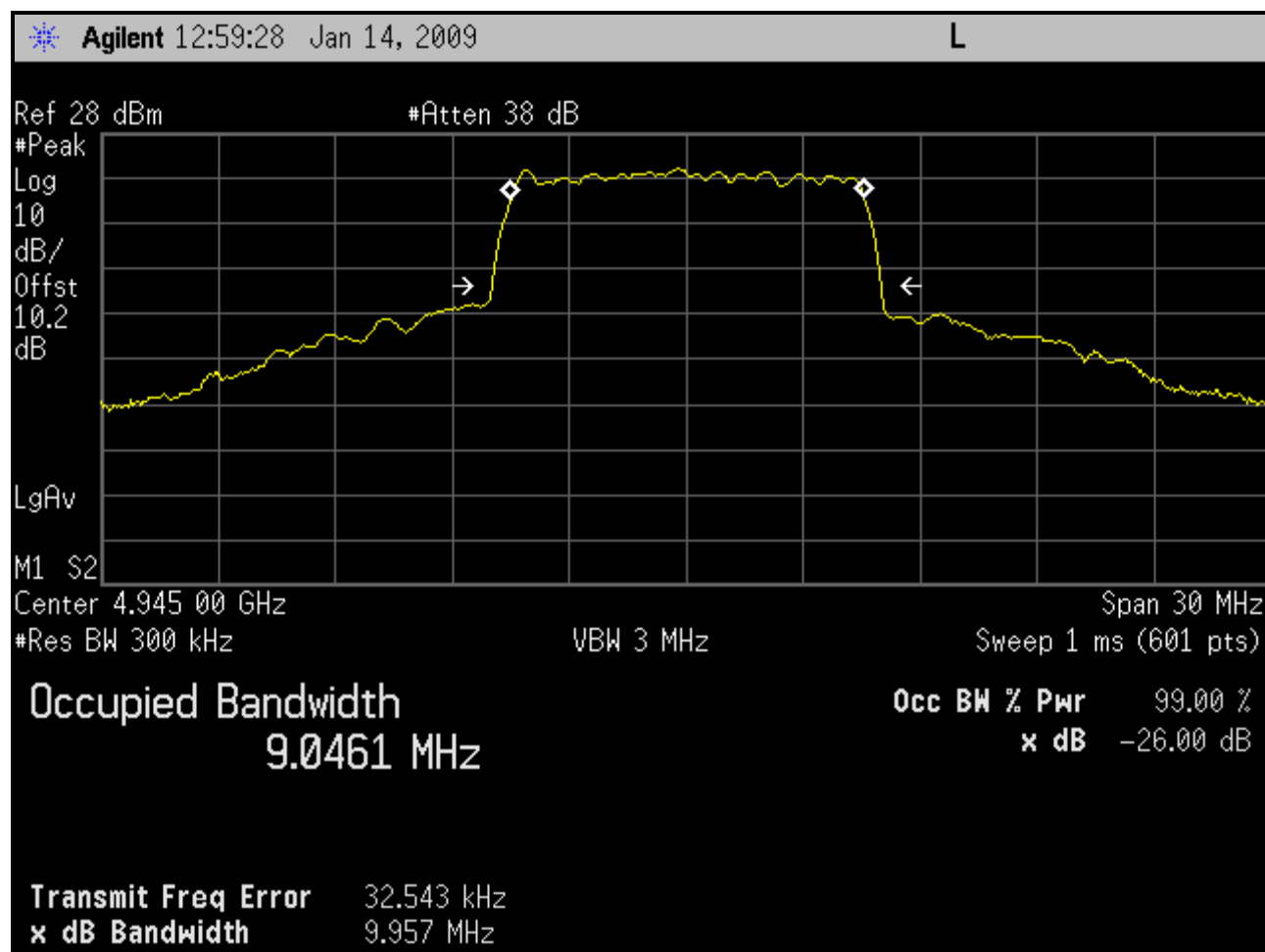
Plot 6-7: Occupied Bandwidth; Channel 1 - 4945 MHz (10 MHz BW; BS)
