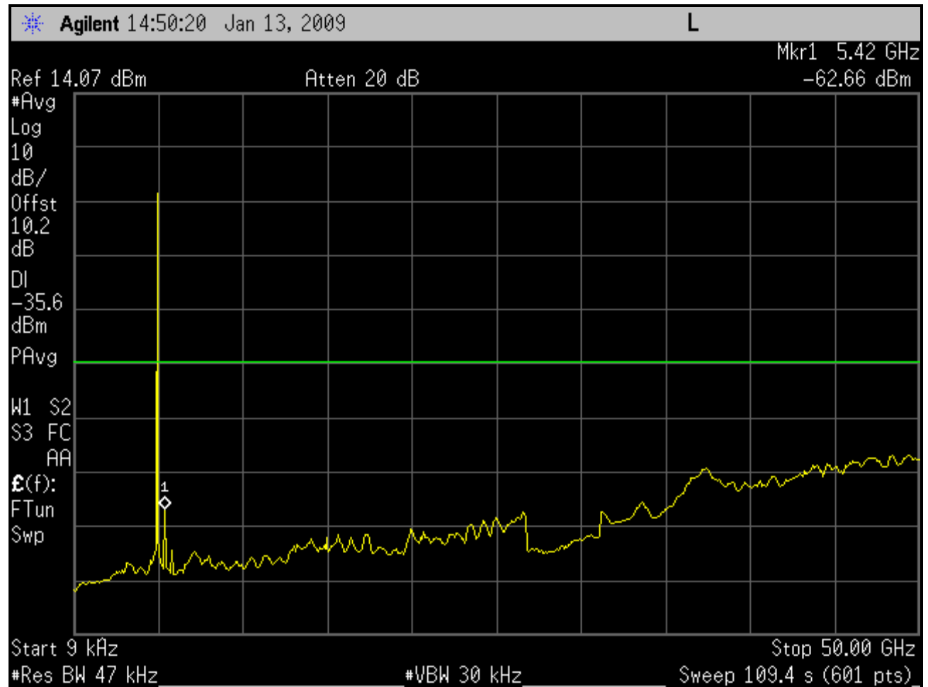
Plot 6-30: Conducted Spurious Emissions; Channel 5 – 4985 MHz (10 MHz BW; Full Band; BS)
