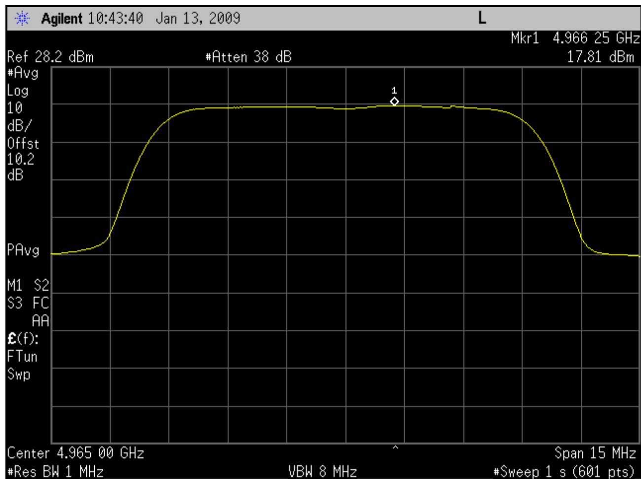
Plot 5-11: Peak Power Spectral Density; Channel 3 - 4965 MHz (SS)
