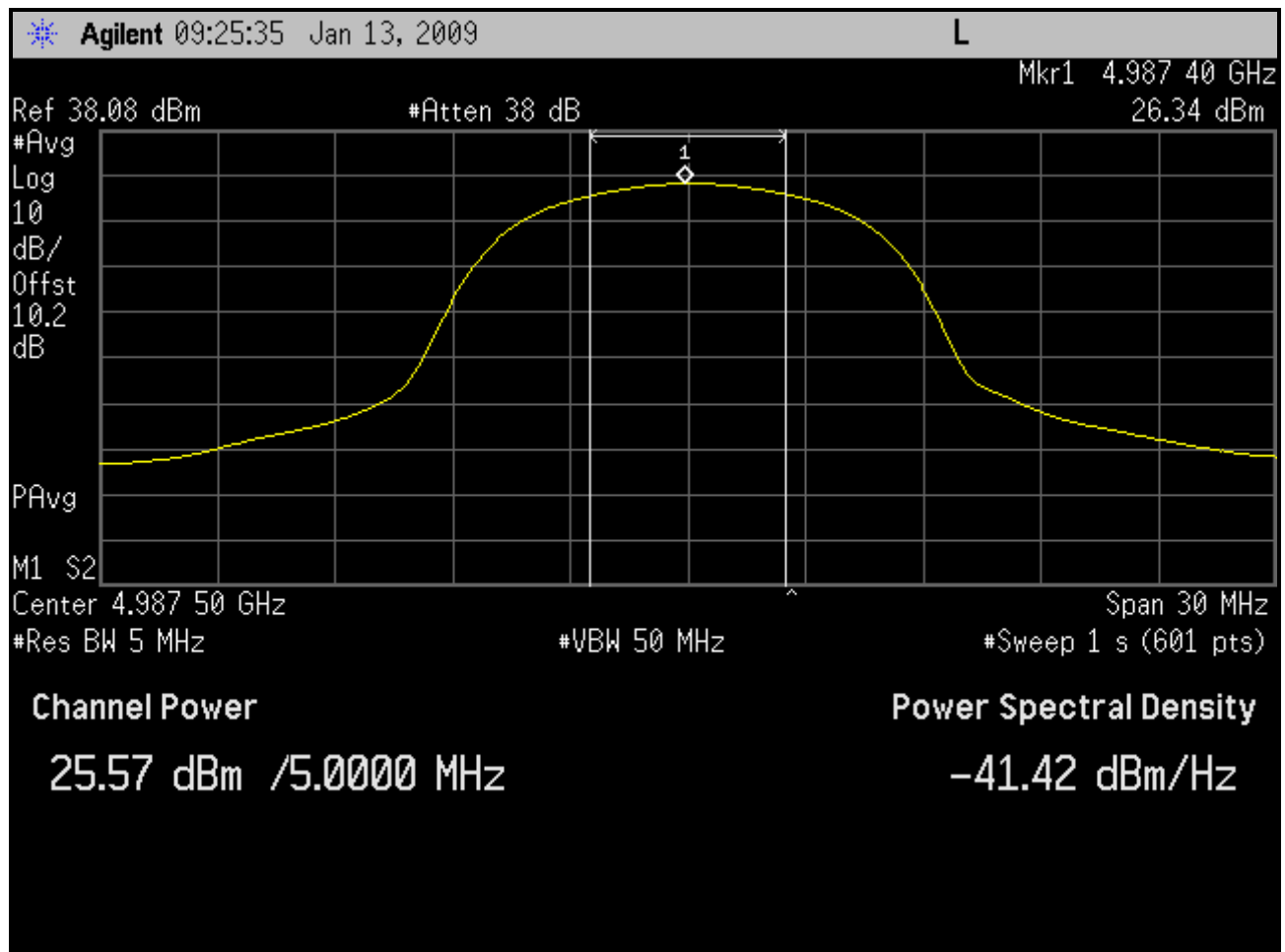
Plot 4-9: Channel Power Output; Channel 10 - 4987.5 MHz (SS)
