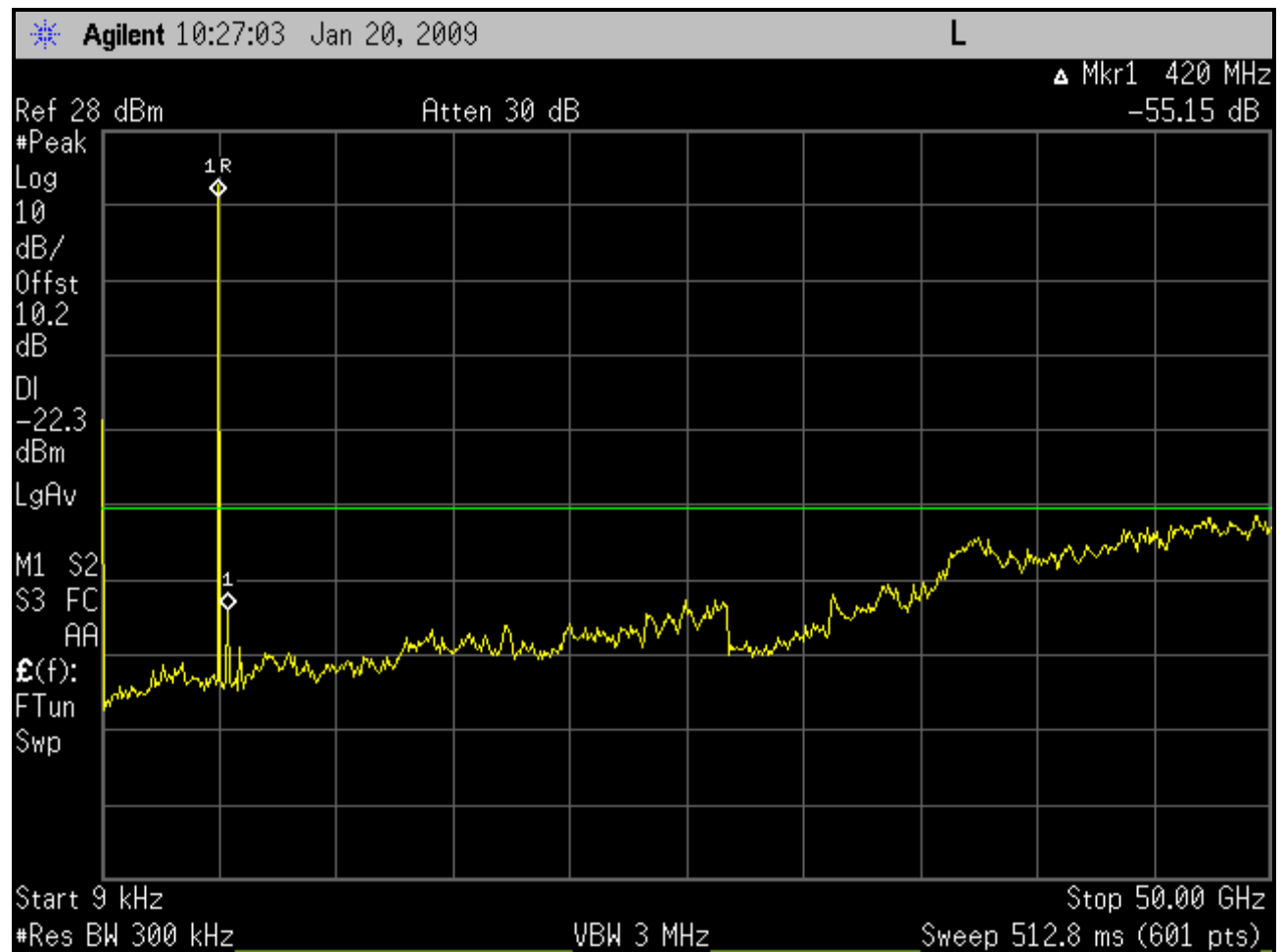
Plot 6-27: Conducted Spurious Emissions; Channel 10 – 4987.5 MHz (5 MHz BW; Full Band; BS)
