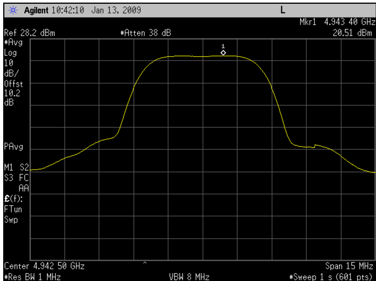
Plot 5-7: Peak Power Spectral Density; Channel 1 - 4942.5 MHz (SS)
