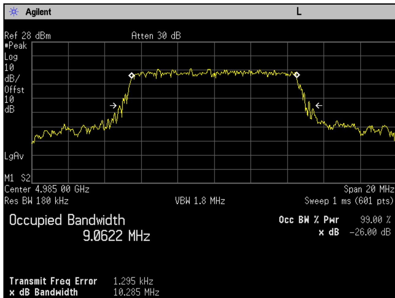
Plot 6-23: Occupied Bandwidth; Channel 5 - 4985 MHz (10 MHz BW; SS)
