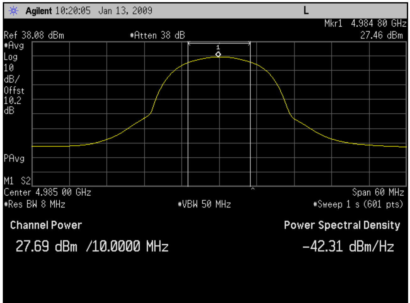
Plot 4-6: Channel Power Output; Channel 5 - 4985 MHz (BS)
