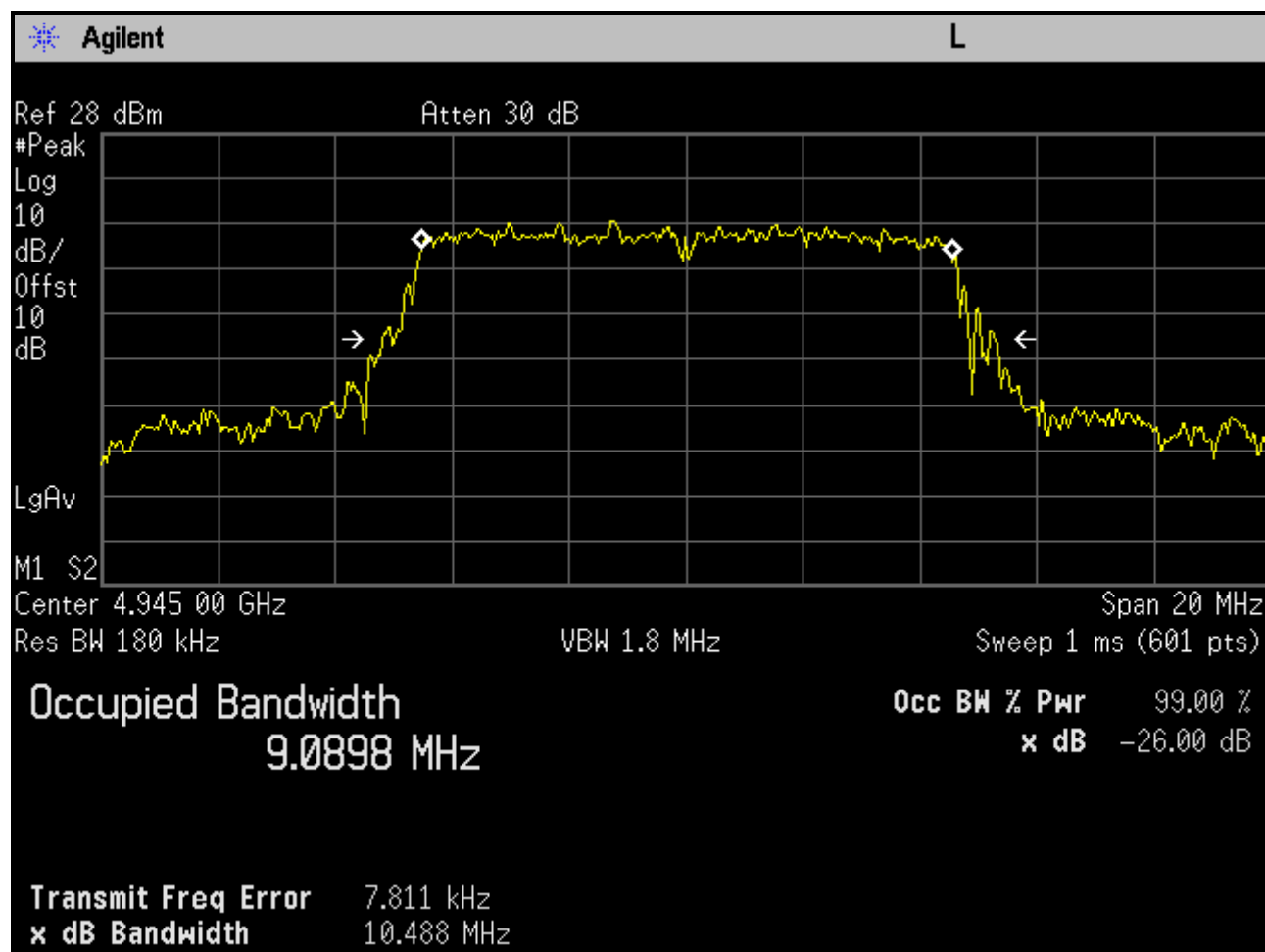
Plot 6-19: Occupied Bandwidth; Channel 1 - 4945 MHz (10 MHz BW; SS)
