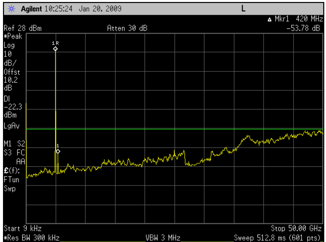
Plot 6-26: Conducted Spurious Emissions; Channel 5 – 4962.5 MHz (5 MHz BW; Full Band; BS)
