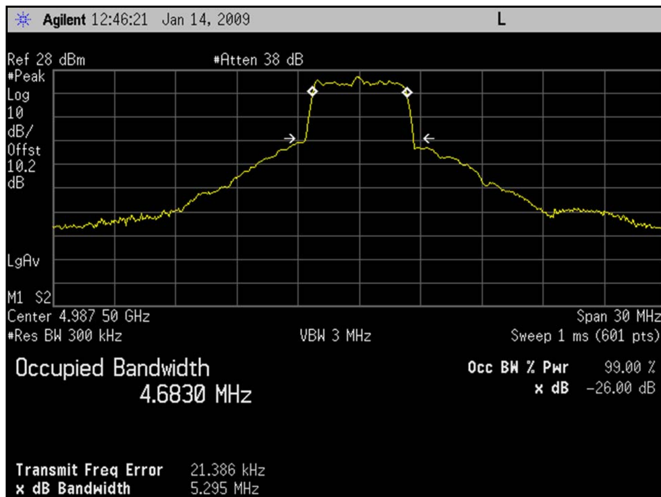
Plot 6-5: Occupied Bandwidth; Channel 10 - 4987.5 MHz (5 MHz BW; BS)
