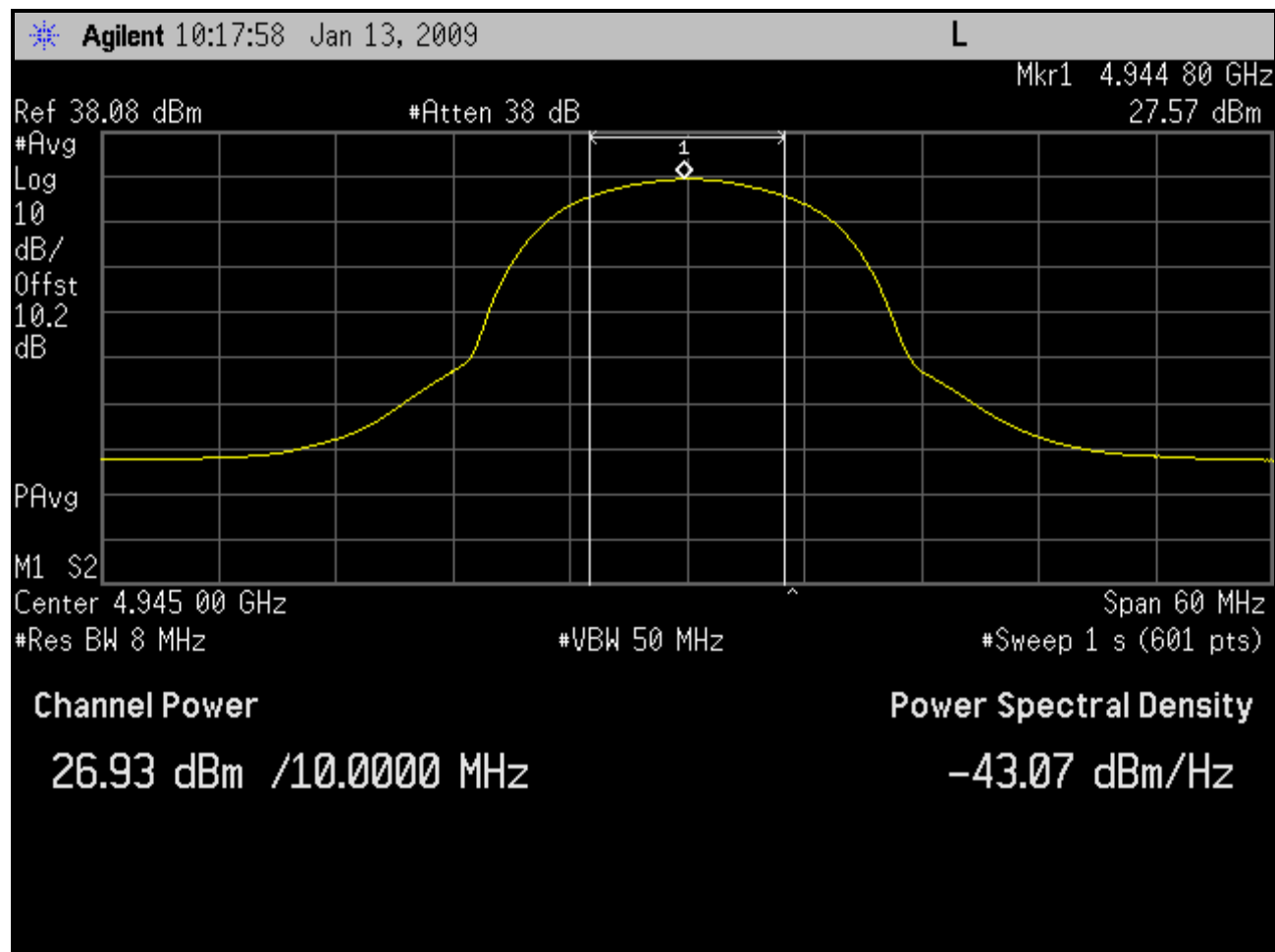
Plot 4-4: Channel Power Output; Channel 1 - 4945 MHz (BS)
