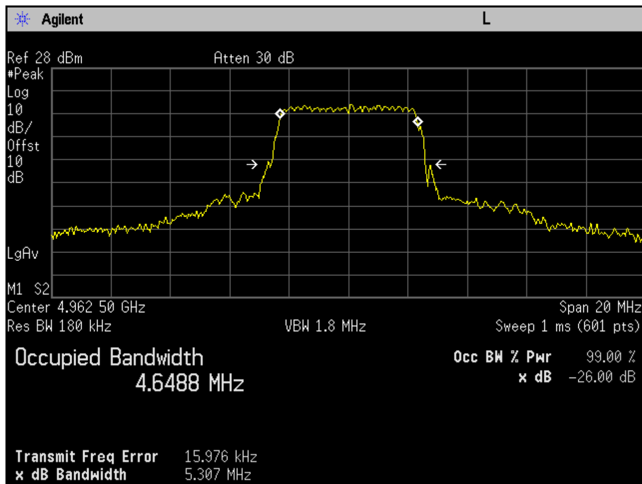
Plot 6-15: Occupied Bandwidth; Channel 5 - 4962.5 MHz (5 MHz BW; SS)
