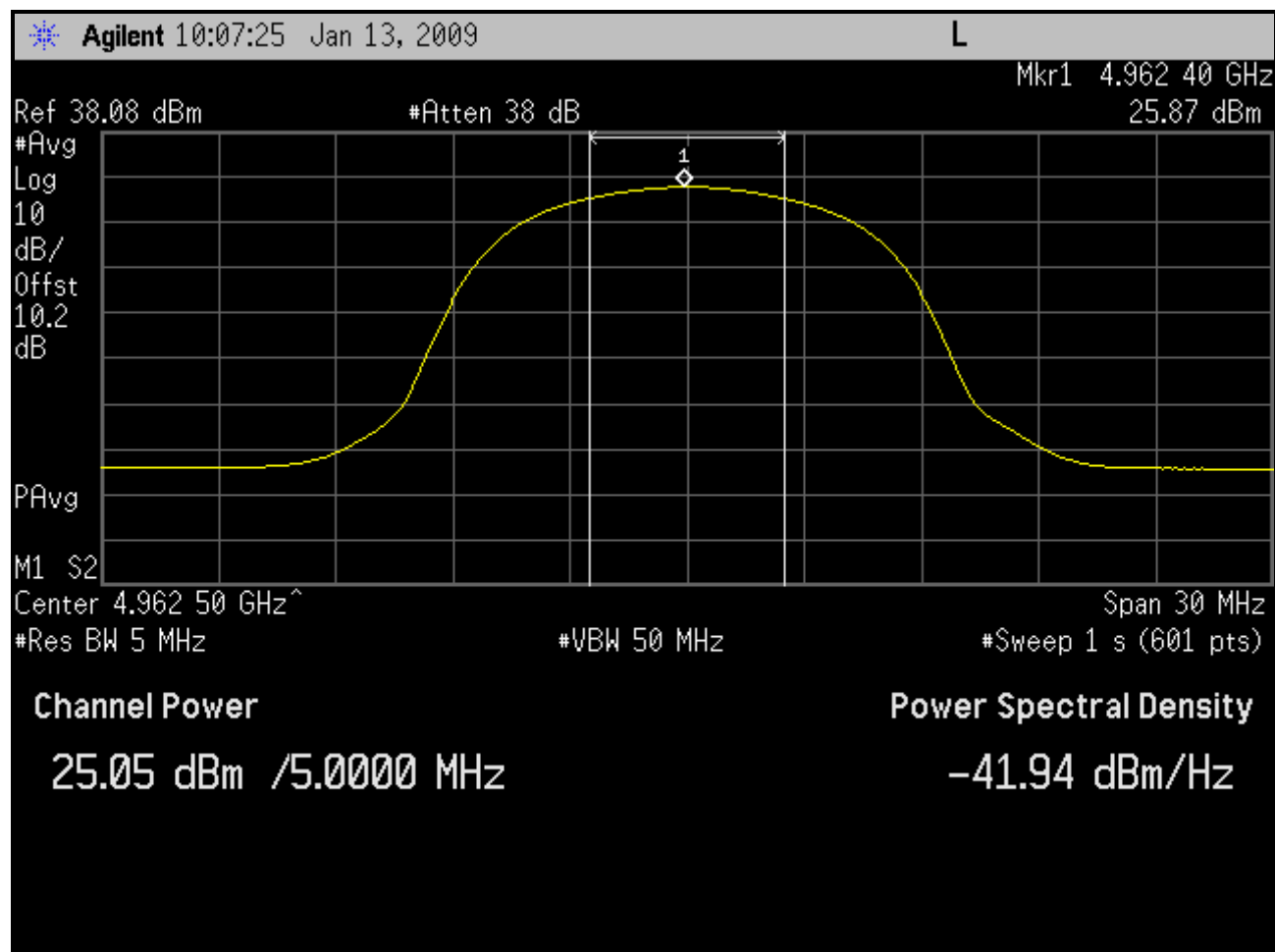
Plot 4-2: Channel Power Output; Channel 5 - 4962.5 MHz (BS)
