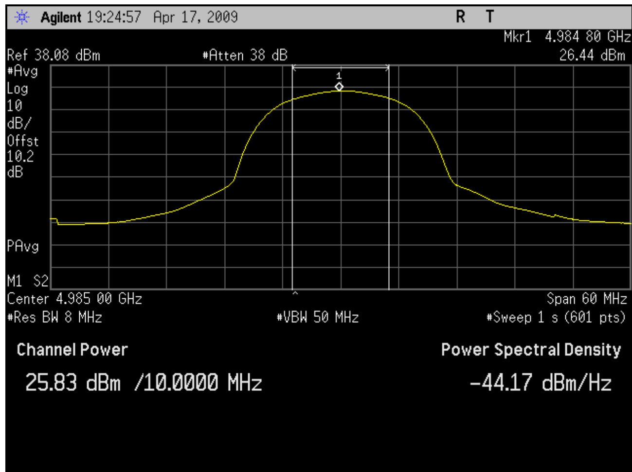
Plot 4-12: Channel Power Output; Channel 5 - 4985 MHz (SS)
