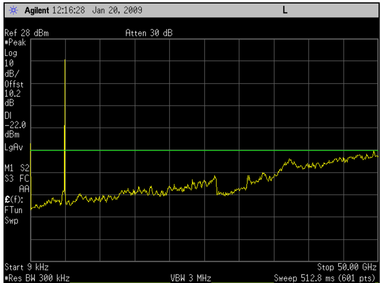
Plot 6-31: Conducted Spurious Emissions; Channel 1 – 4942.5 MHz (5 MHz BW; Full Band; SS)
