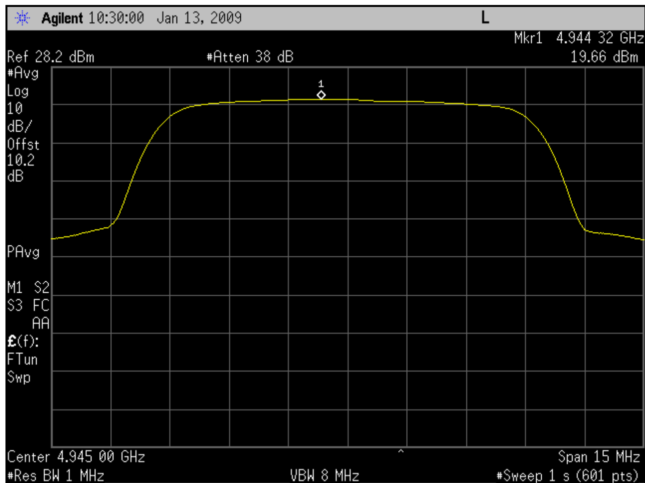
Plot 5-4: Peak Power Spectral Density; Channel 1 - 4945 MHz (BS)
