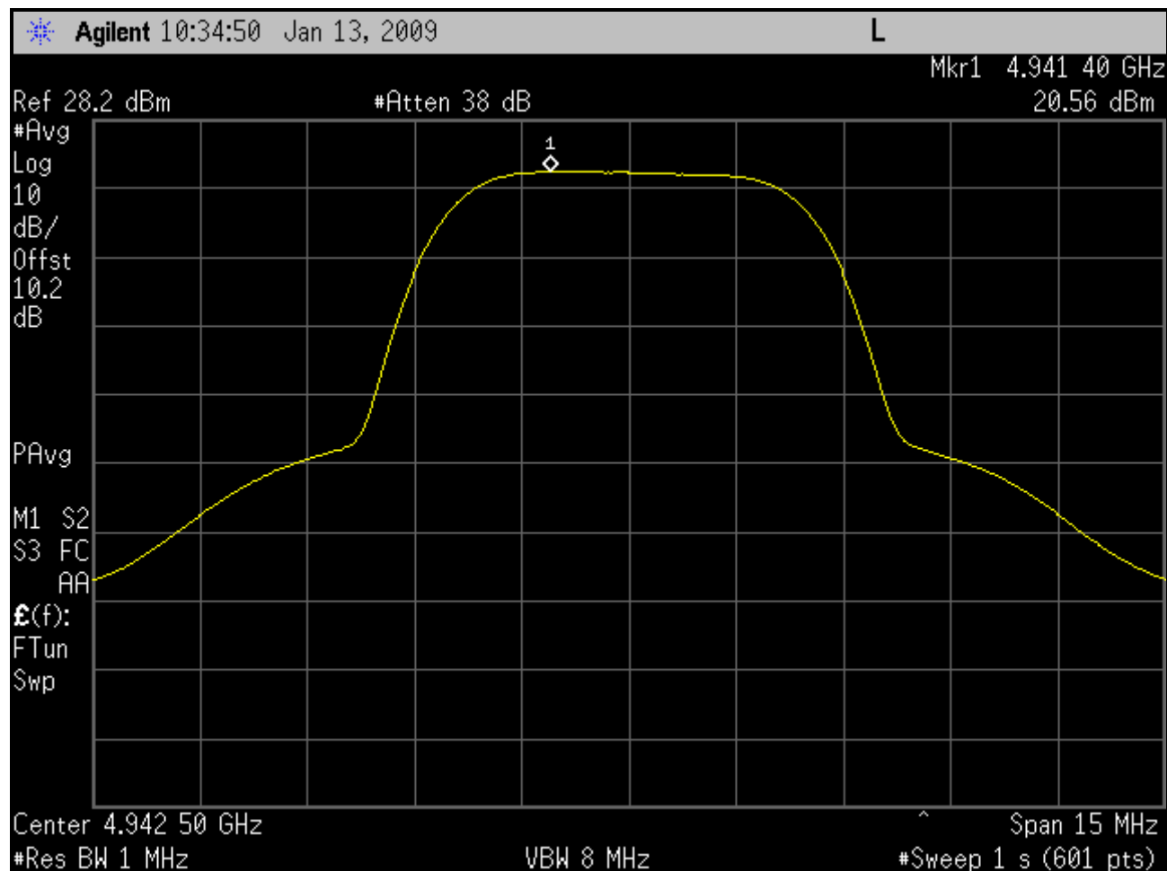
Plot 5-1: Peak Power Spectral Density; Channel 1 - 4942.5 MHz (BS)
