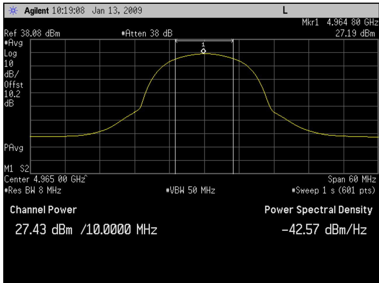
Plot 4-5: Channel Power Output; Channel 3 - 4965 MHz (BS)
