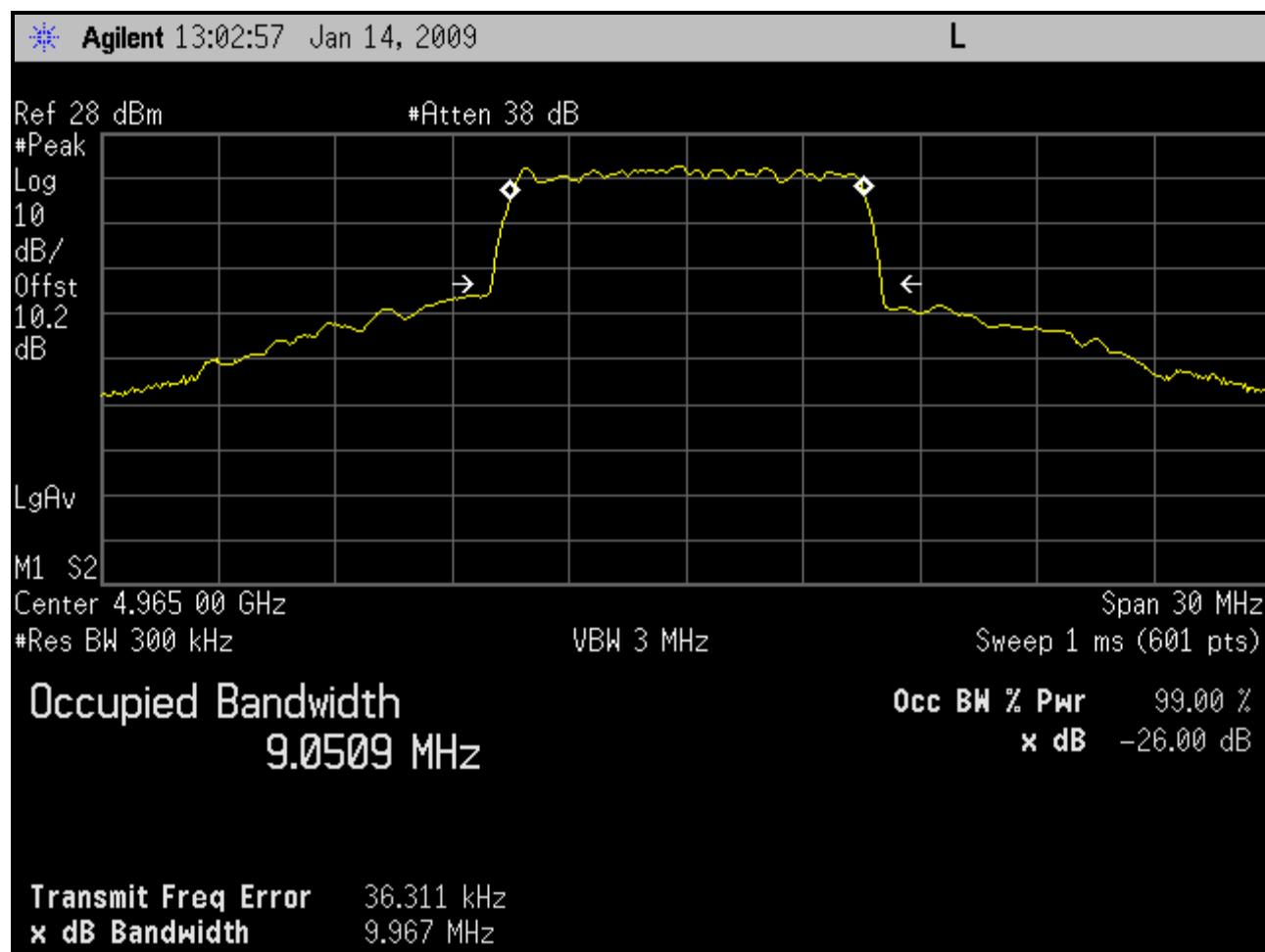
Plot 6-9: Occupied Bandwidth; Channel 3 - 4965 MHz (10 MHz BW; BS)
