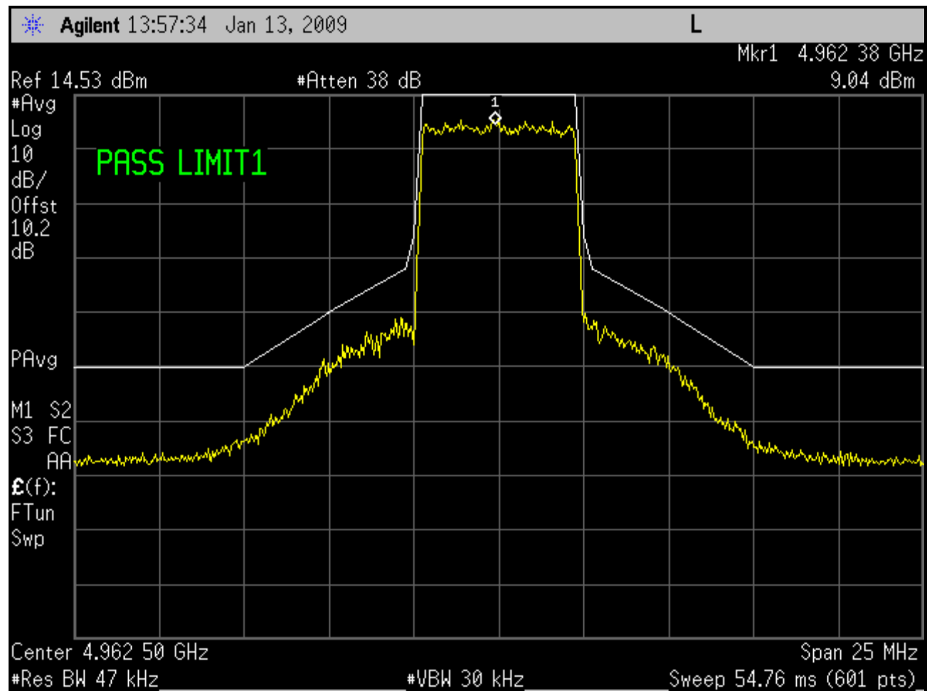
Plot 6-4: Emissions Mask M; Channel 5 - 4962.5 MHz (5 MHz BW; BS)
