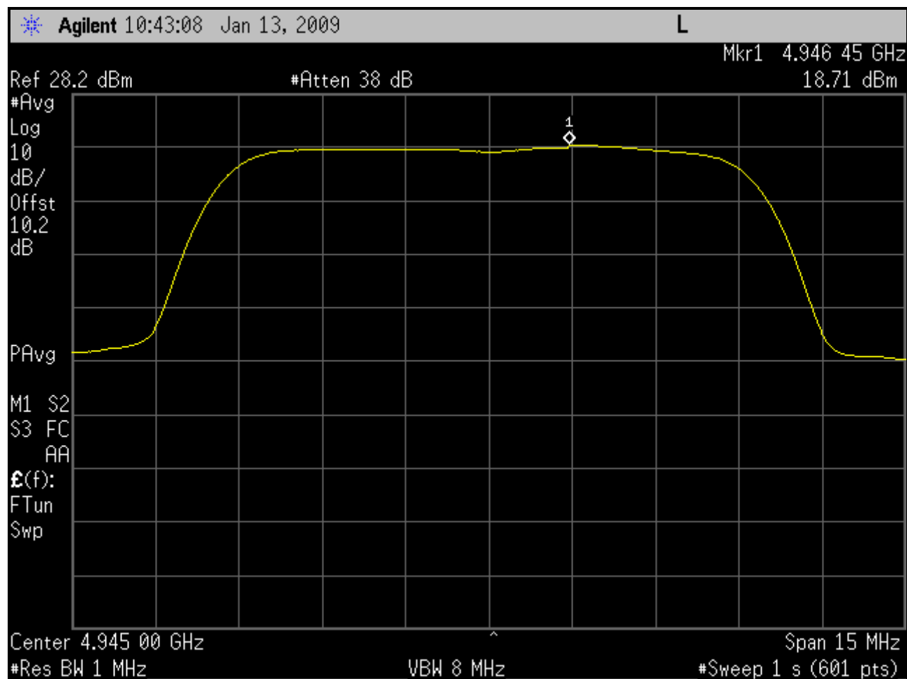
Plot 5-10: Peak Power Spectral Density; Channel 1 - 4945 MHz (SS)
