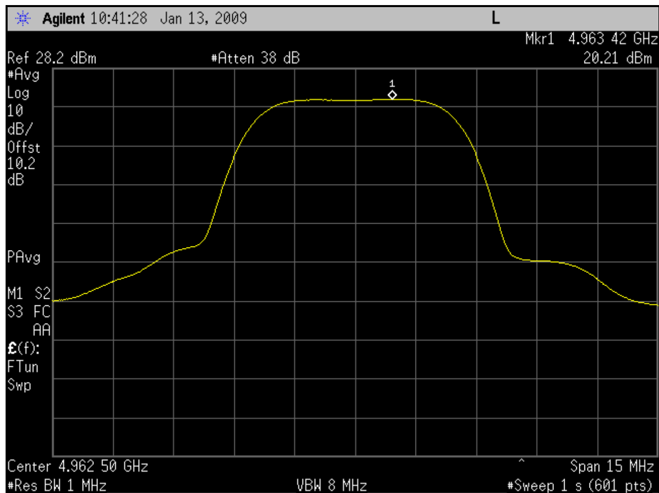
Plot 5-8: Peak Power Spectral Density; Channel 5 - 4962.5 MHz (SS)
