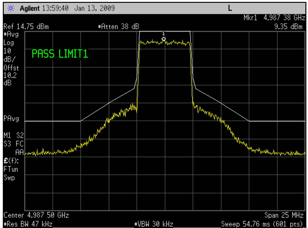
Plot 6-6: Emissions Mask M; Channel 10 - 4987.5 MHz (5 MHz BW; BS)
