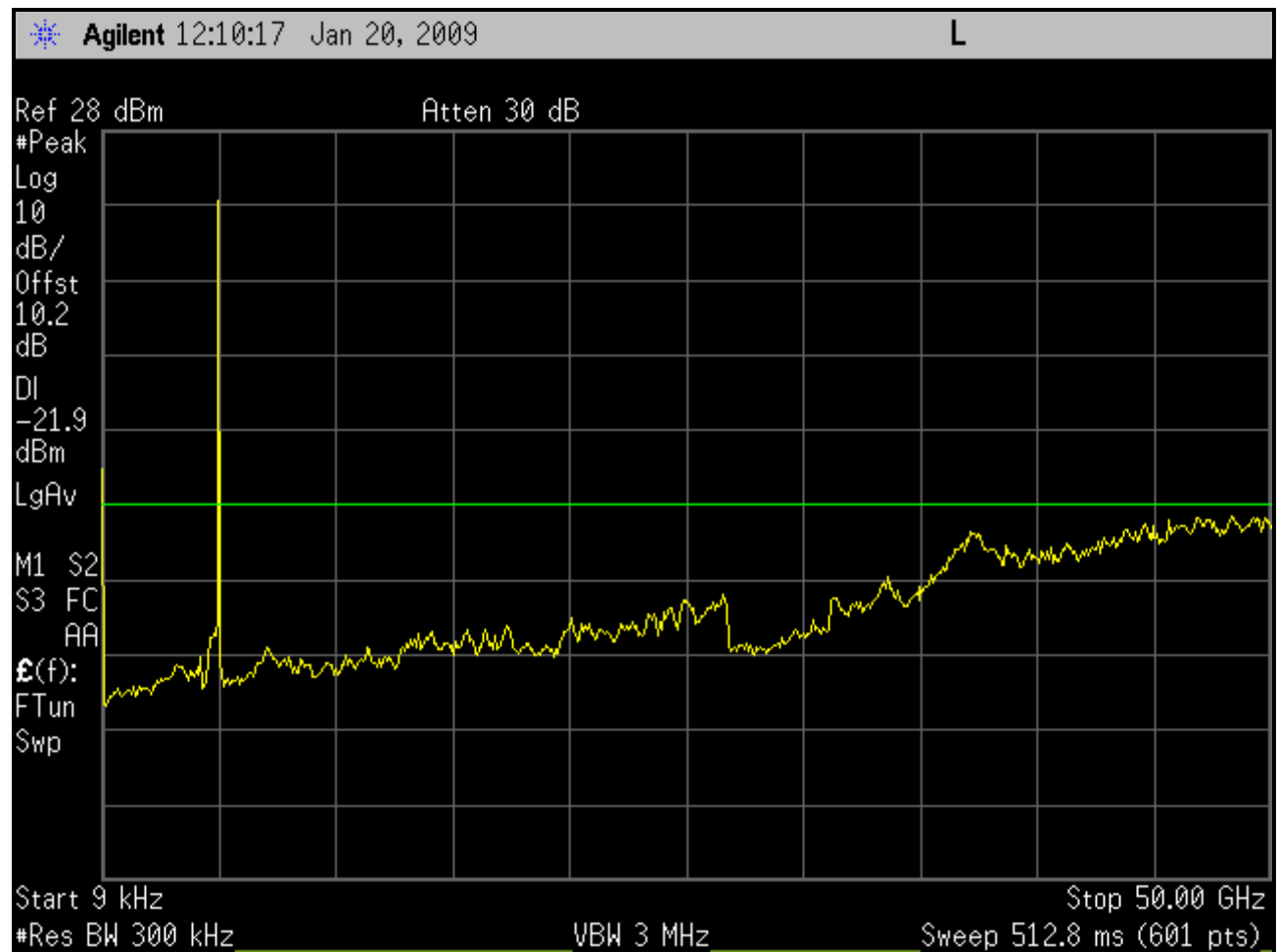
Plot 6-36: Conducted Spurious Emissions; Channel 5 – 4985 MHz (10 MHz BW; Full Band; SS)
