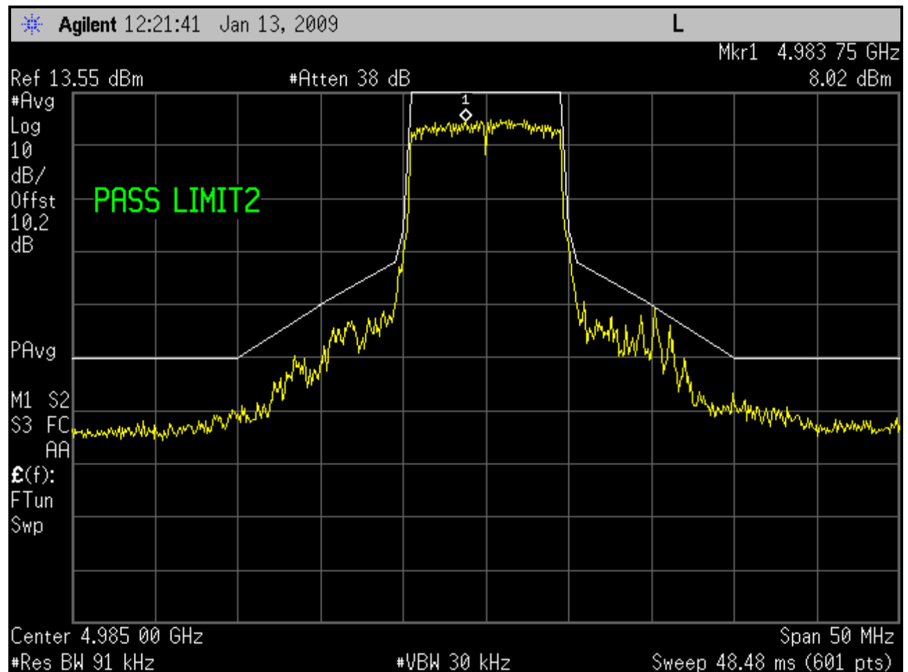
Plot 6-24: Emissions Mask M; Channel 5 - 4985 MHz (10 MHz BW; SS)
