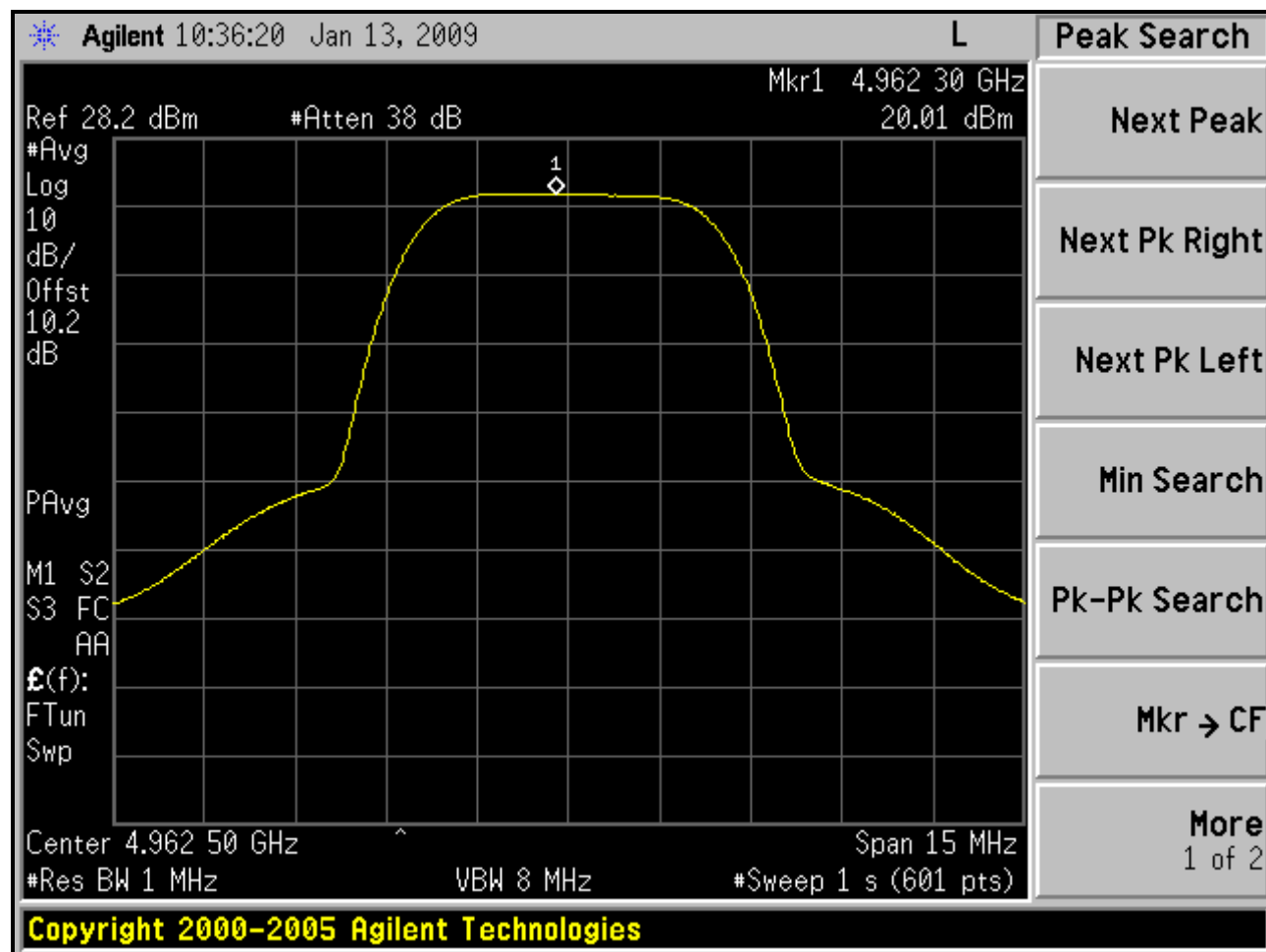
Plot 5-2: Peak Power Spectral Density; Channel 5 - 4962.5 MHz (BS)
