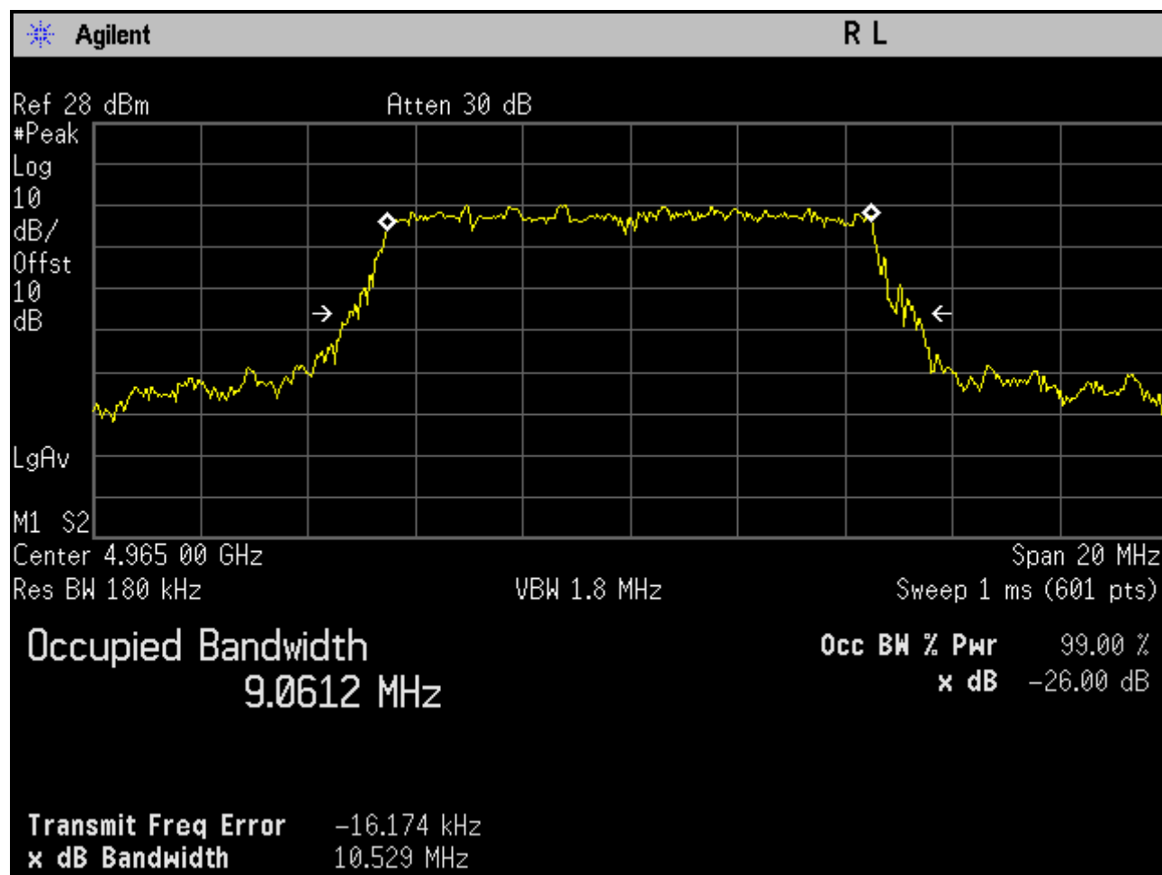
Plot 6-21: Occupied Bandwidth; Channel 3 - 4965 MHz (10 MHz BW; SS)
