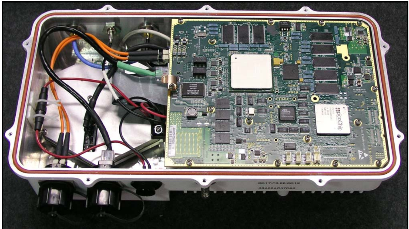
Photograph 8: Internal View
