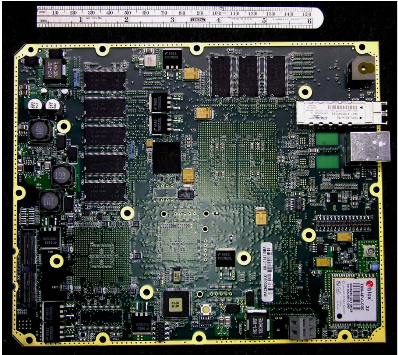
Photograph 11: Digital Board Side 1
