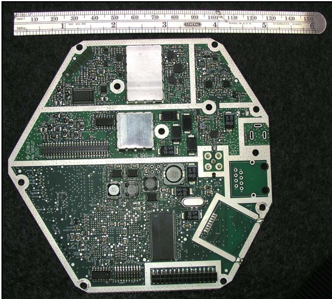
Photograph 13: Client PCB Side 1
