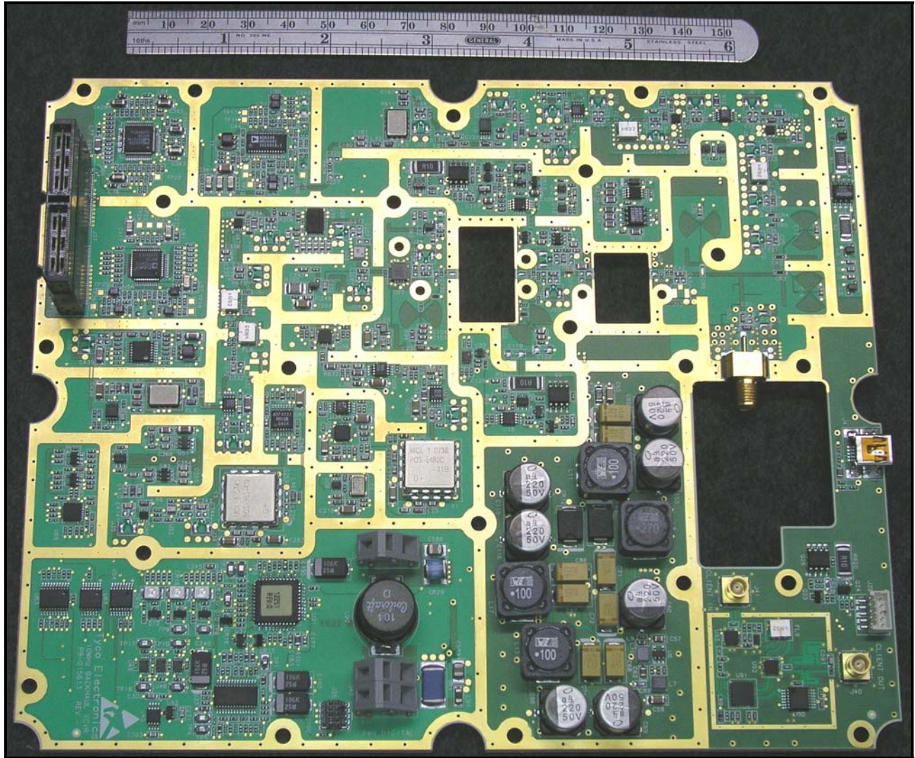
Photograph 9: RF PCB Side 1
