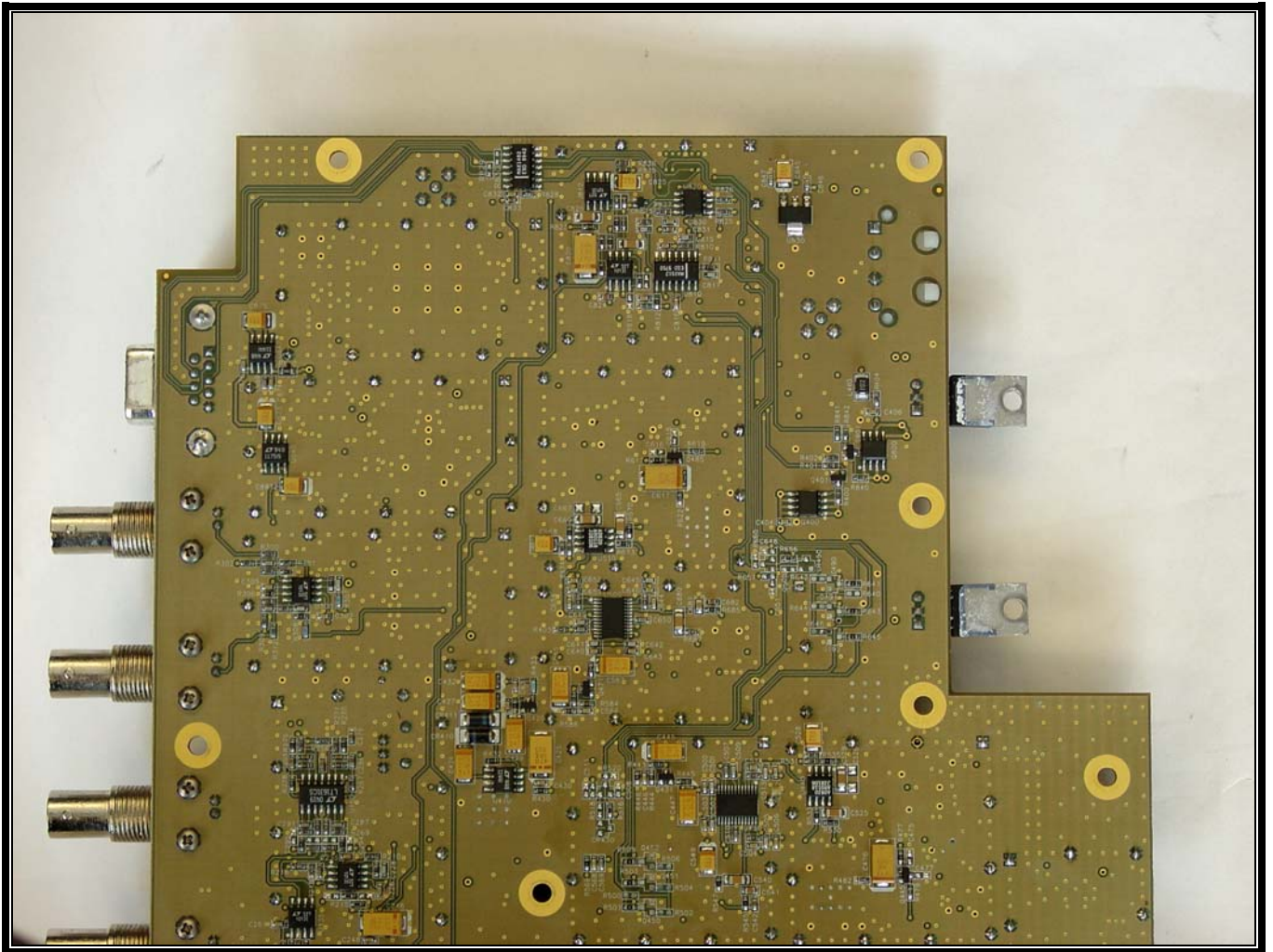
Photograph 29: BSX PCB – Bottom View, Upper Left and Right Corners
