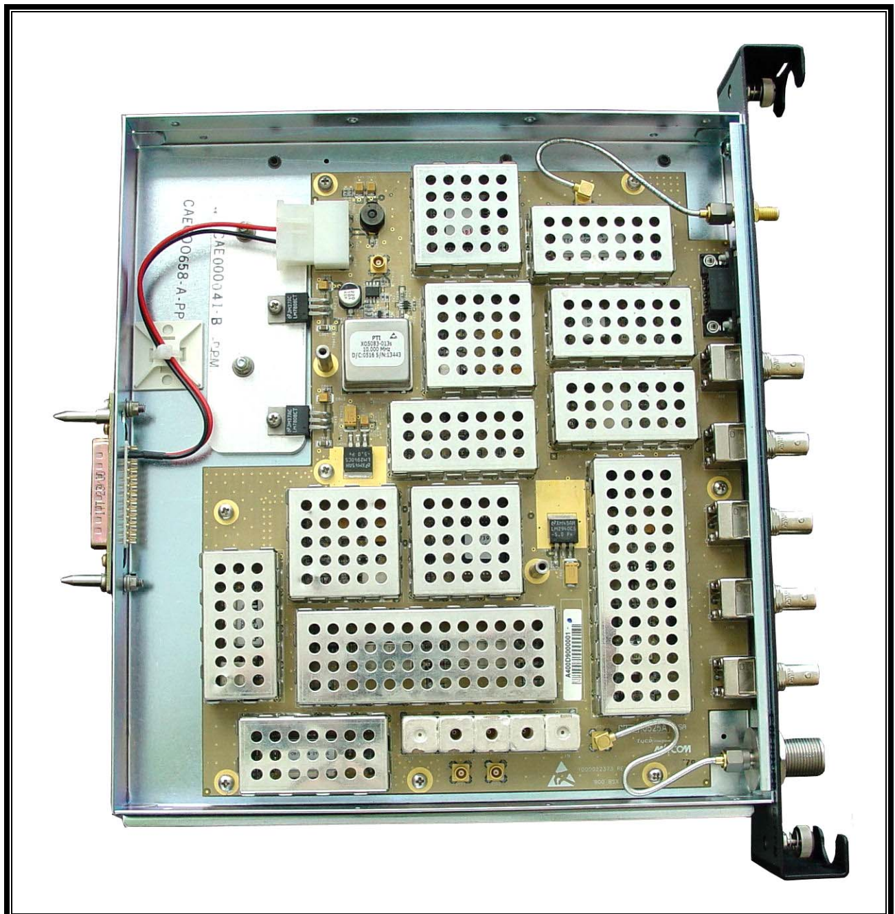
Photograph 26: BSX Without Cover – Top View
