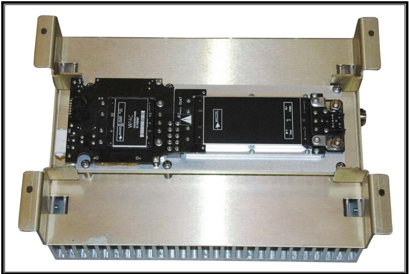
Photograph 20: HPA Underside RF Deck (Power Supply)
