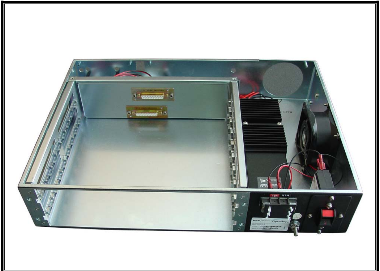
Photograph 25: DCX Without Cover – Rear View
