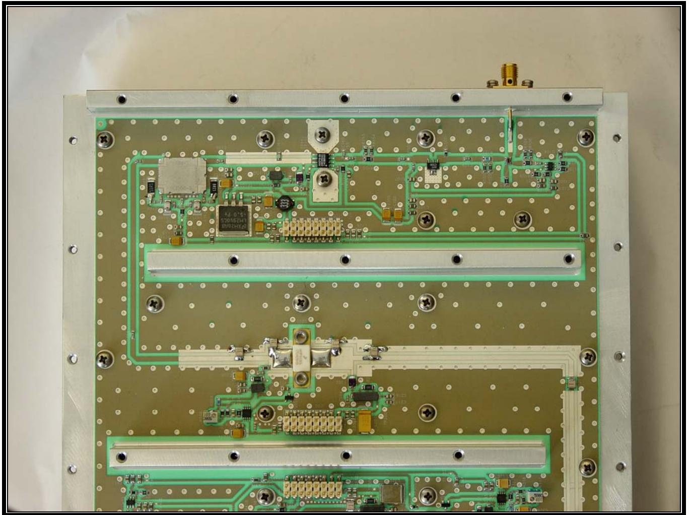
Photograph 13: HPA RF Deck – Top View, Upper Left and Right Corners
