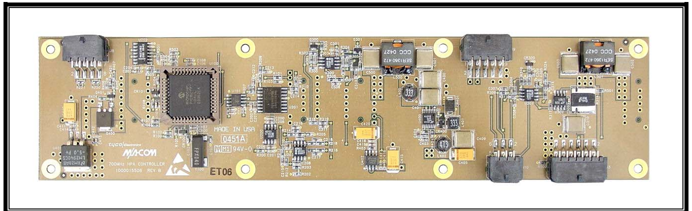
Photograph 21: HPA Controller PCB - Top View
