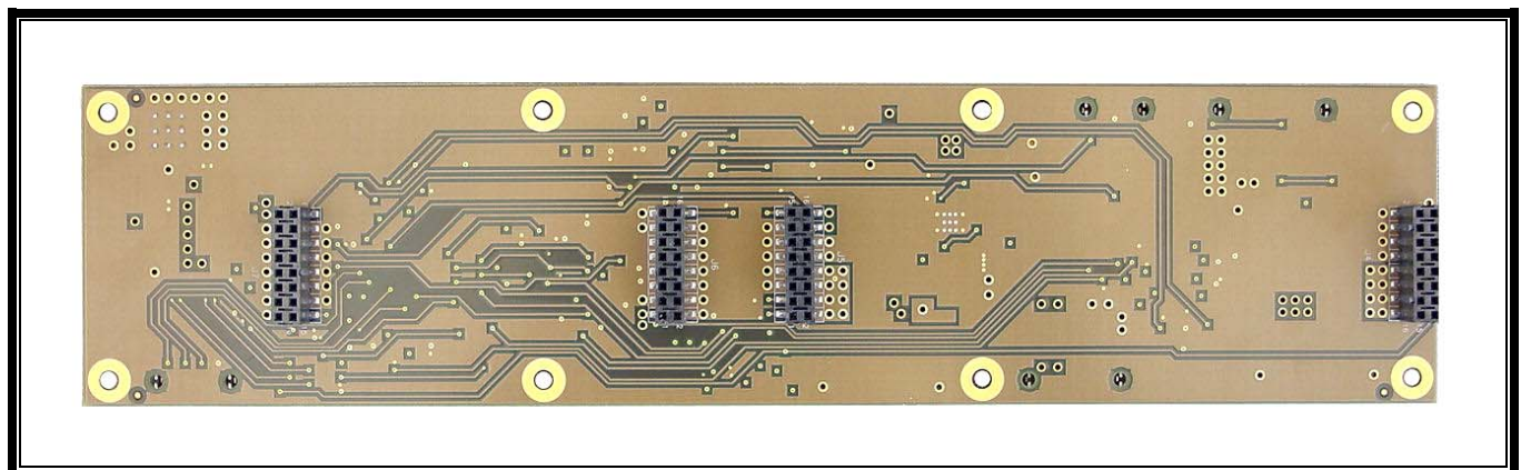
Photograph 22: HPA Controller PCB - Bottom View
