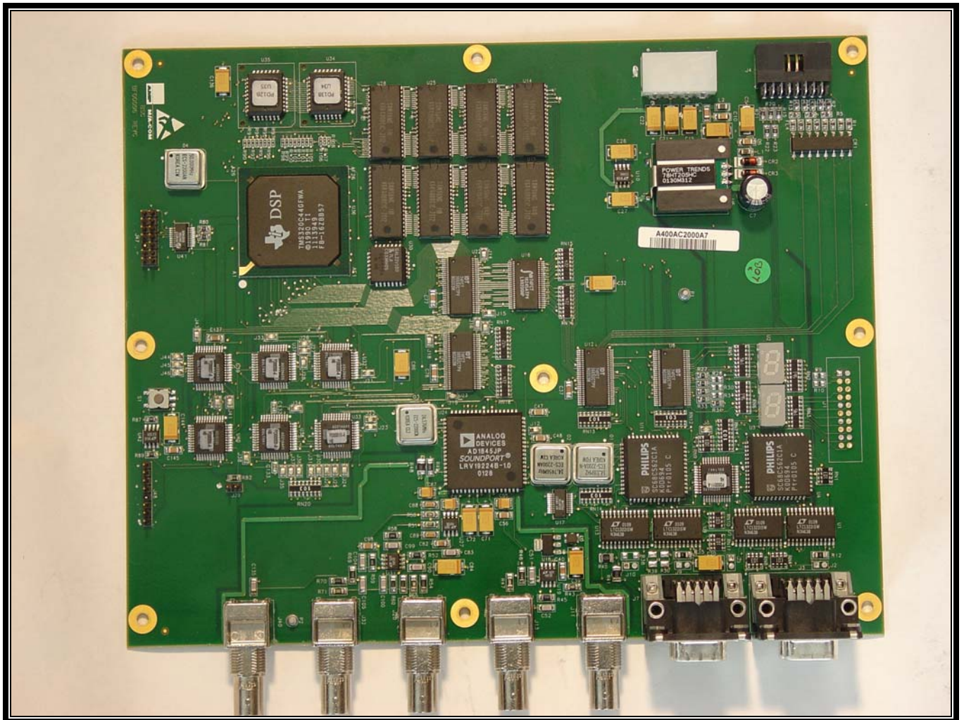
Photograph 32: BSC PCB - Top View
