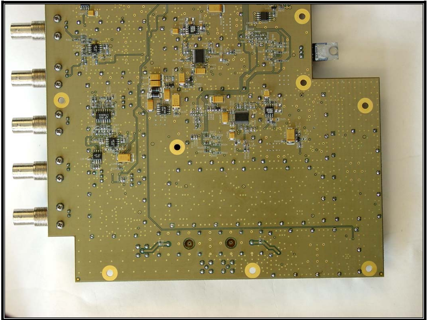
Photograph 30: BSX PCB – Bottom View, Lower Left and Right Corners
