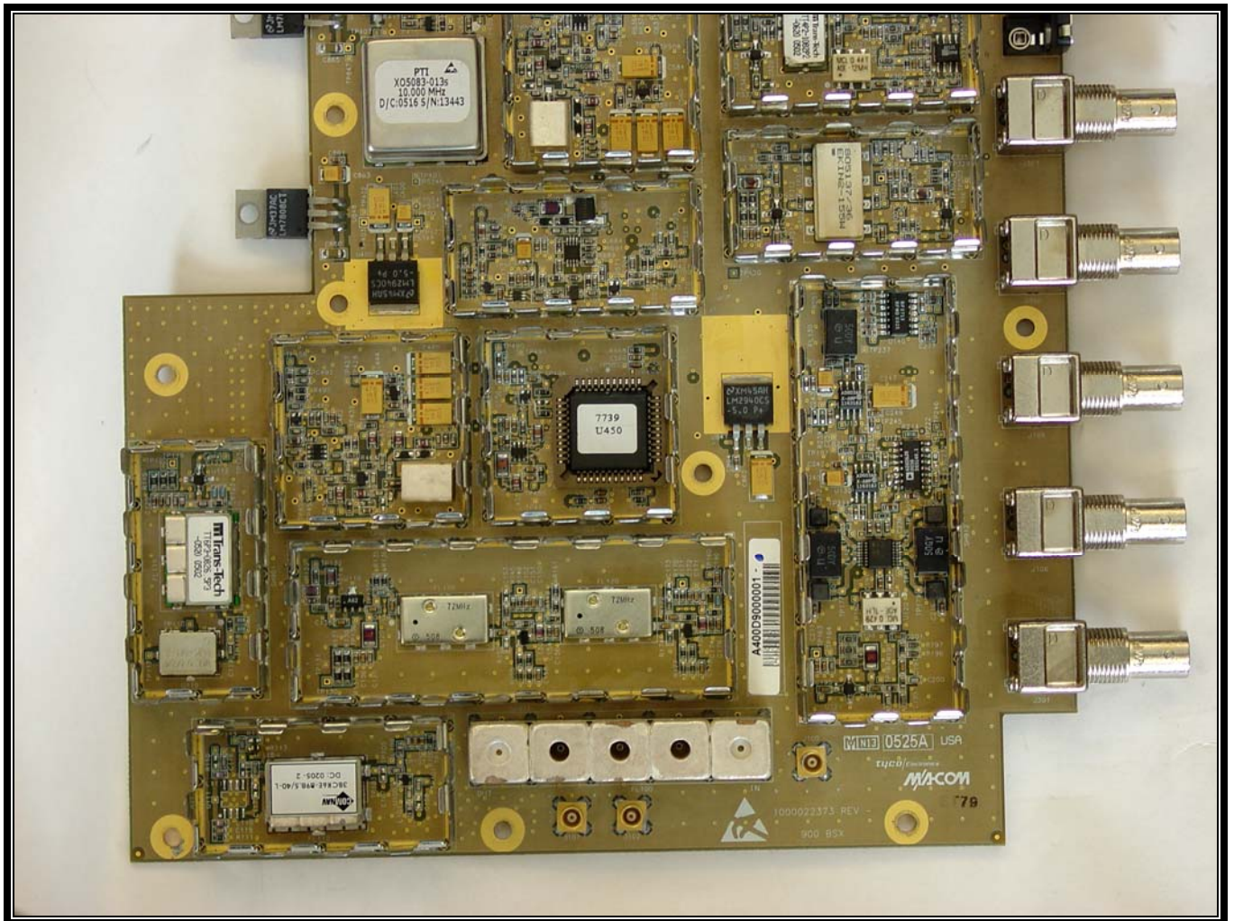
Photograph 28: BSX PCB - Top View, Lower Left and Right Corners
