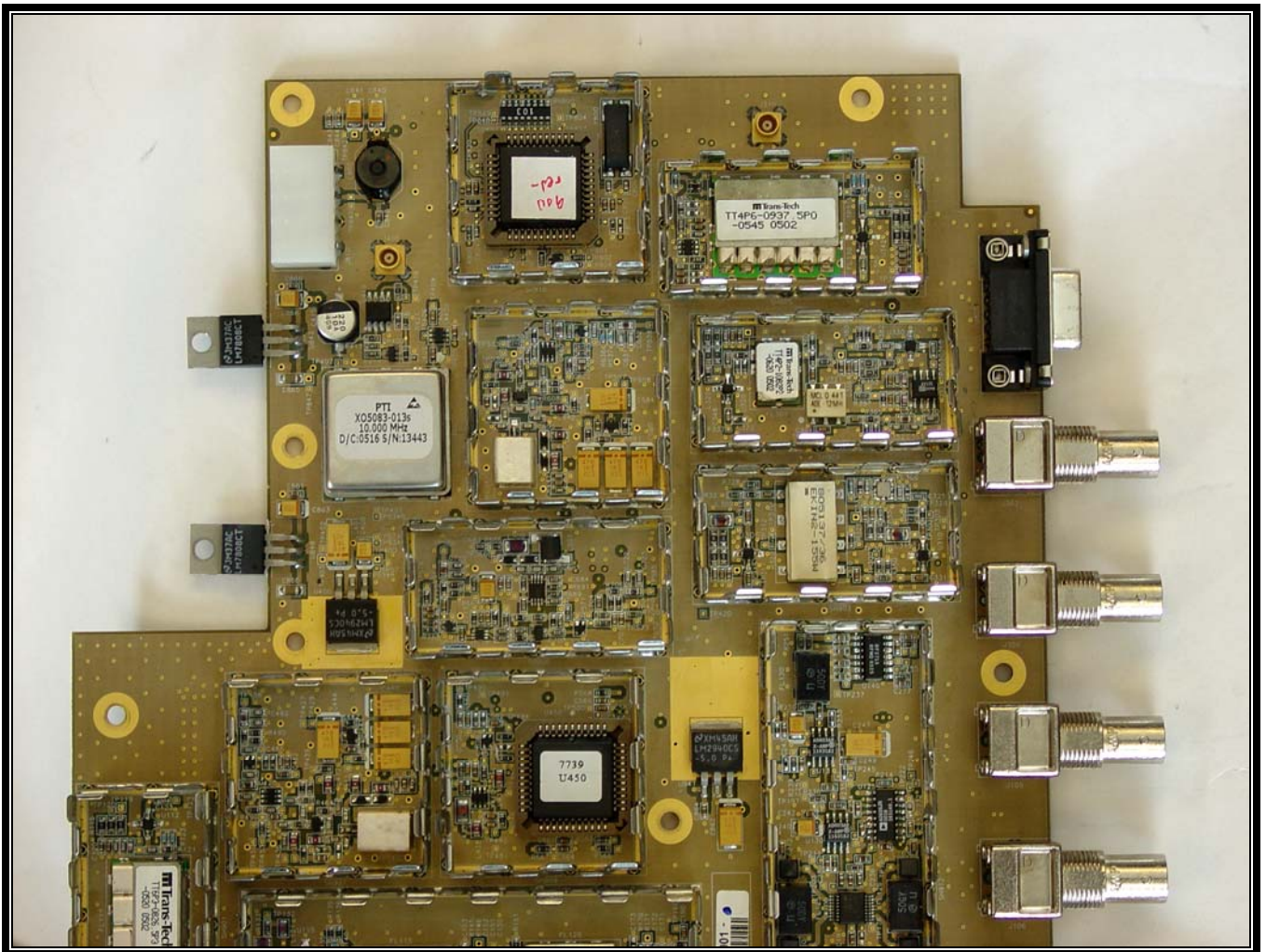
Photograph 27: BSX PCB - Top View, Upper Left and Right Corners
