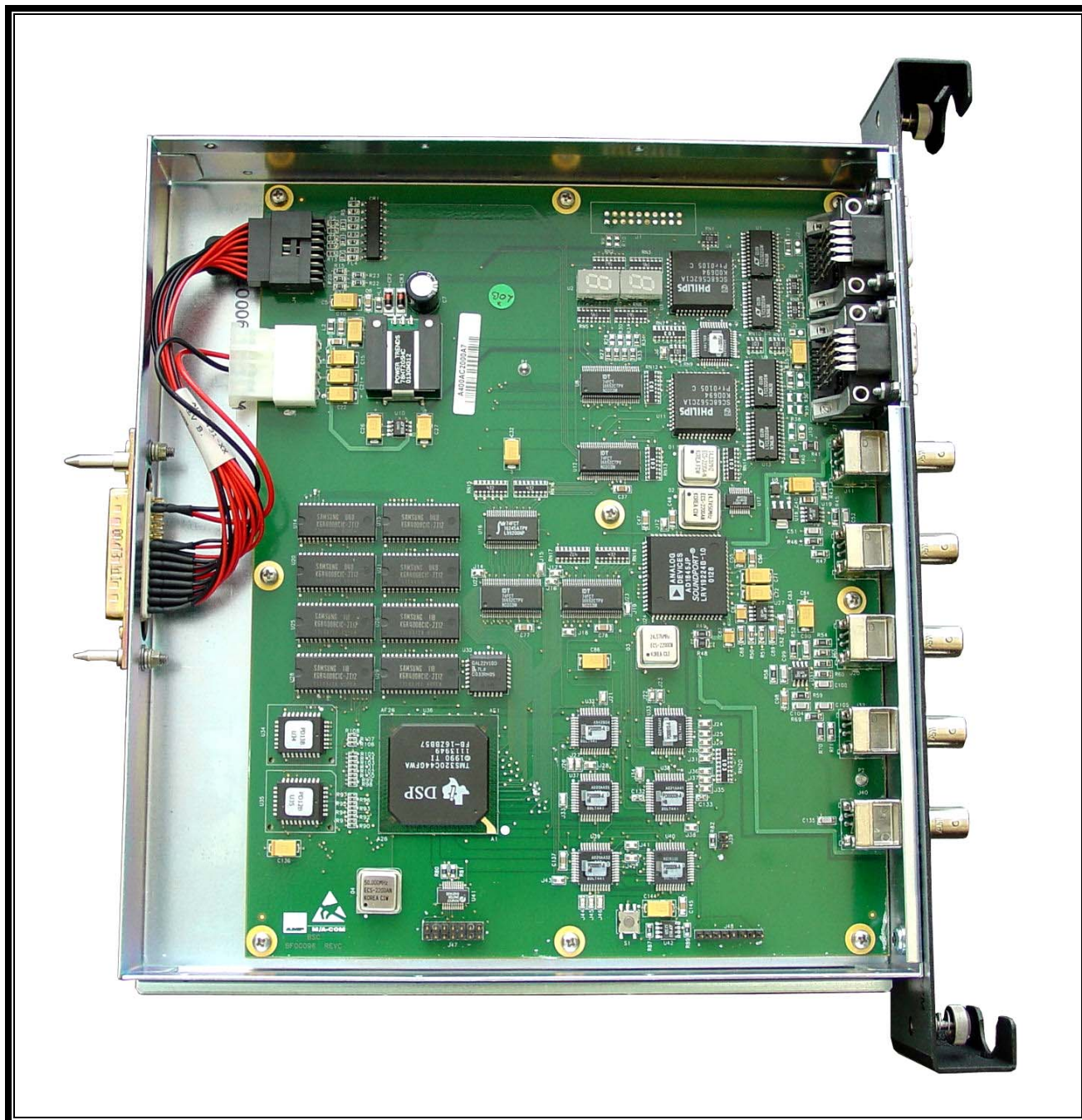
Photograph 31: BSC Without Cover – Top View
