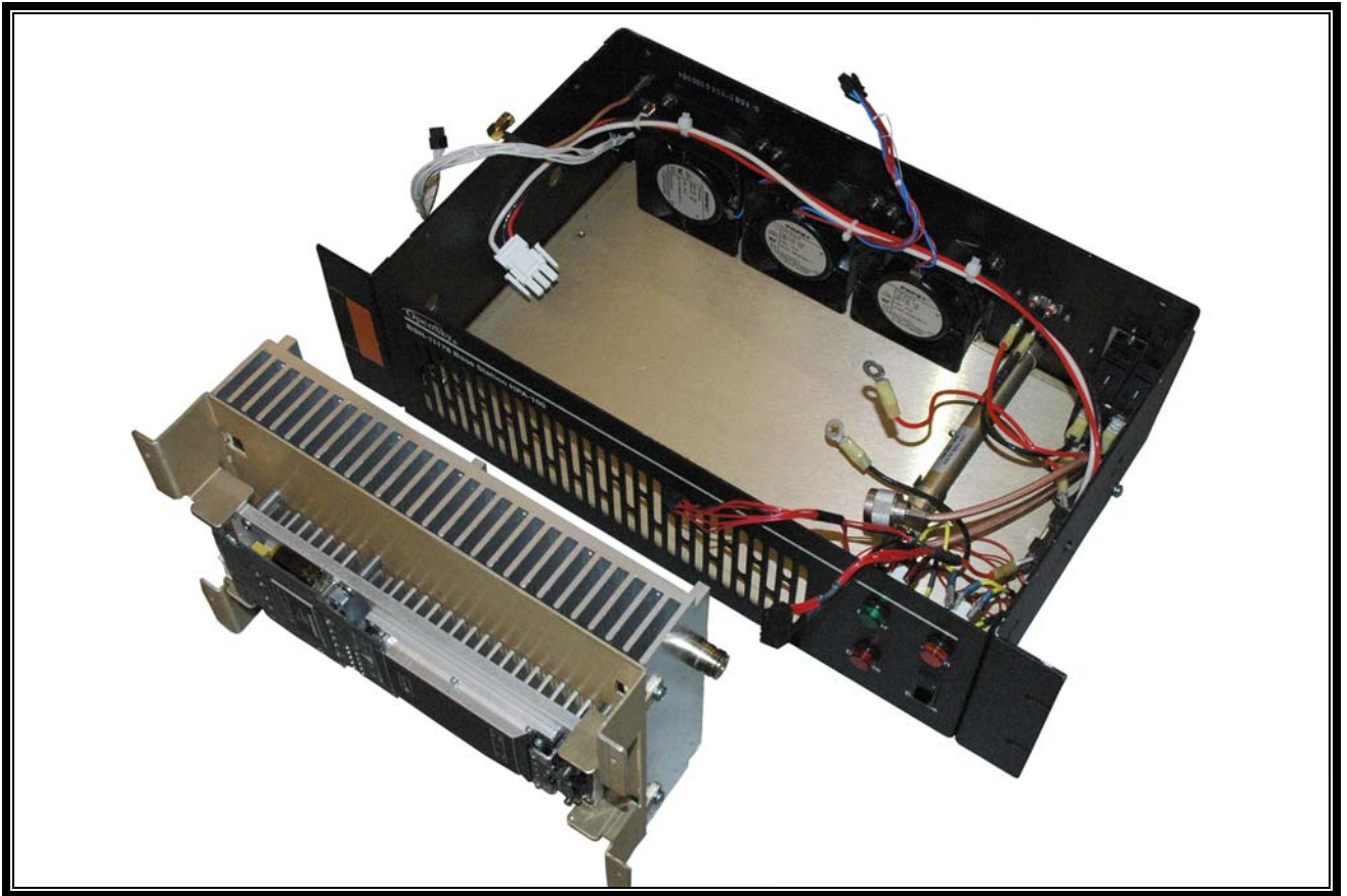
Photograph 15: HPA RF Deck Removed
