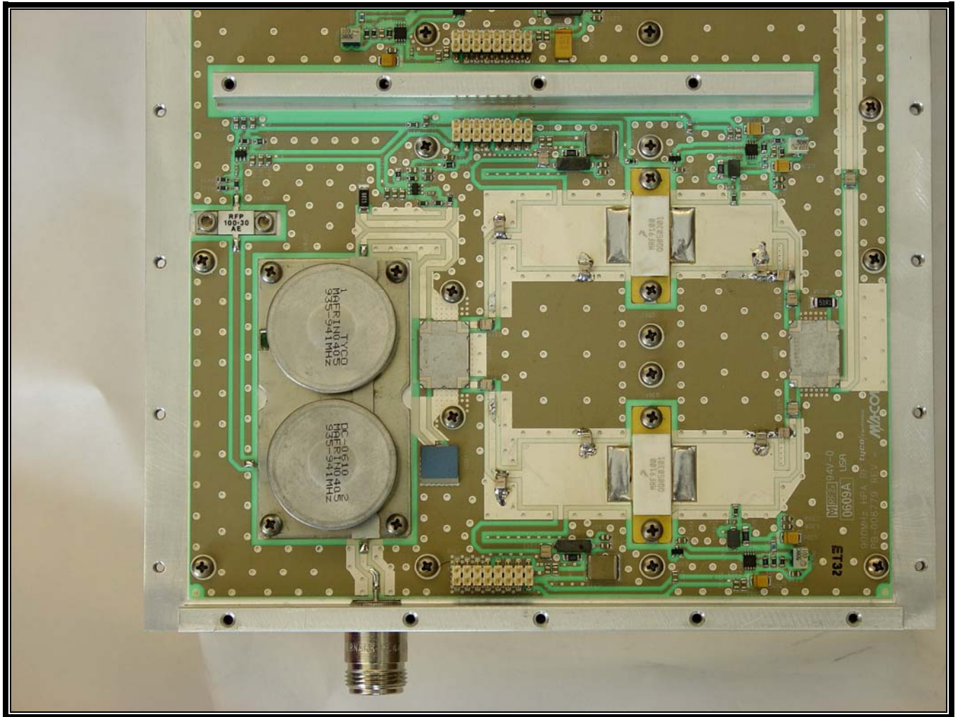
Photograph 14: HPA RF Deck – Top View, Lower Left and Right Corners
