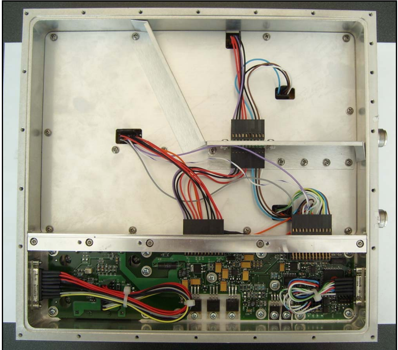
Photograph 18: HPA RF Deck without Cover
