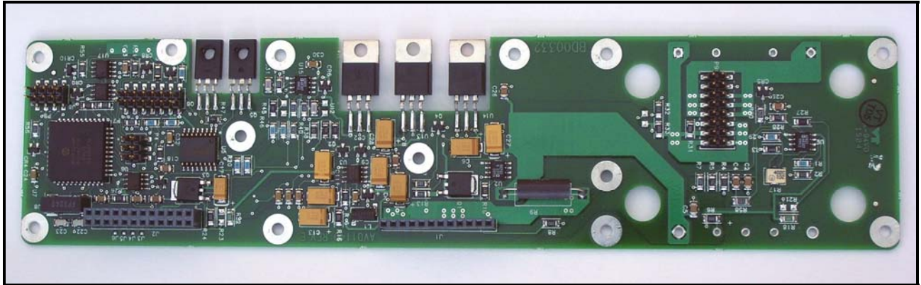
Photograph 23: HPA Controller PCB Top
