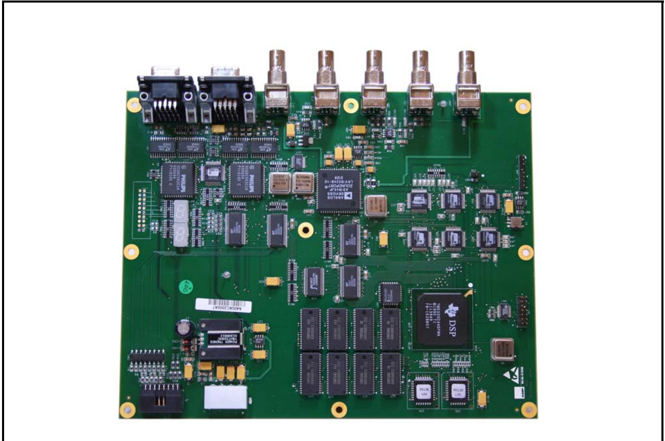
Photograph 26: BSC PCB Top
