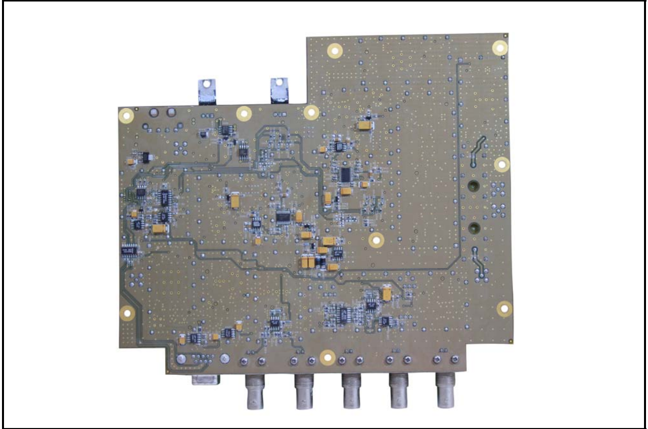
Photograph 30: BSX PCB Bottom
