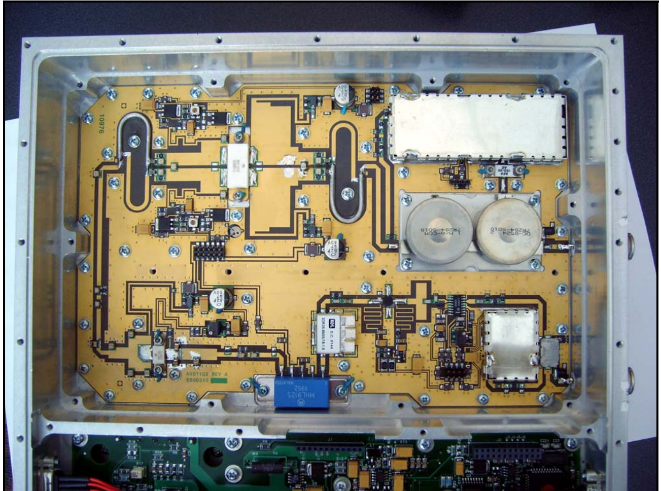
Photograph 19: HPA RF Board Installed in RF Deck
