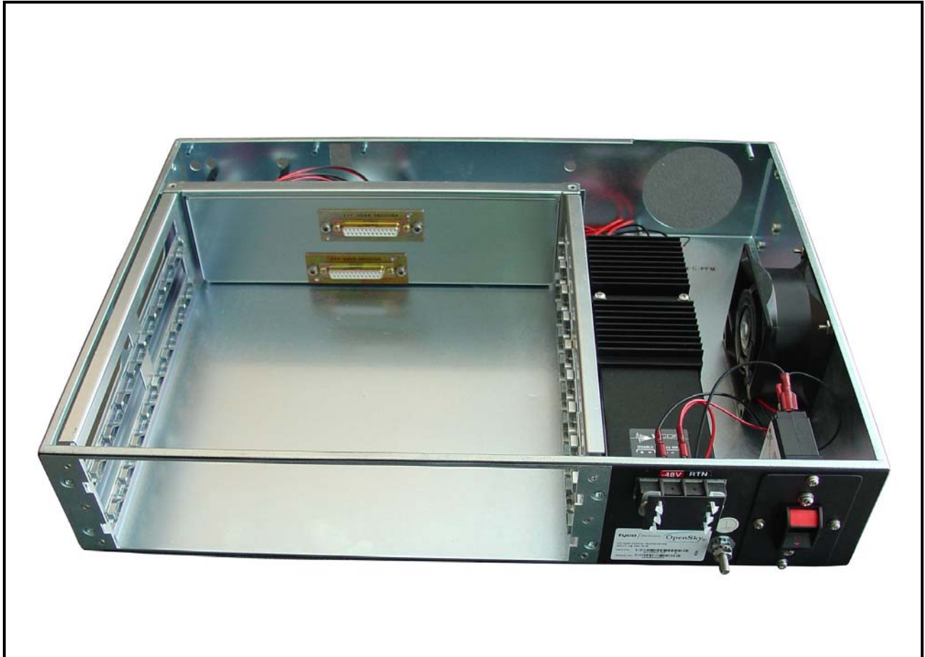
Photograph 33: DCX without Cover Rear
