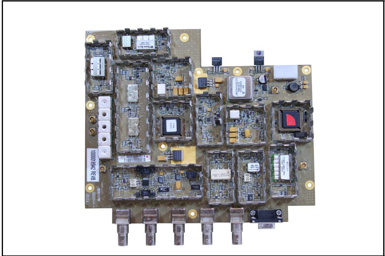
Photograph 29: BSX PCB Top
