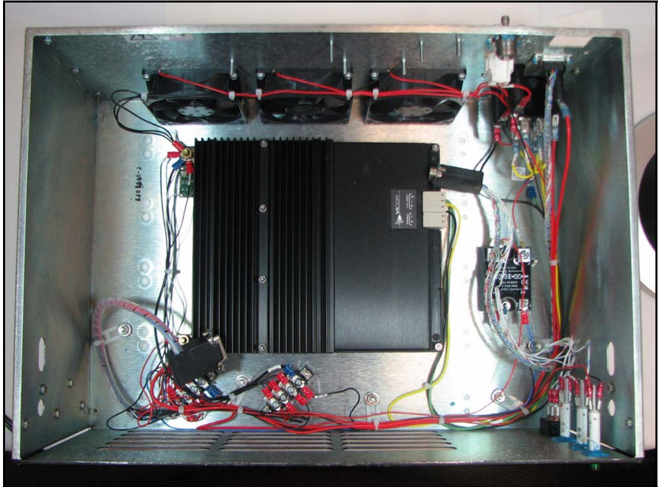
Photograph 20: HPA with RF Deck Removed
