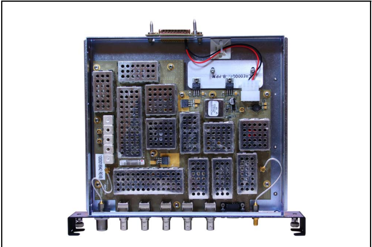
Photograph 28: BSX without cover
