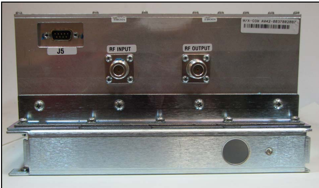
Photograph 9: HPA RF Deck Right
