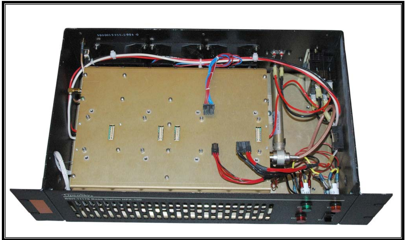
Photograph 25: HPA Without Controller
