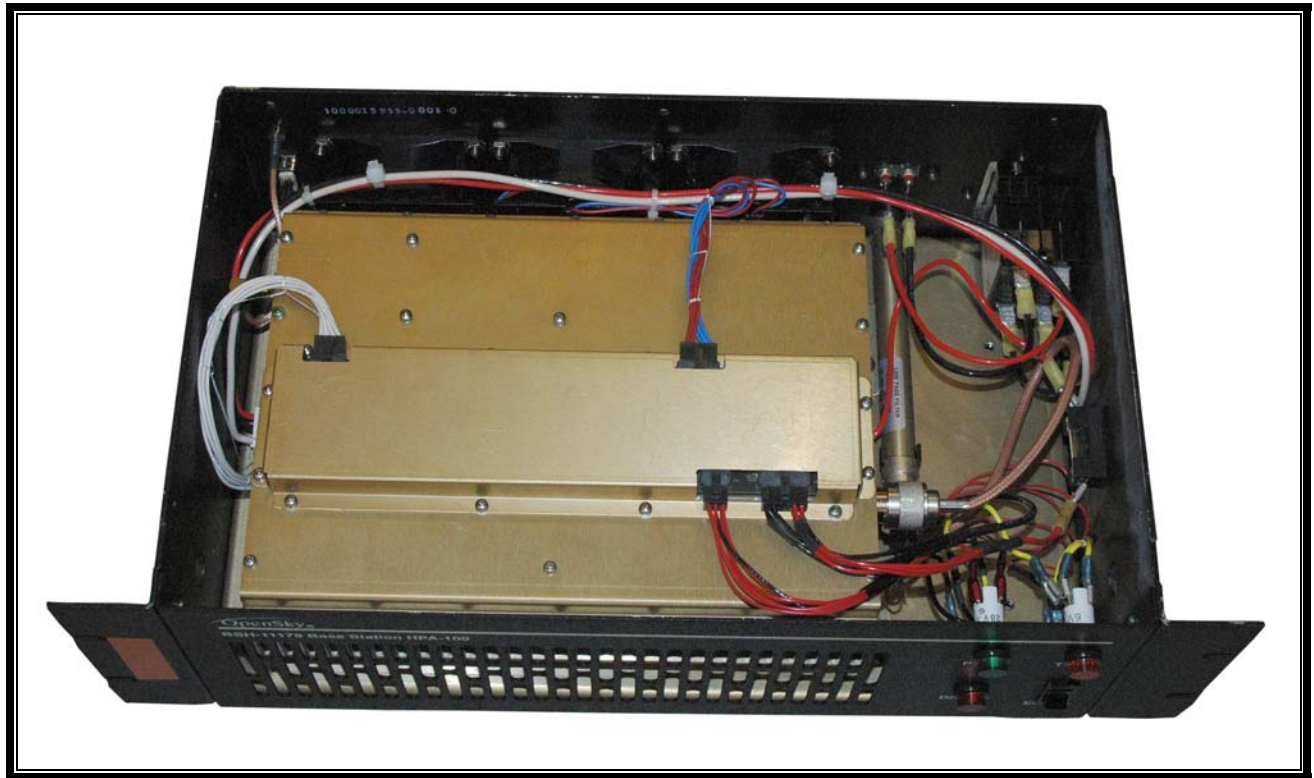
Photograph 23: HPA Without Top Cover
