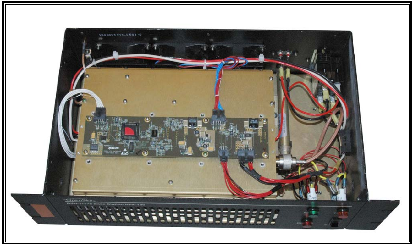
Photograph 24: HPA Without Controller Cover
