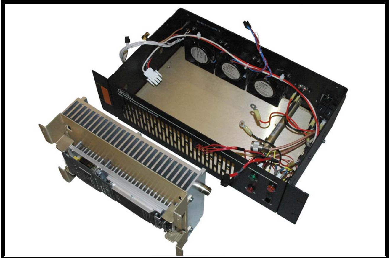
Photograph 26: HPA RF Deck Removed
