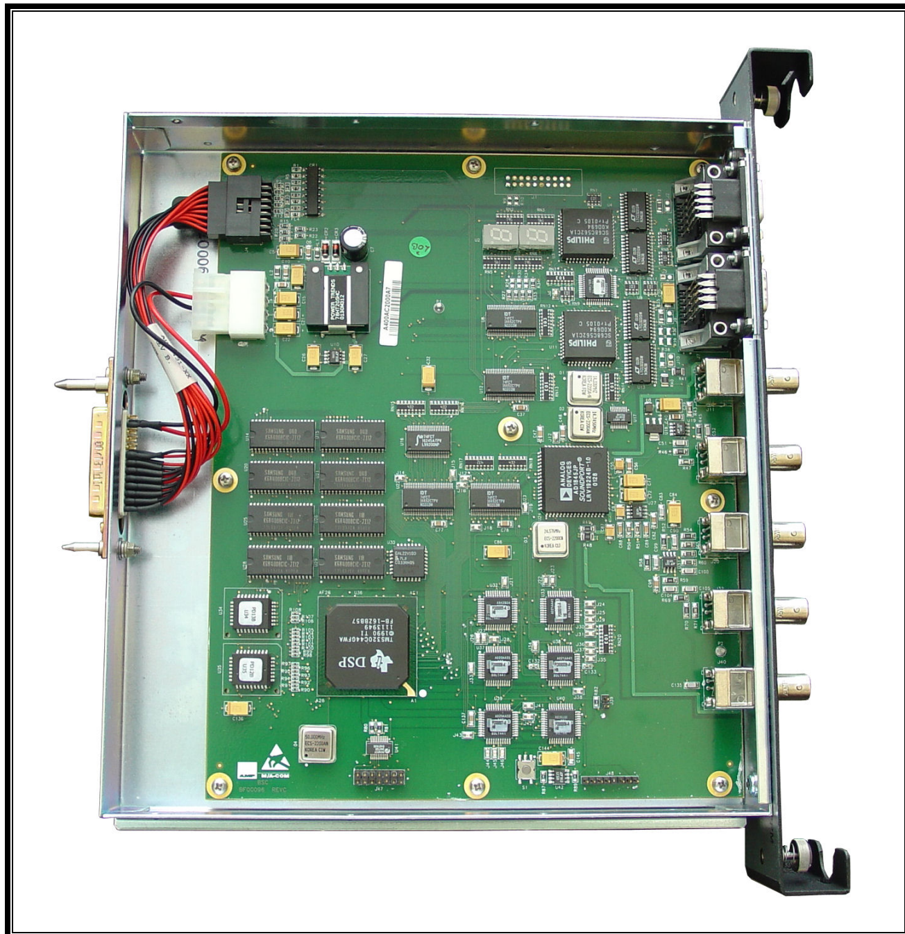
Photograph 14: BSC Without Cover
