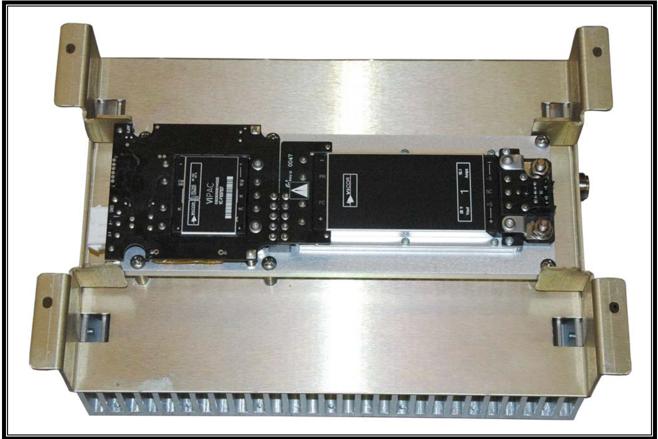
Photograph 28: HPA Underside RF Deck (Power Supply)
