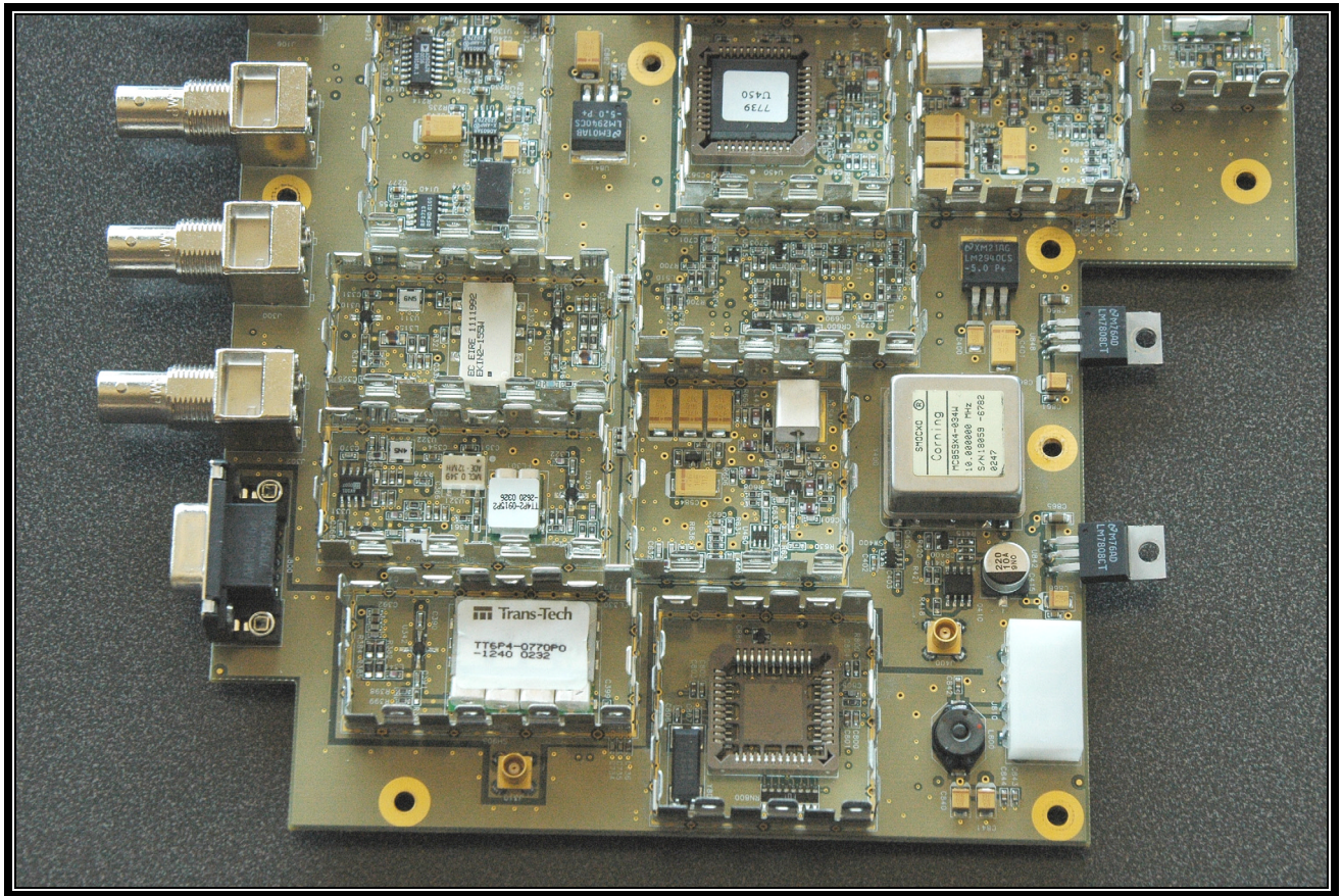
PHOTOGRAPH 29: BSX PCB TOP VIEW (B)
