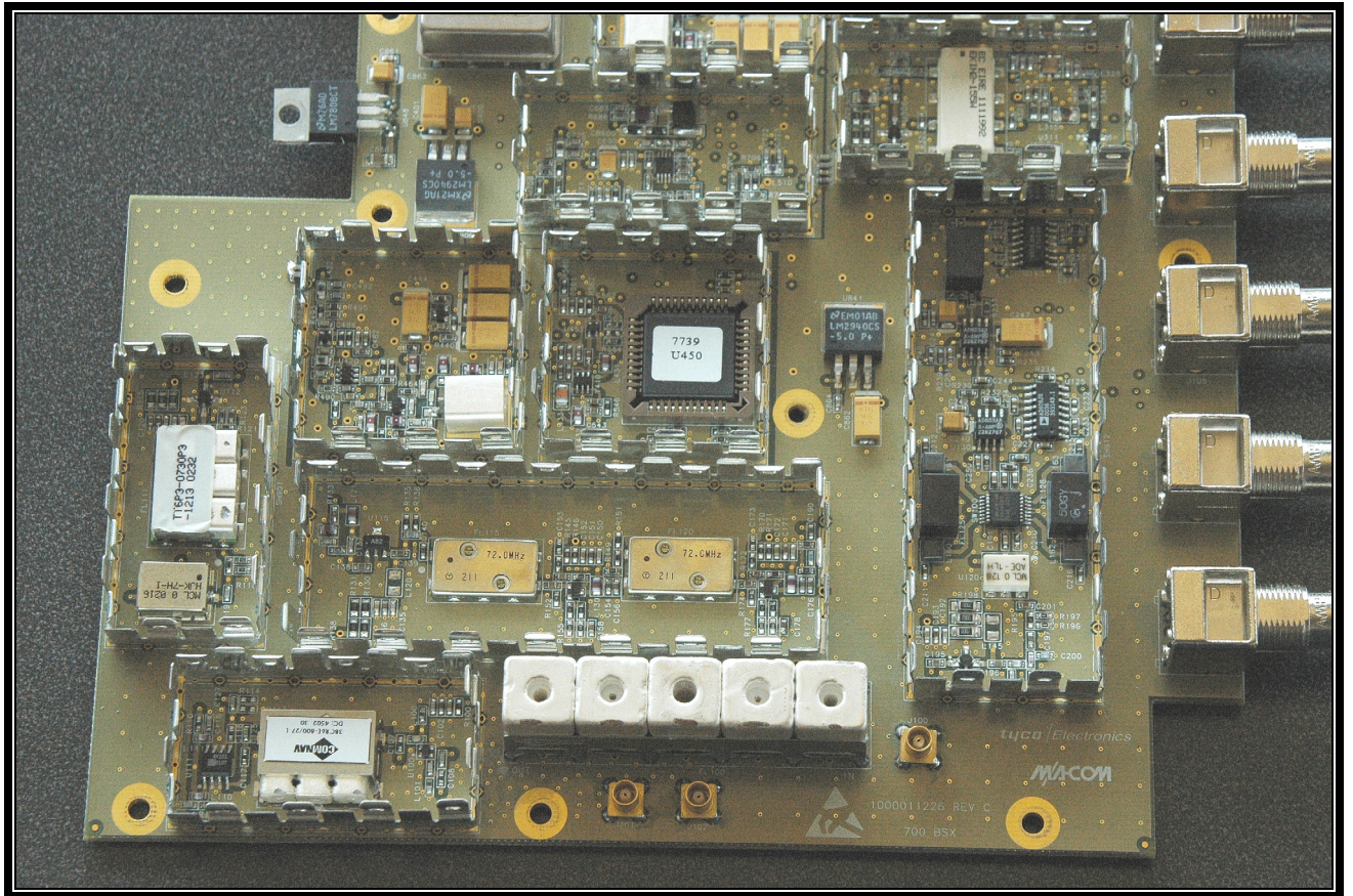
PHOTOGRAPH 19: BSX PCB TOP VIEW (A)
