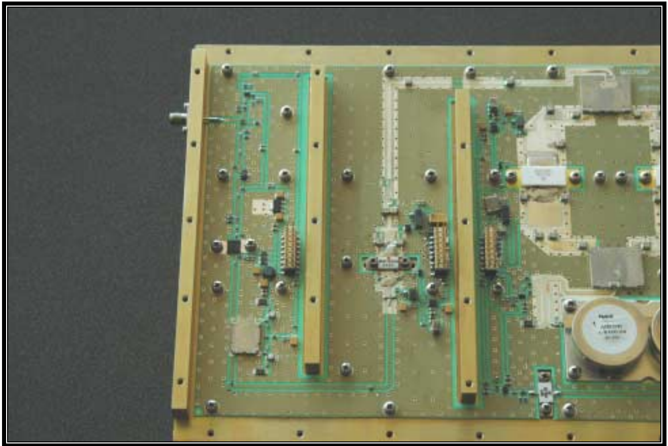
PHOTOGRAPH 21: HPA RF AMP (LEFT SIDE)
