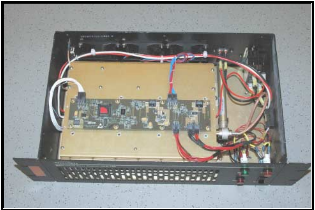
PHOTOGRAPH 11: HPA CONTROLLER WITHOUT COVER
