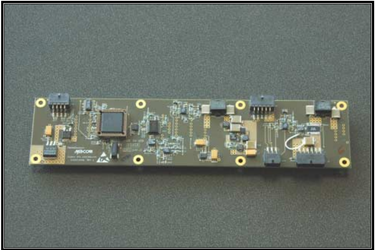
PHOTOGRAPH 12: HPA CONTROLLER PCB FRONT VIEW
