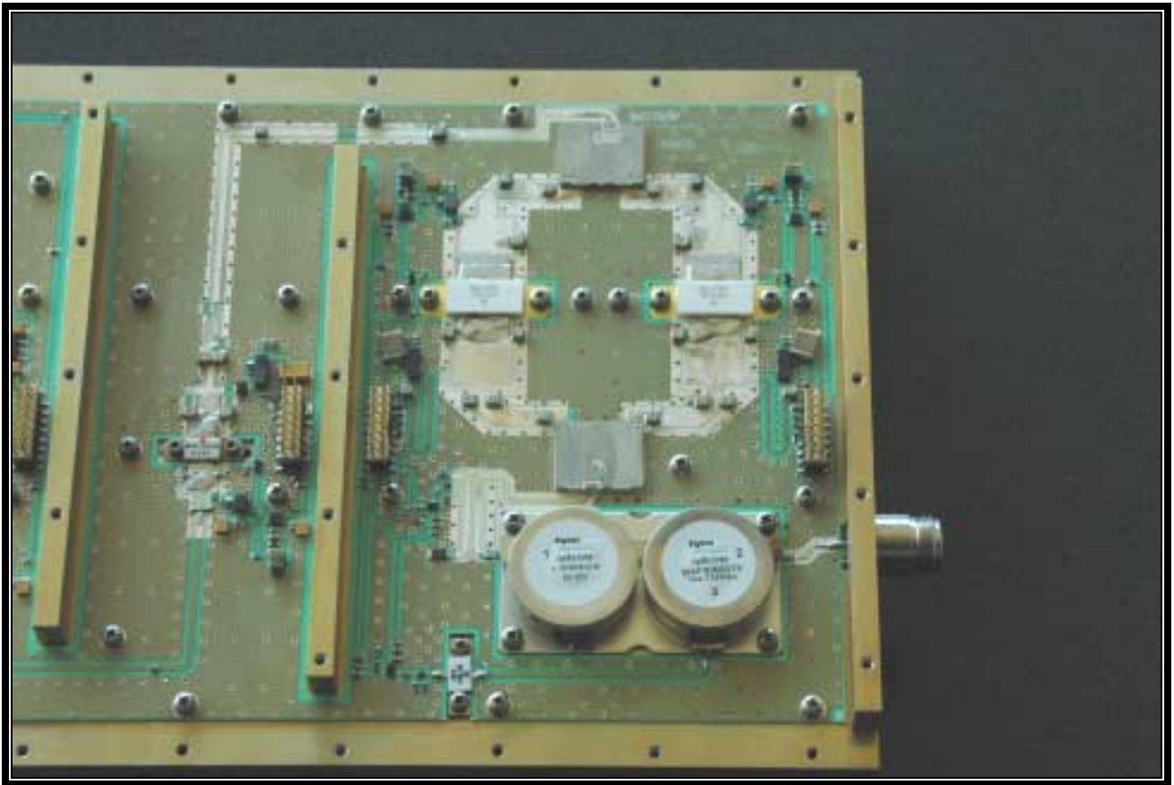
PHOTOGRAPH 22: HPA RF AMP (RIGHT SIDE)
