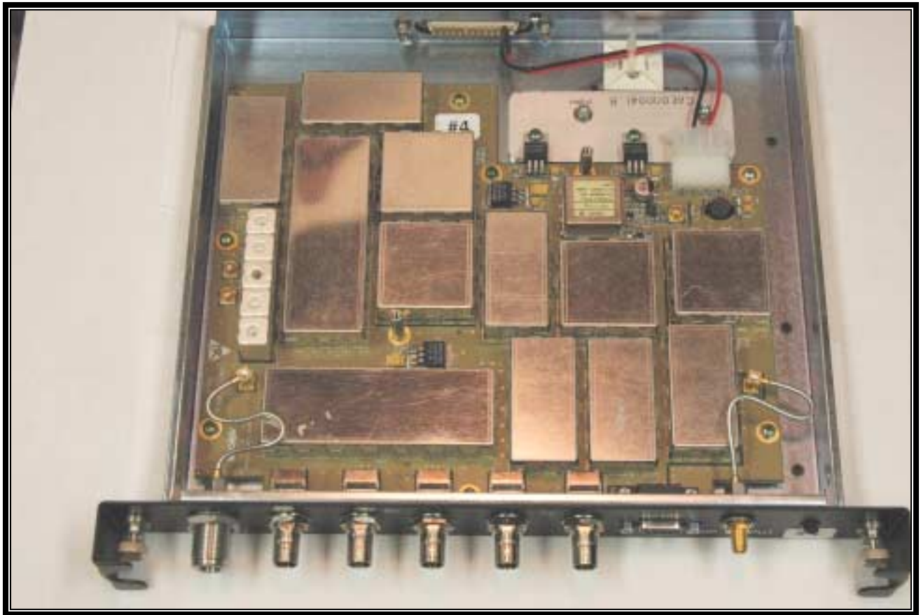
PHOTOGRAPH 26: BSX WITH SHIELDS
