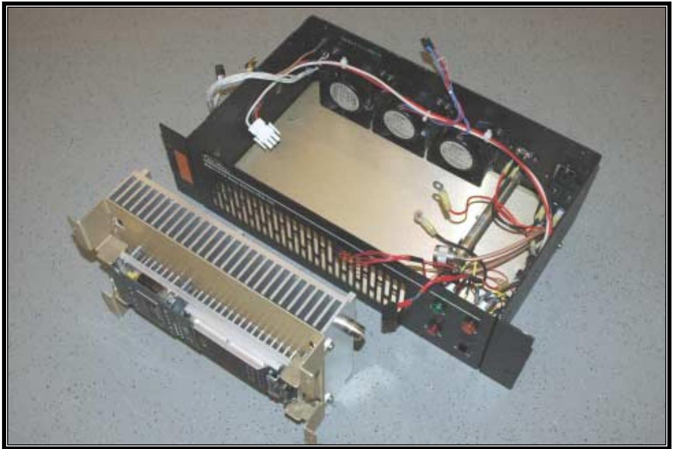
PHOTOGRAPH 16: HPA WITH RF DECK REMOVED
