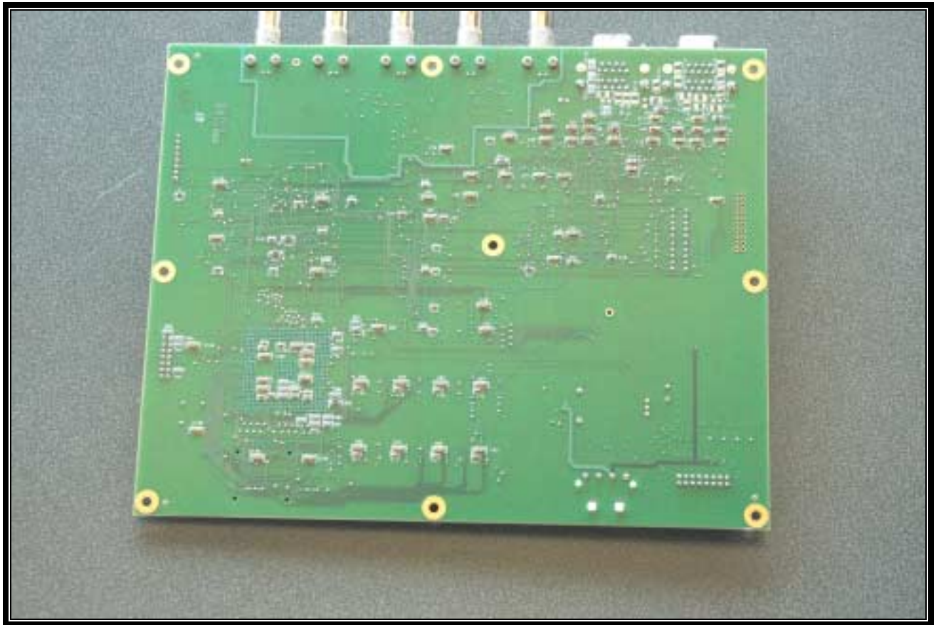
PHOTOGRAPH 25: BSC PCB BOTTOM VIEW
