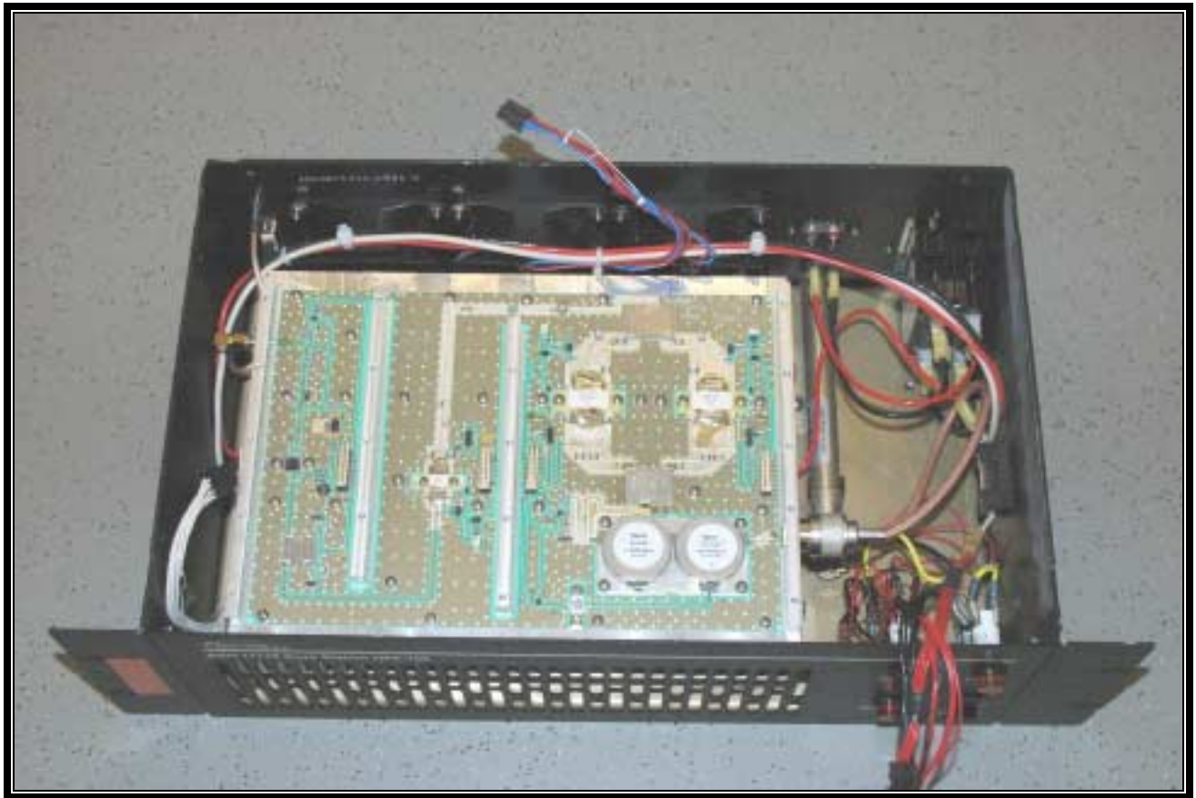
PHOTOGRAPH 15: HPA WIHOUT RF COVER
