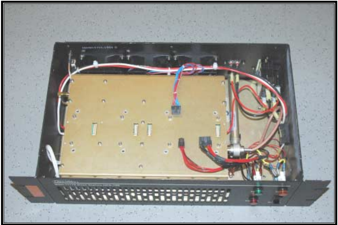
PHOTOGRAPH 14: HPA WITHOUT CONTROLLER
