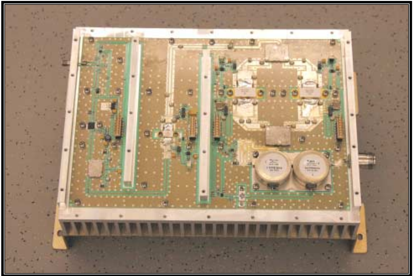
PHOTOGRAPH 18: HPA RF DECK TOP VIEW
