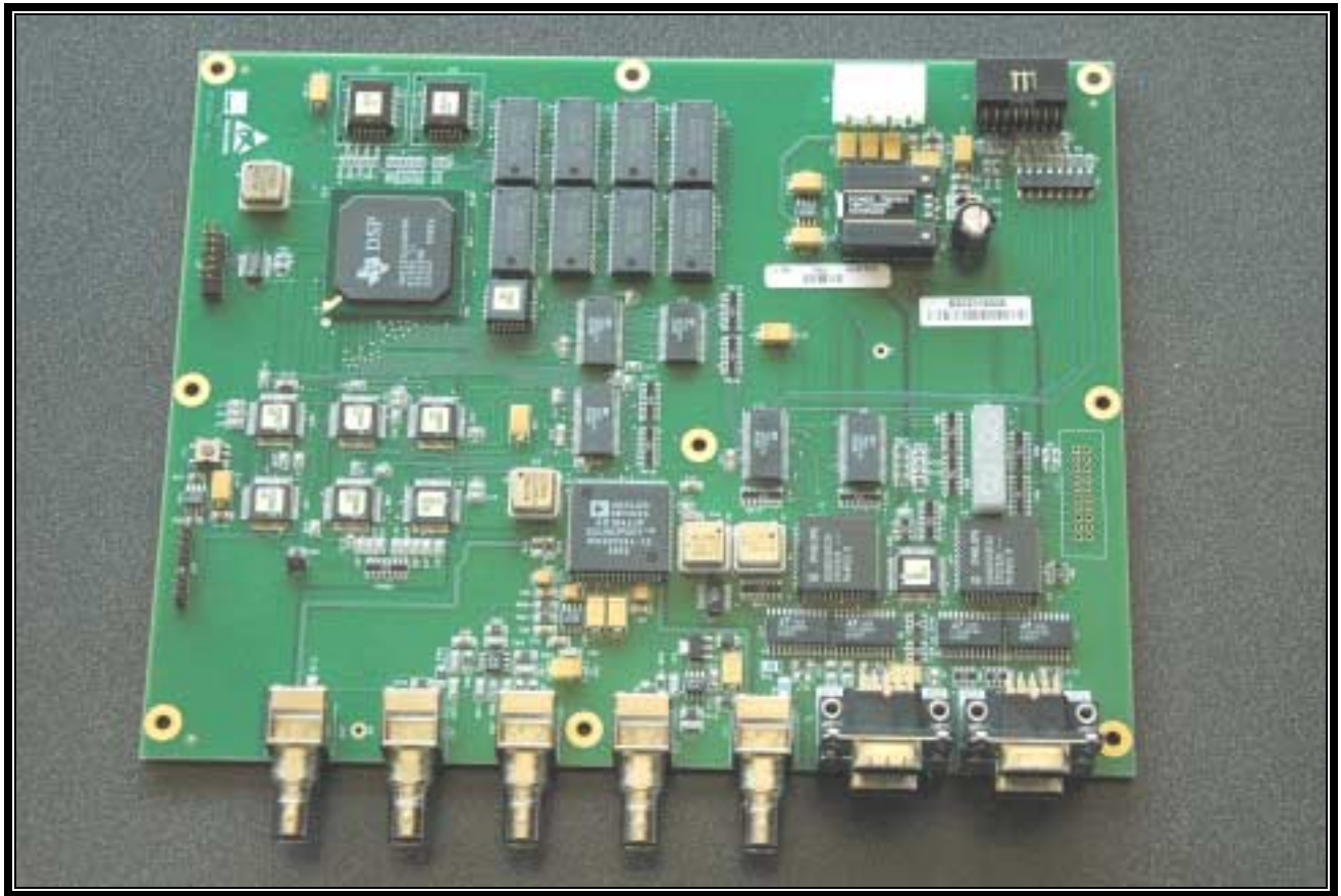
PHOTOGRAPH 24: BSC PCB TOP VIEW
