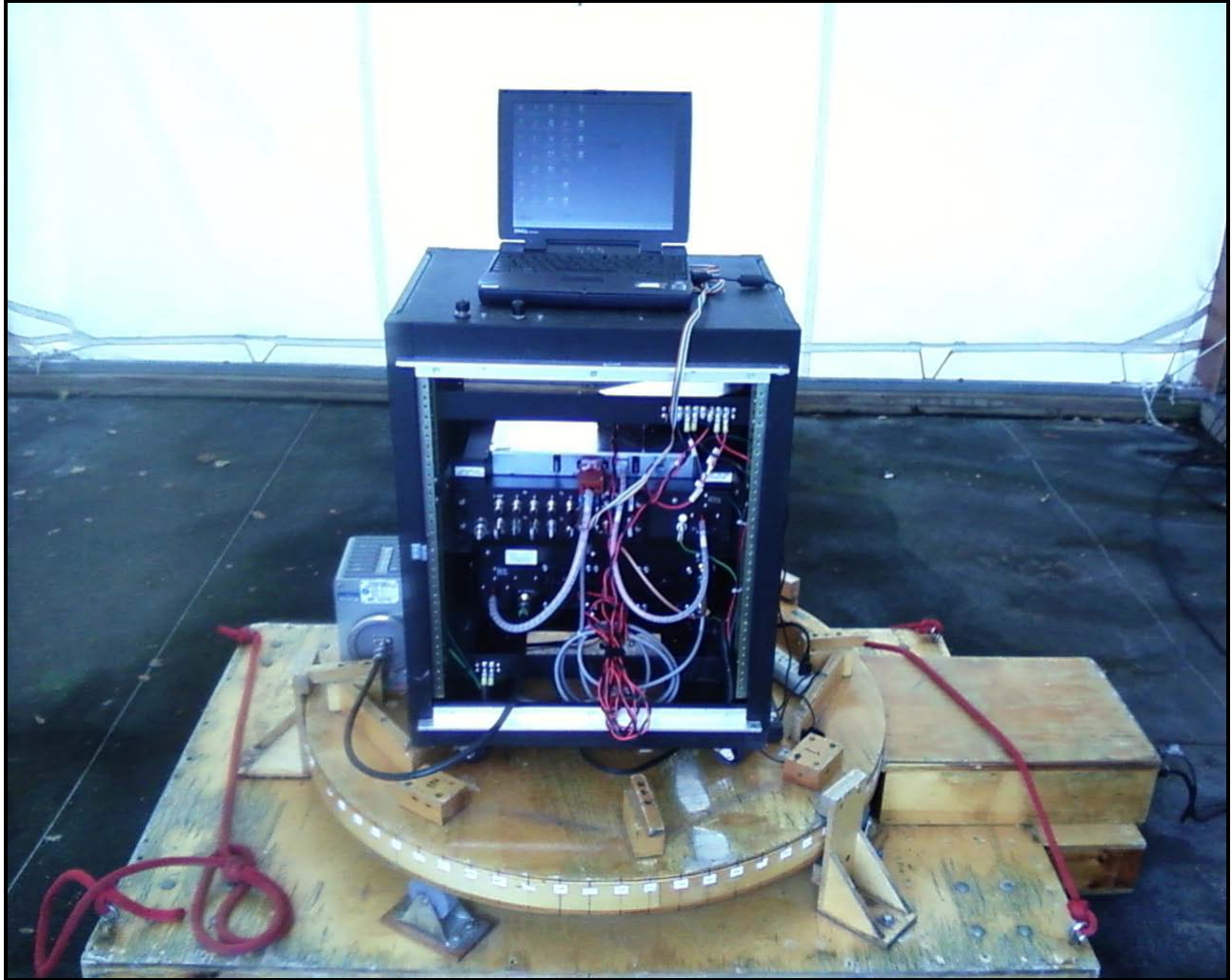
Photograph 2: Radiated Emissions (Rear View)
