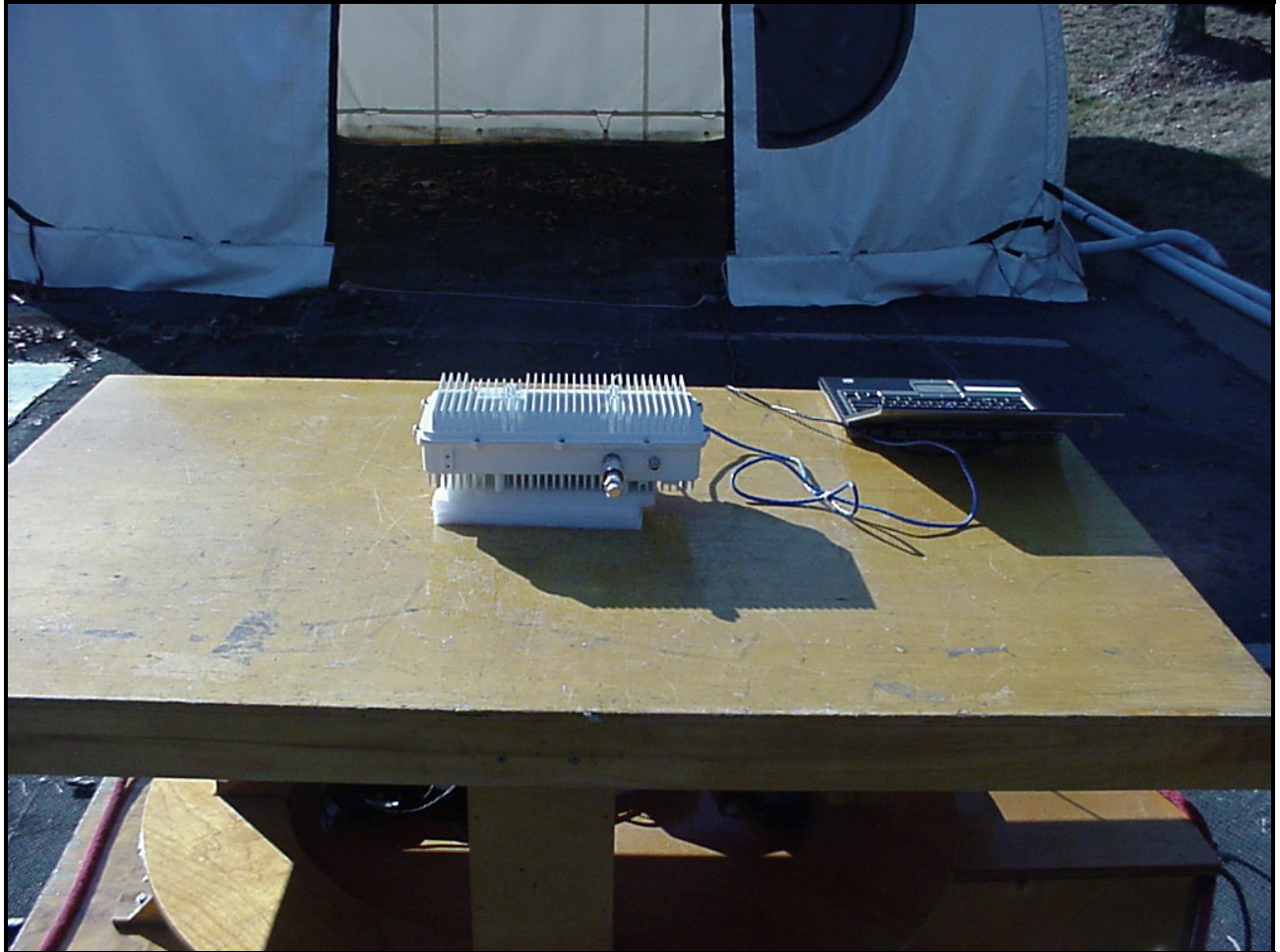
Photograph 3: Radiated Emissions Rear View
