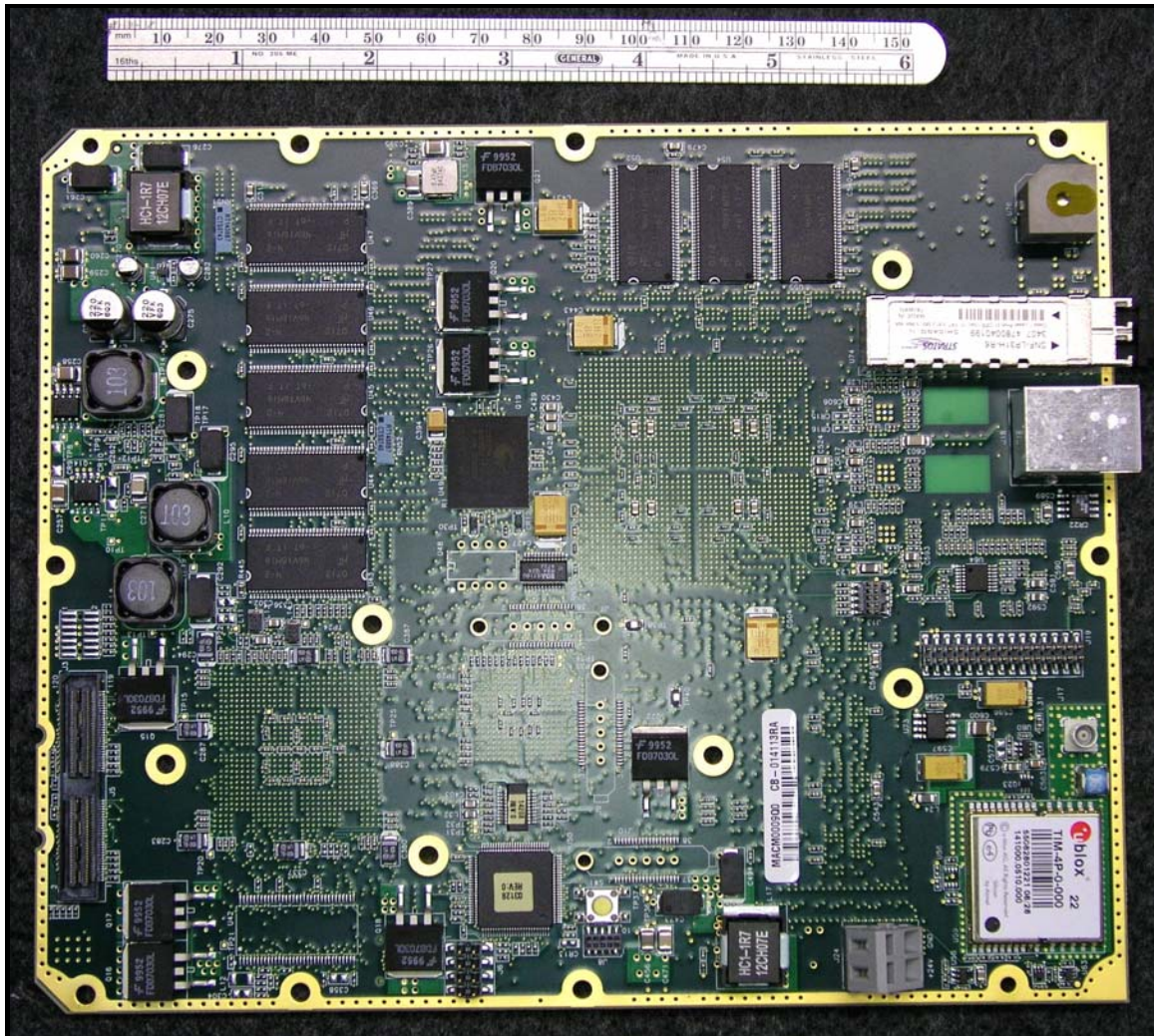
Photograph 11: Digital Board Side 1
