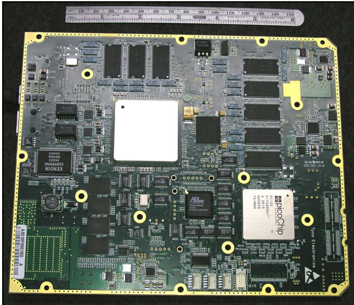
Photograph 12: Digital Board Side 2
