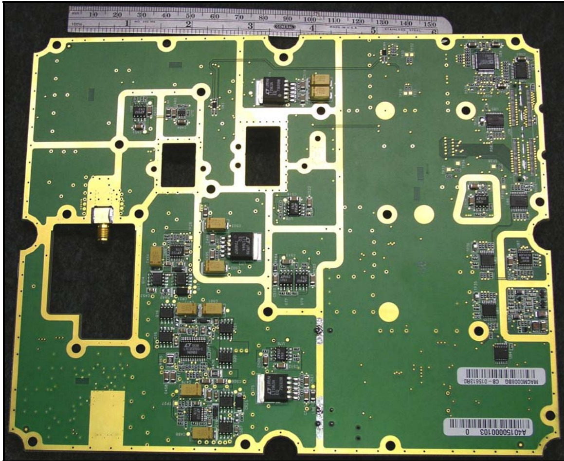
Photograph 10: RF PCB Side 2
