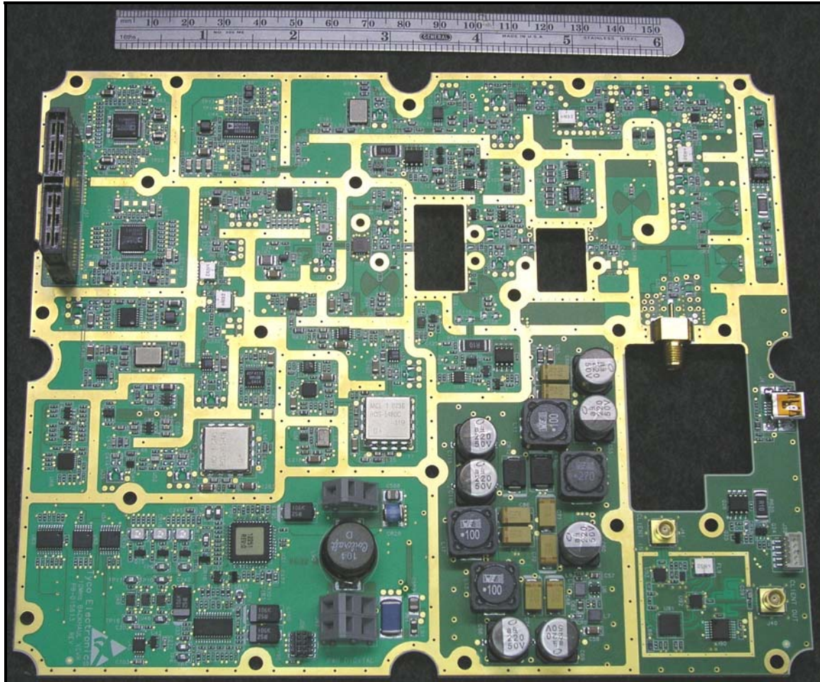
Photograph 9: RF PCB Side 1
