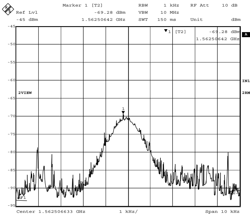
Figure 8-2: UWB radiated emissions within GPS band, SHORT PULSE mode; RBW=1kHz
