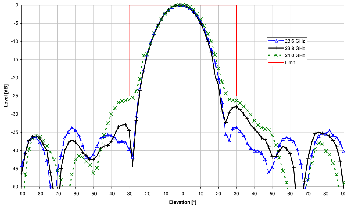
Figure 7-1: Transmit elevation pattern taken from SN 030002112. Limit lines for compliance until 2010-01-01.
