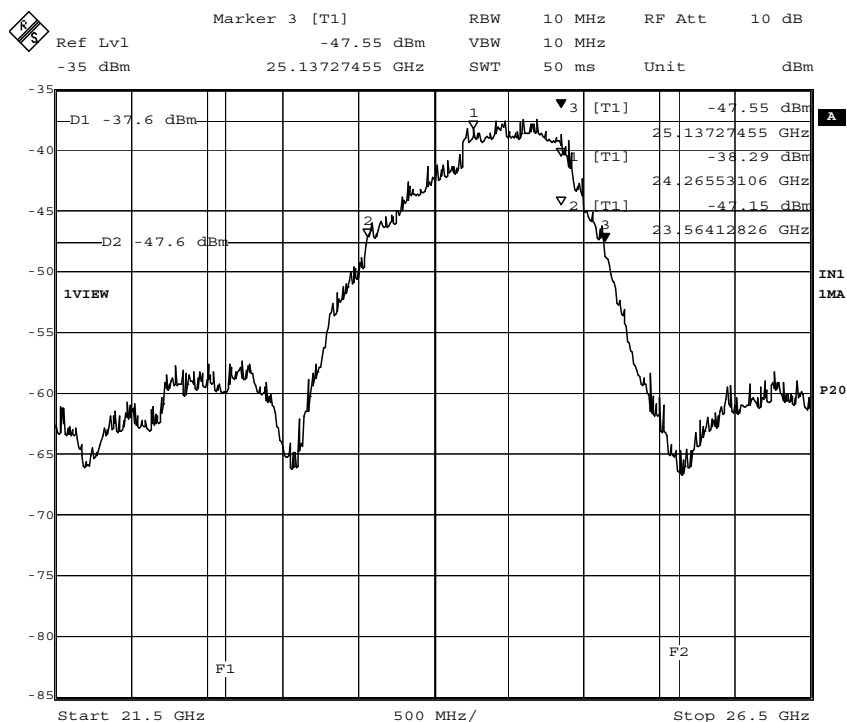
Figure 6-2: Occupied Bandwidth, SHORT PULSE mode
