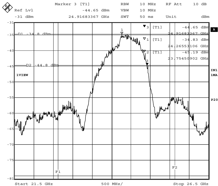
Figure 6-1: Occupied Bandwidth, LONG PULSE mode
