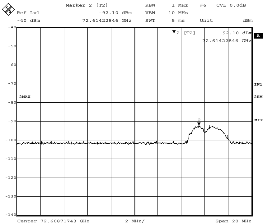
Figure 8-8: UWB radiated emissions, CW mode with RF switch set to its high insertion loss state; RMS reading
