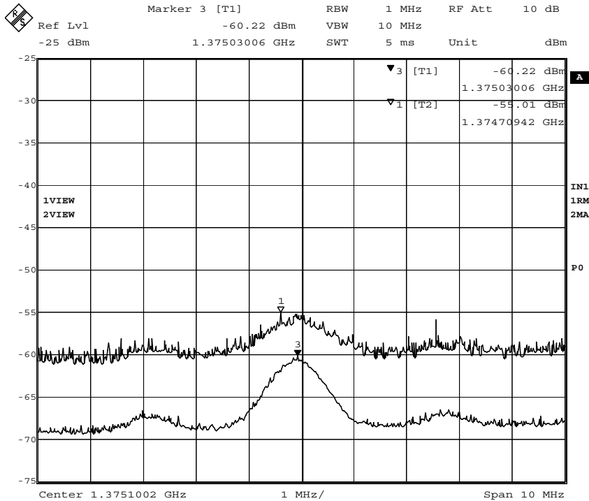
Figure 8-1: UWB radiated emissions, SHORT PULSE mode; RMS and PEAK reading
