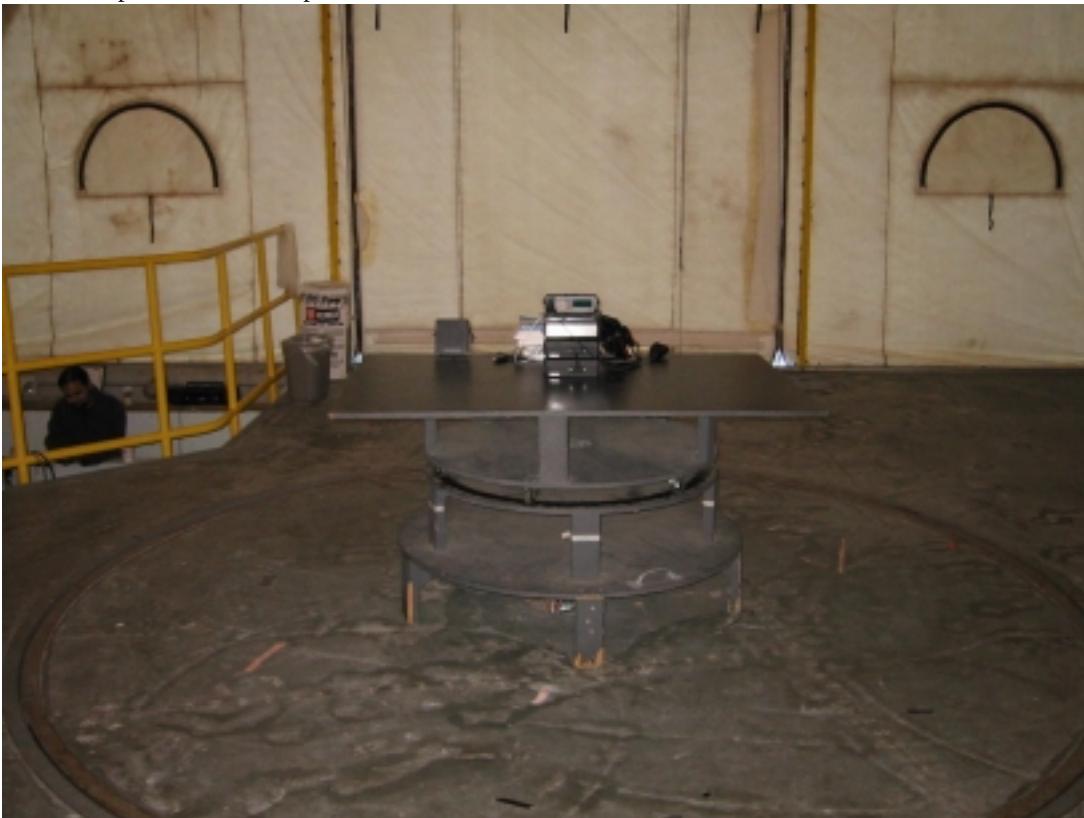
Radiated Spurious Test Setup, Front
