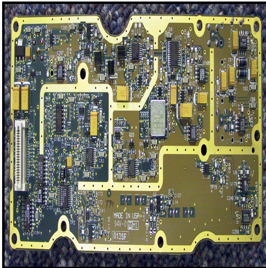
Fi Figure 4 VRB Bottom View #2
