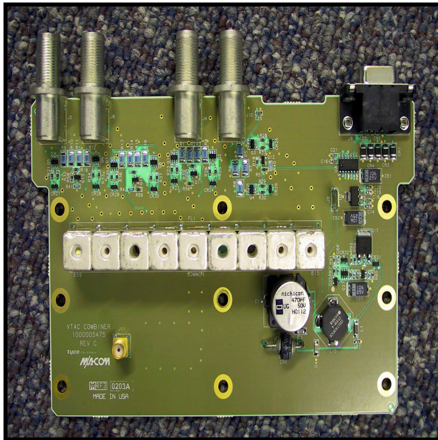
Figure 2 RFC Top View #2
