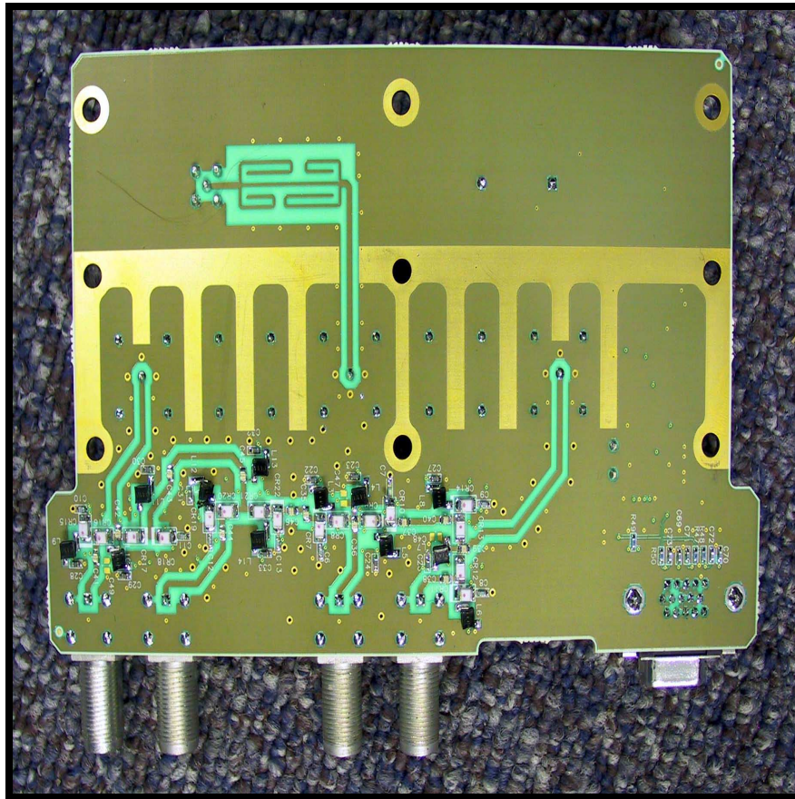
Figure 3 RFC Bottom View
