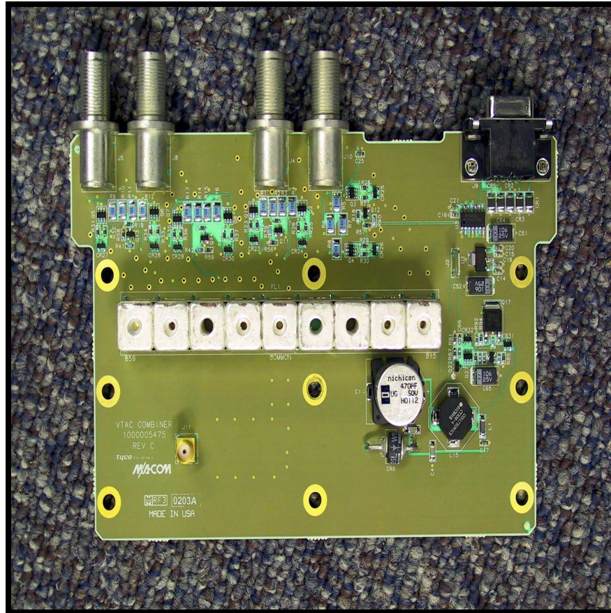
Figure 1 RFC Top View#1
