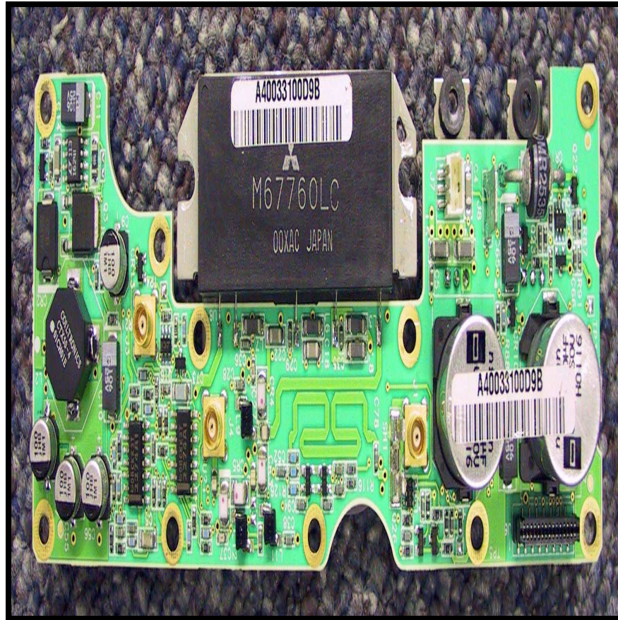
Figure 1 HPA Top View#1
