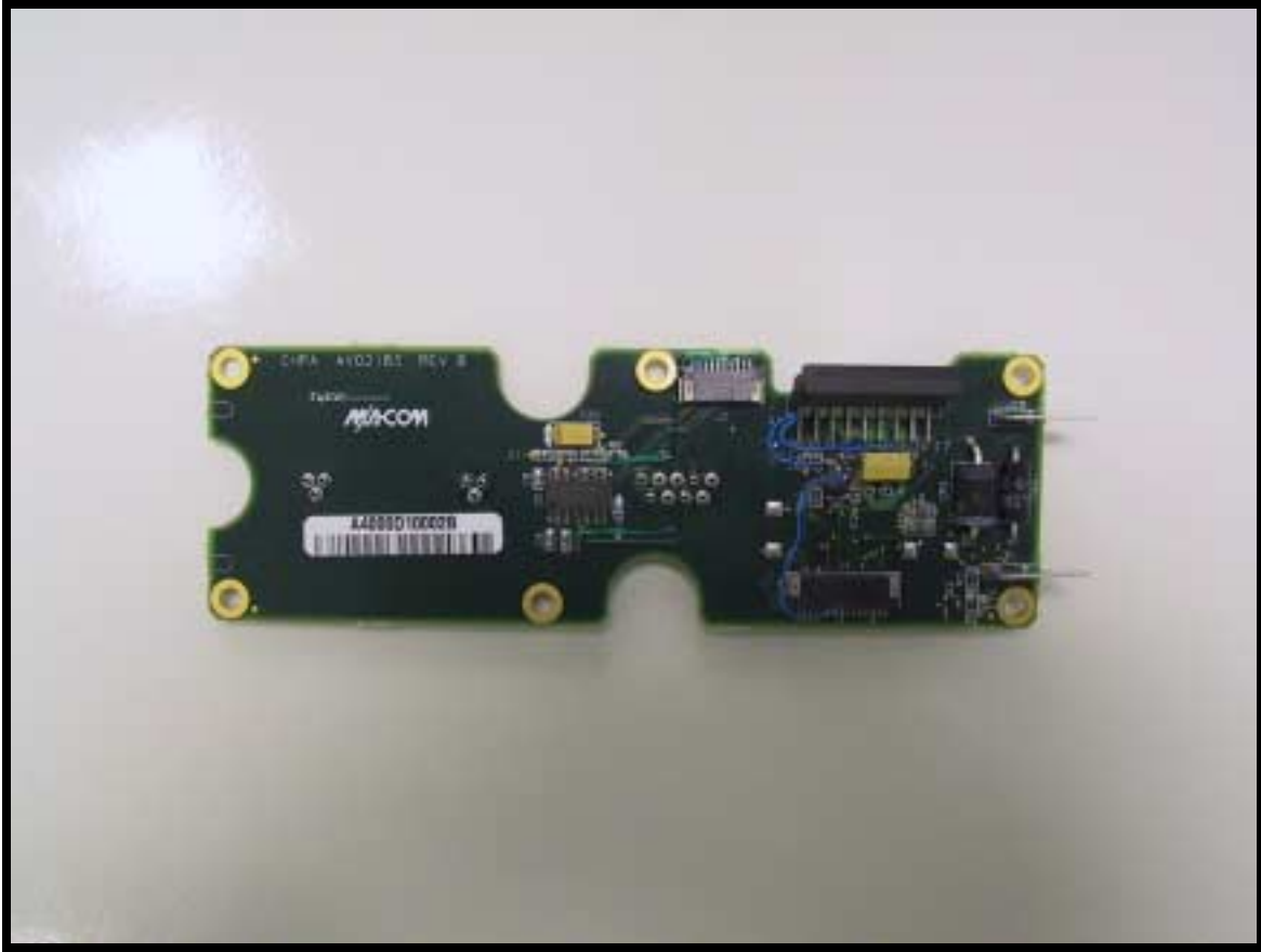
Figure 11 Display Board Top View
