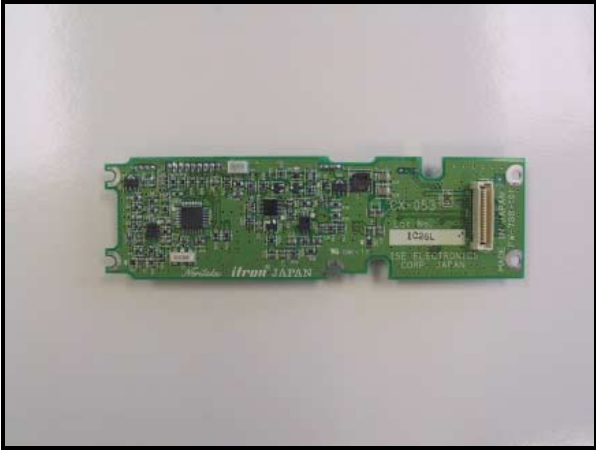
Figure 10 Display Board Bottom View
