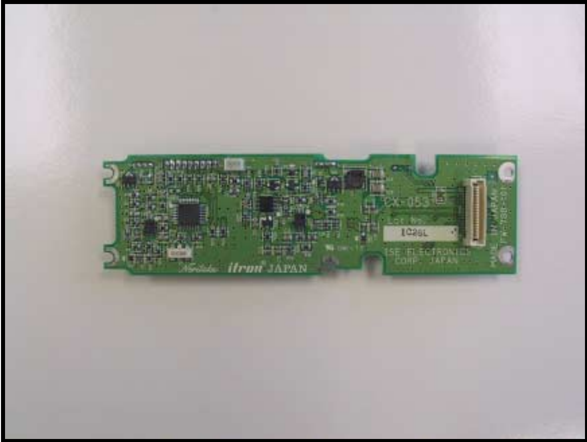
Figure 18 Display Board Bottom View
