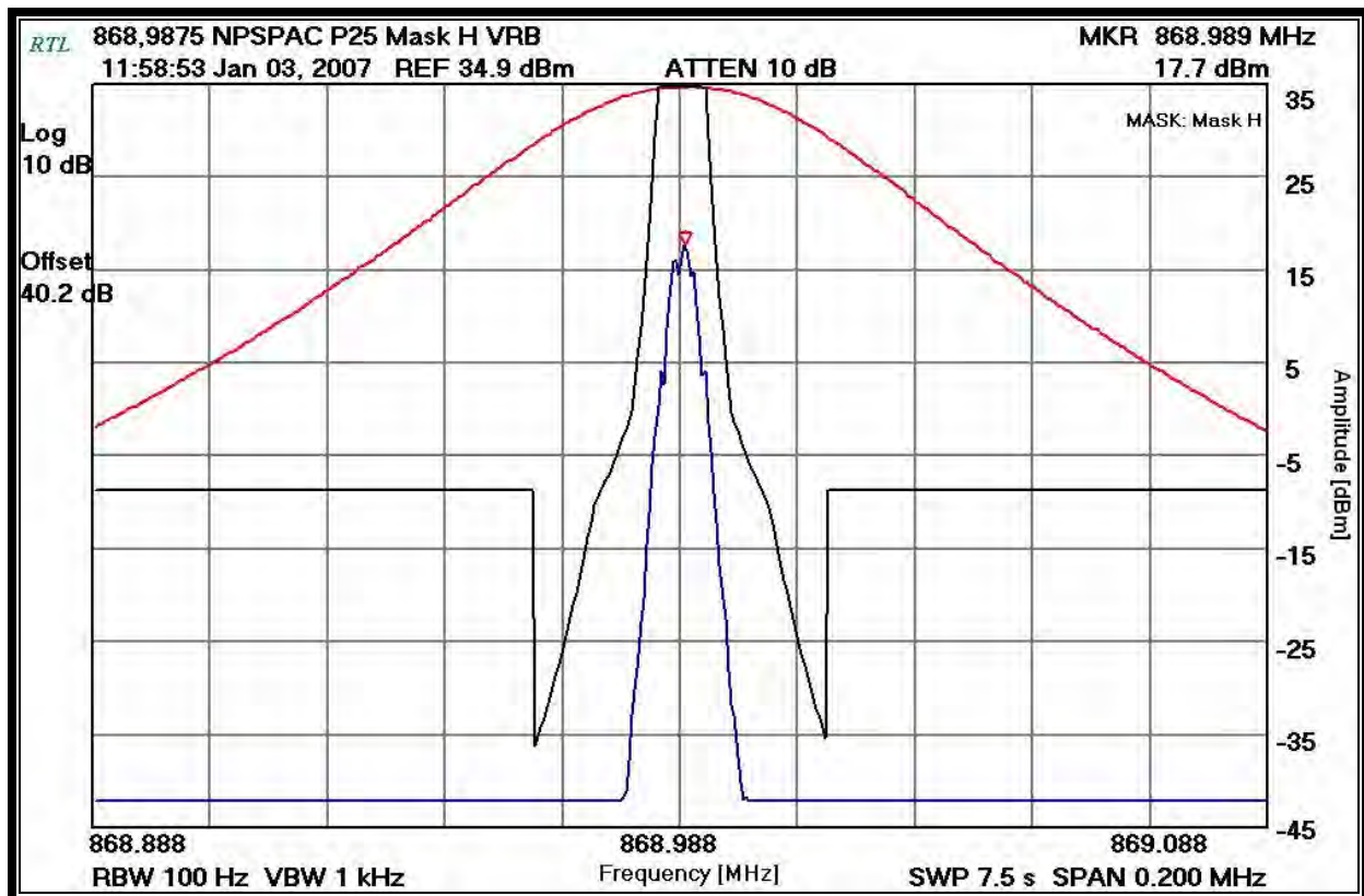
Plot 8-20: Emissions Masks – VRB – NPSPAC; P25; 868.9875 MHz
