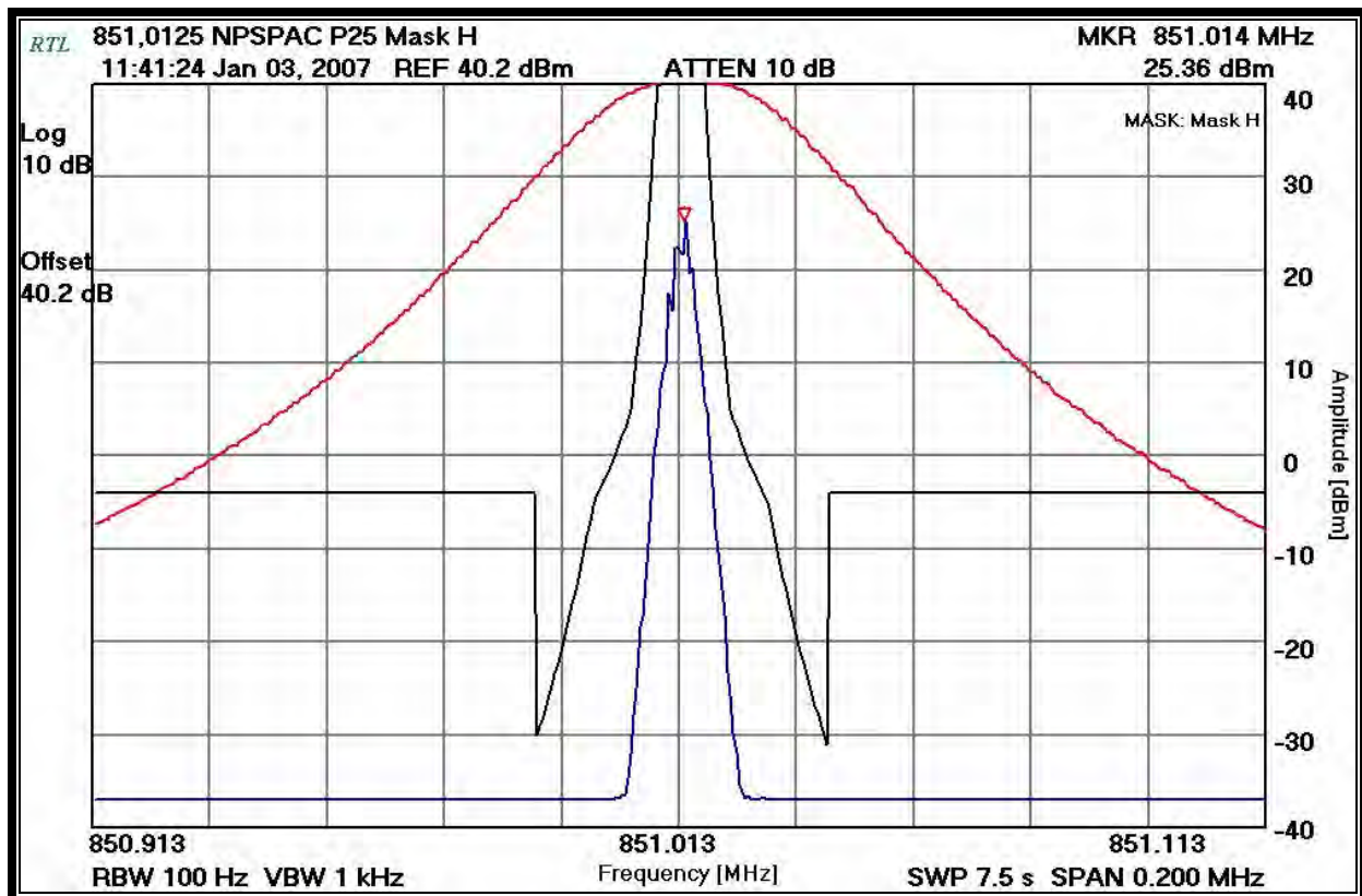
Plot 8-14: Emissions Masks – VRM – NPSPAC; P25; 851.0125 MHz
