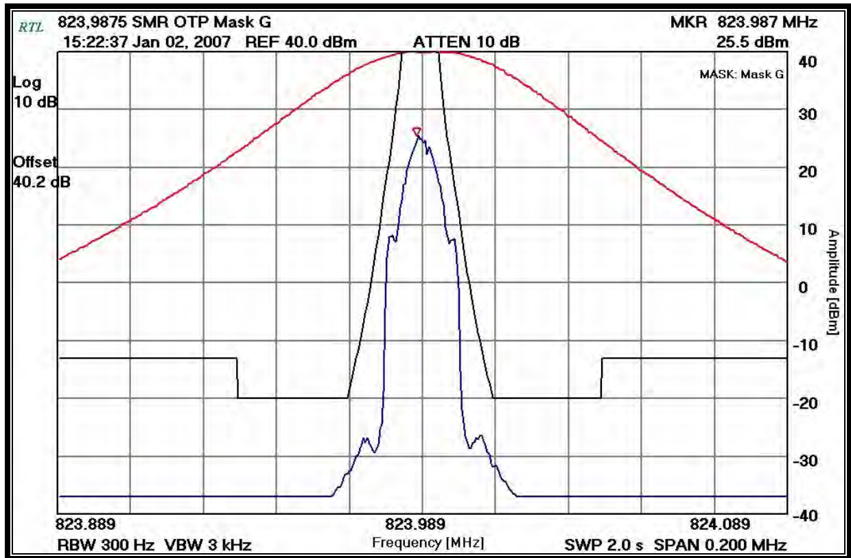
Plot 8-23: Emissions Masks – VRM – SMR; OTP; 823.9875 MHz
