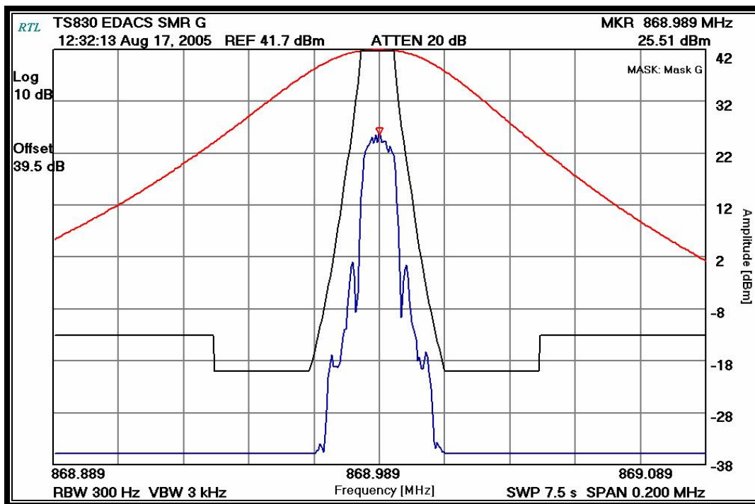
PLOT 9-28: OCCUPIED BANDWIDTH – 868.9875 MHz; EDACS; SMR; (MASK G)
