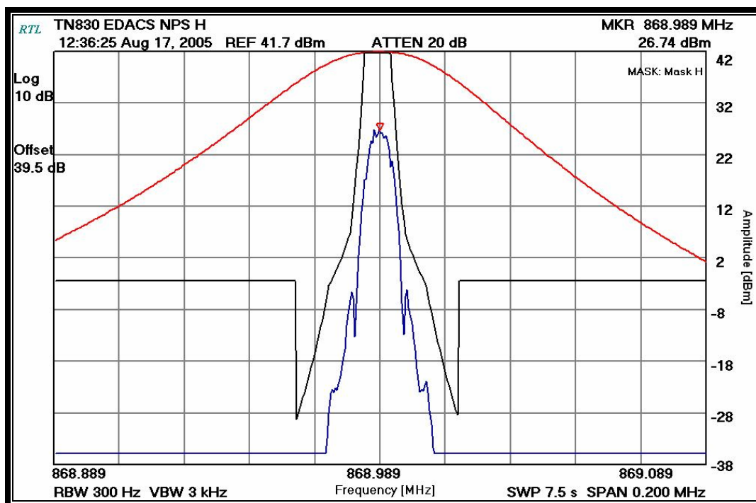
PLOT 9-27: OCCUPIED BANDWIDTH – 868.9875 MHz; EDACS; NPSPAC; (MASK H)
