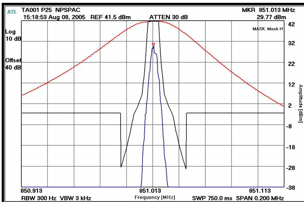
PLOT 9-21: OCCUPIED BANDWIDTH – 851.0125 MHz; P25 TALKAROUND; NPSPAC; (MASK H)
