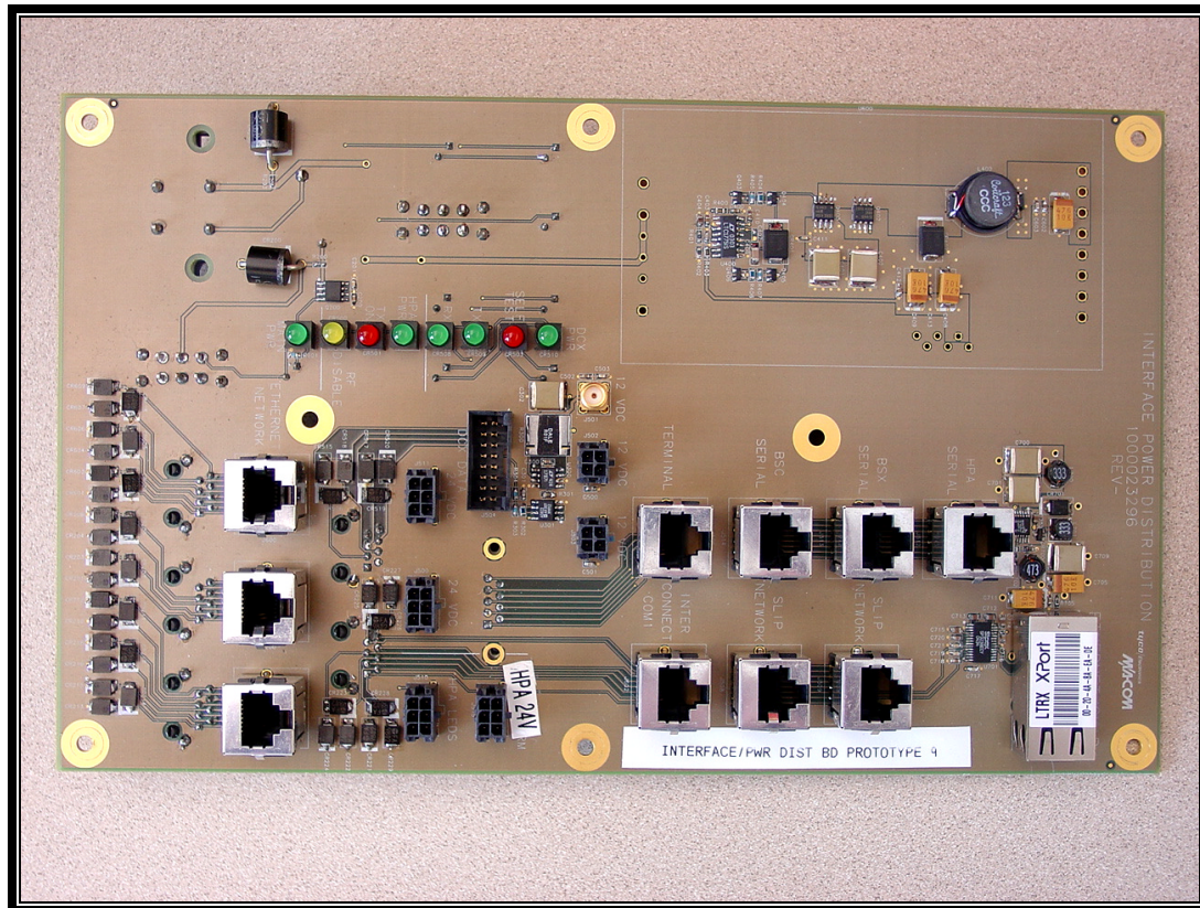
Photograph 29: Interface Board Back
