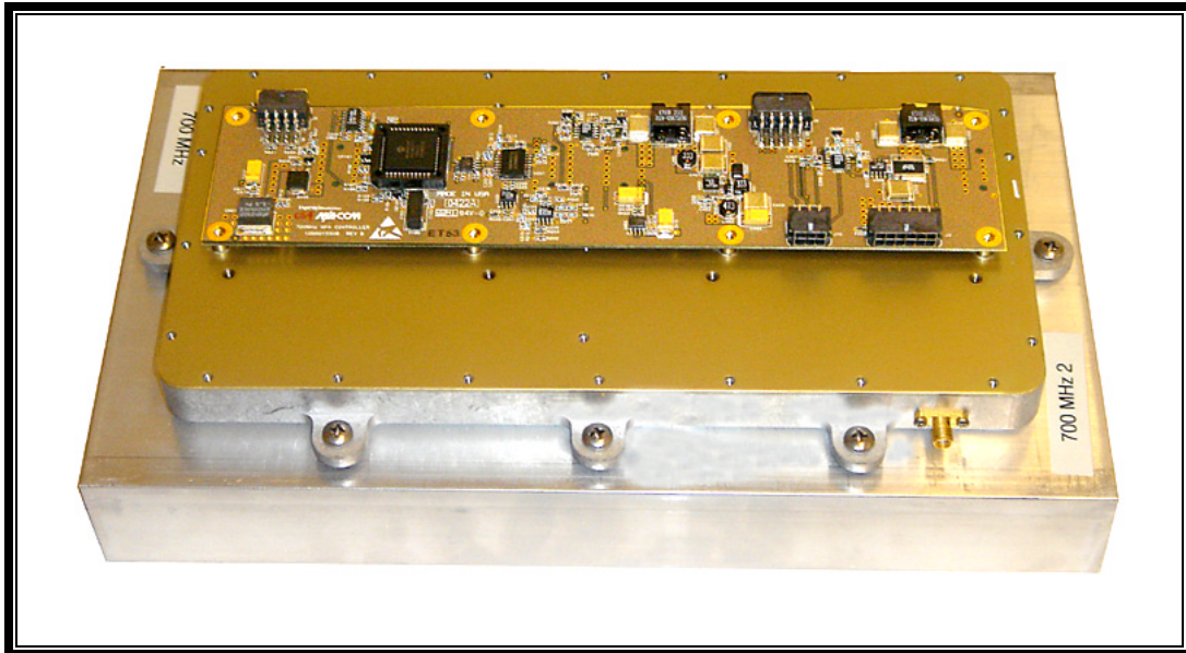
Photograph 16: 700 MHz Cell Site HPA Assembly – Control Board Cover
