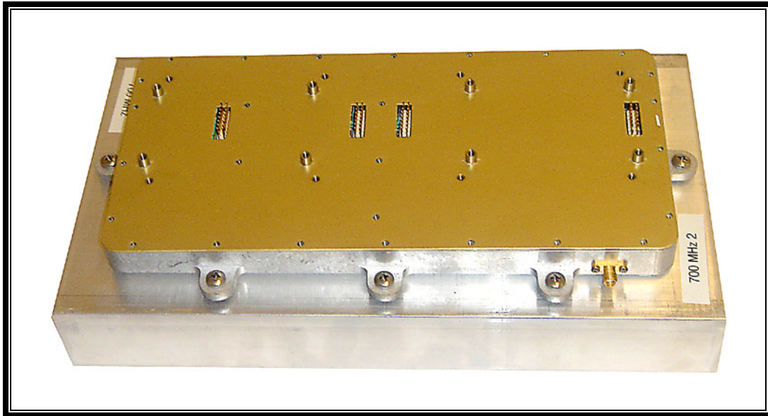
Photograph 17: 700 MHz Cell Site HPA RF Assembly
