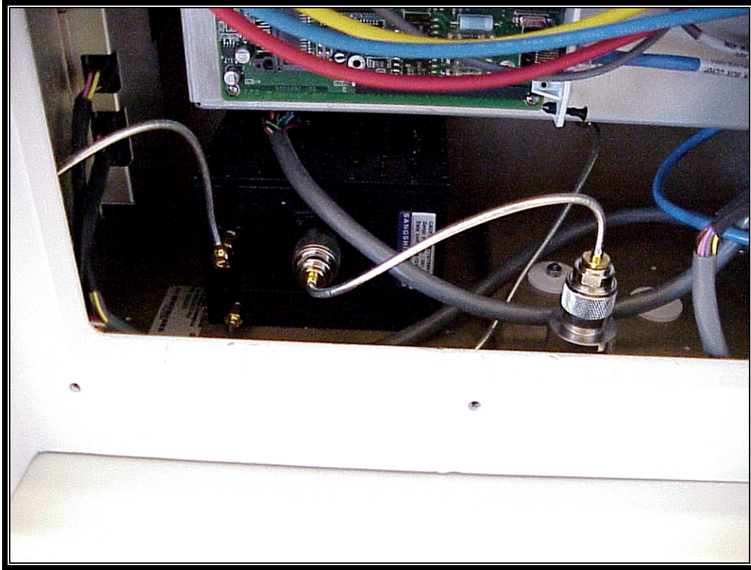
Photograph 14: 700 MHz Cell Site Enclosure with Duplexer
