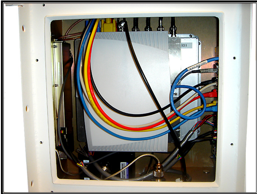
Photograph 10: 700 MHz Cell Site Straight On
