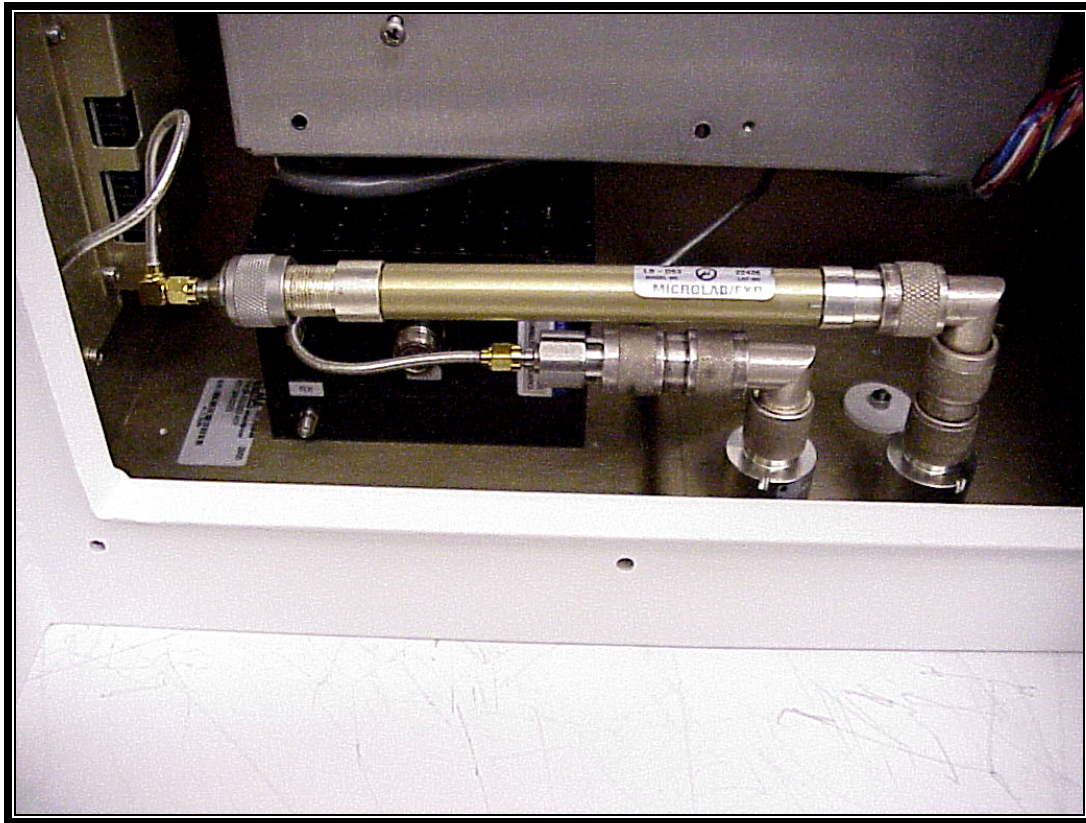
Photograph 13: 700 MHz Cell Site Interior with Filter
