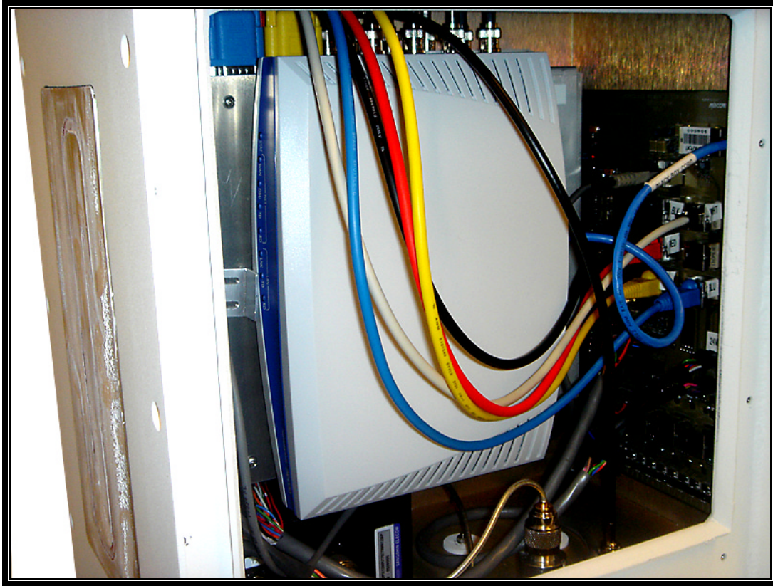
Photograph 11: 700 MHz Cell Site Interior Front
