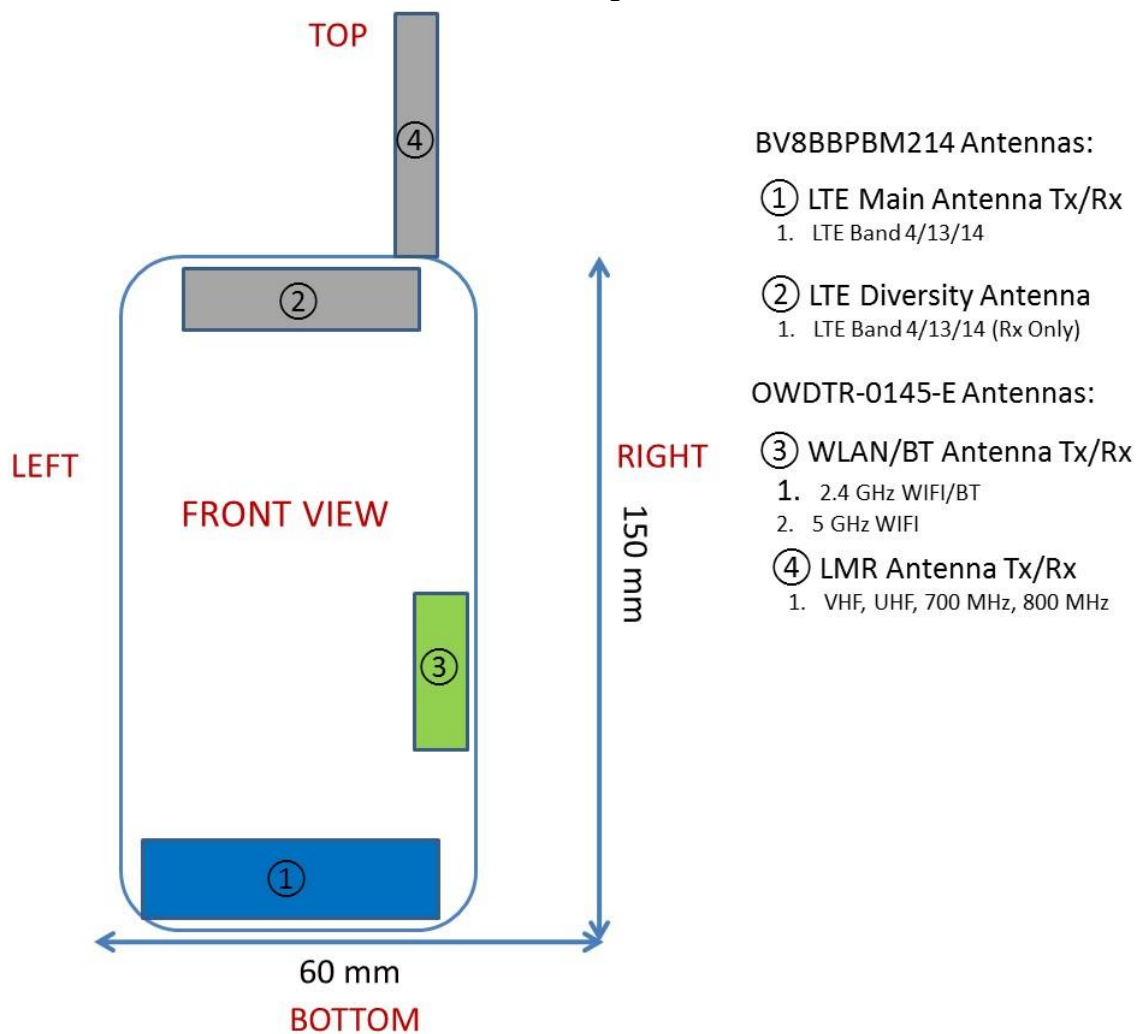
Figure F-1 DUT Antenna Locations
