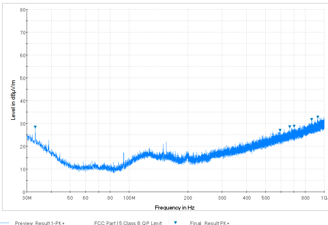
Plot 7-47. Radiated Spurious Plot from 30MHz - 1GHz (Whip Antenna: 14035-4440-01) (Pol. V)
