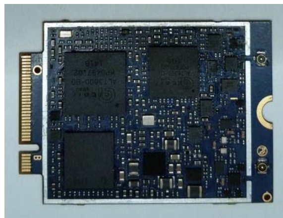
Module topside without frame
