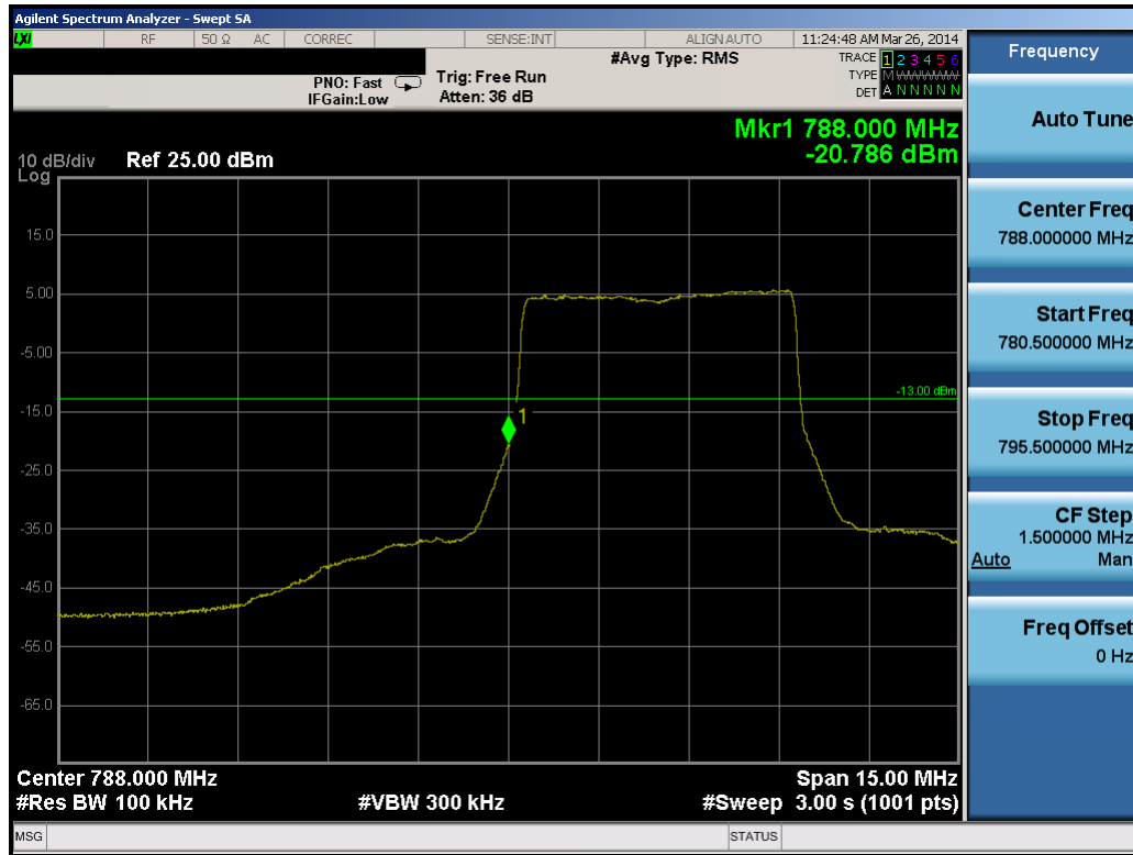
Plot 7-2. Lower Band Edge Plot (16QAM, 25RB)
