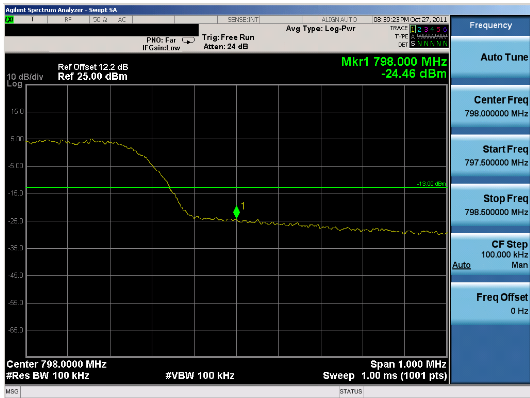
Plot 7-4. Upper Band Edge Plot (QPSK, 25RB)
