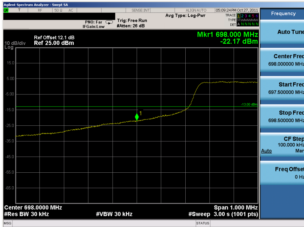
Plot 8-2. Lower Band Edge Plot (QPSK, 25RB)
