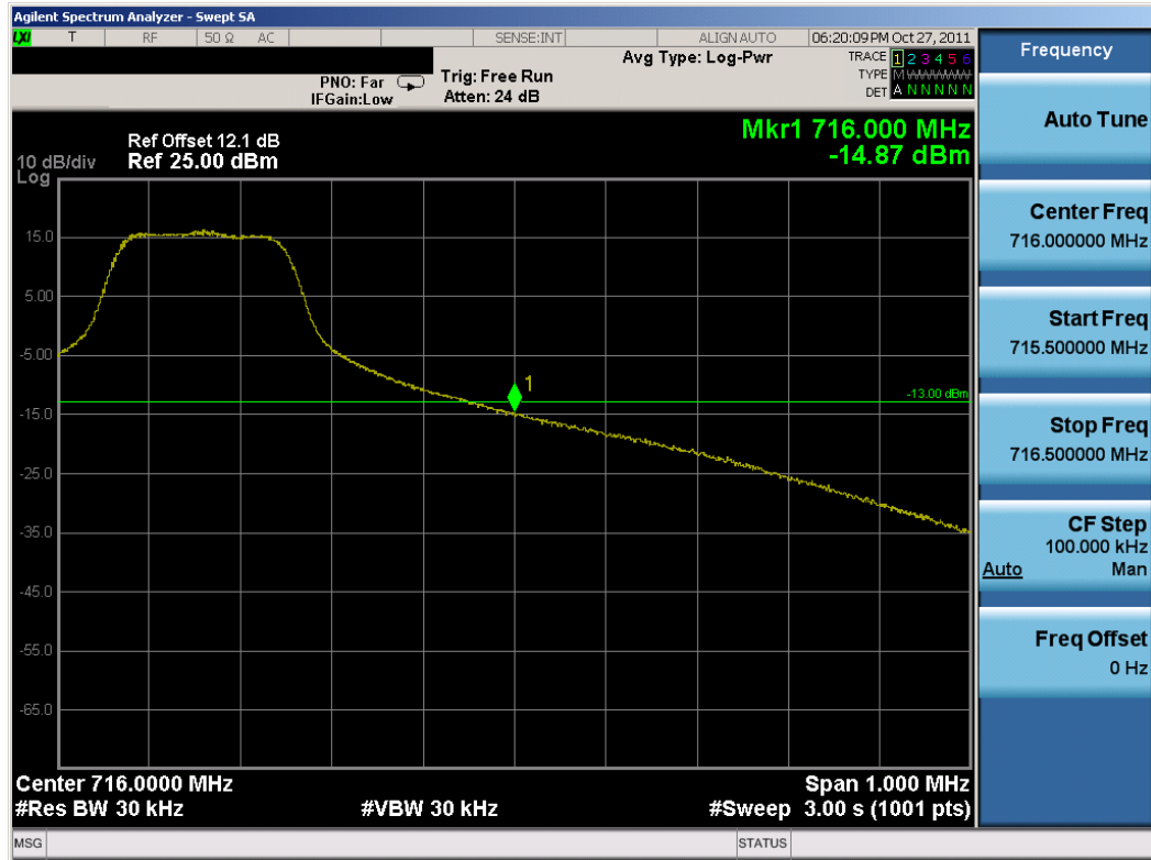
Plot 8-5. Upper Band Edge Plot (QPSK, 1RB, Offset 24)
