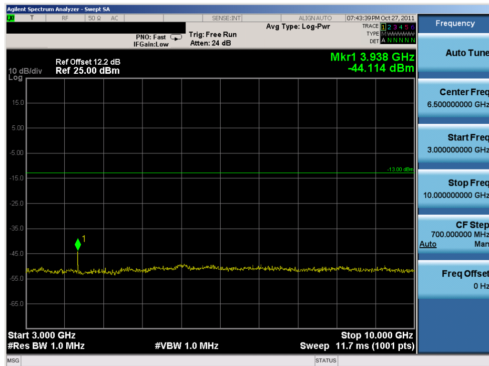
Plot 9-12. Conducted Spurious Plot (790.5 MHz)
