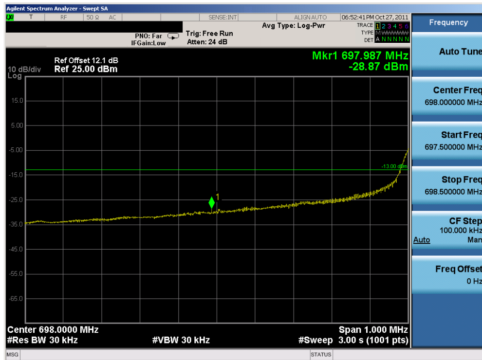
Plot 7-2. Lower Band Edge Plot (QPSK, 50RB)
