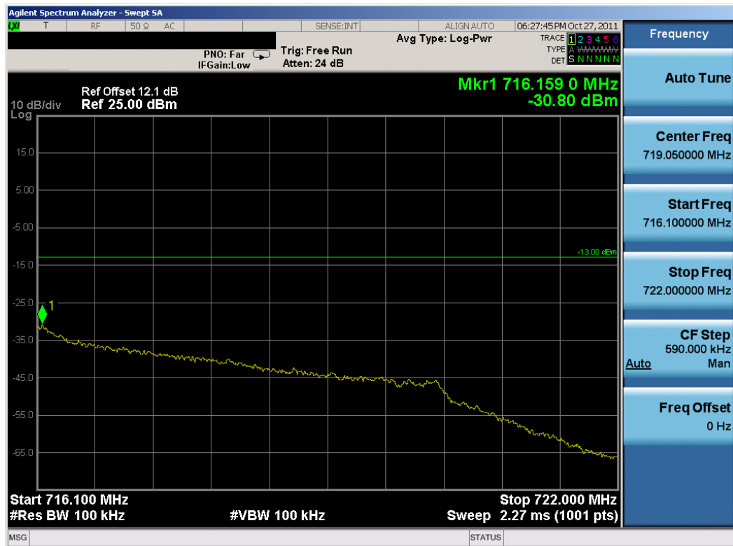
Plot 8-8. Upper Extended Band Edge Plot (QPSK, 25RB)
