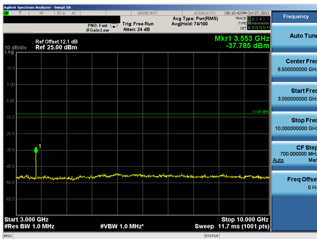
Plot 8-16. Conducted Spurious Plot (High Channel)
