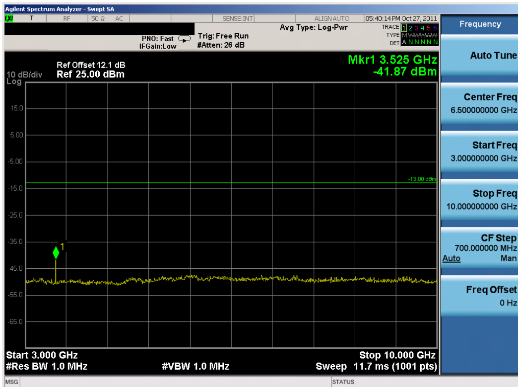
Plot 8-14. Conducted Spurious Plot (Mid Channel)
