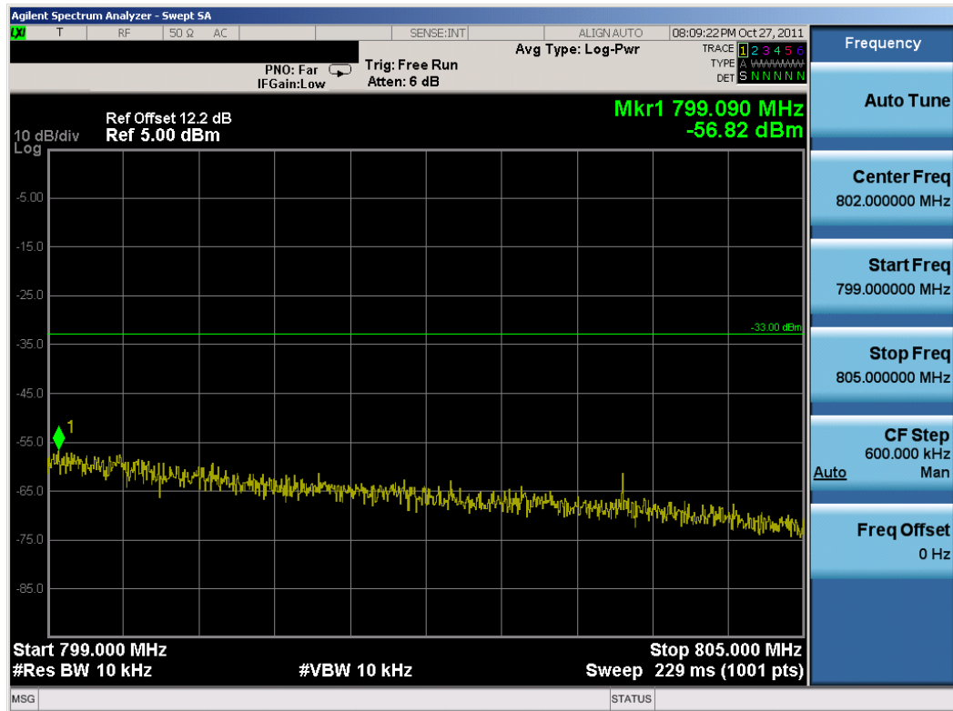
Plot 9-4. Upper Emission Mask 799-805 MHz Plot (QPSK, 25RB)
