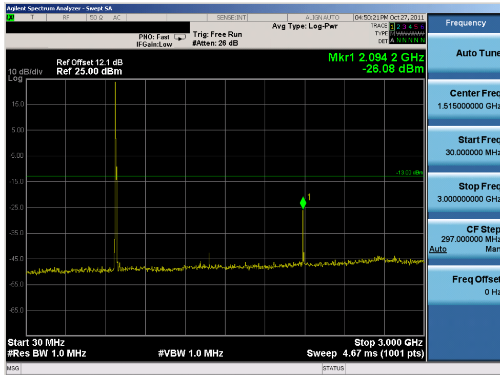
Plot 8-11. Conducted Spurious Plot (Low Channel)
