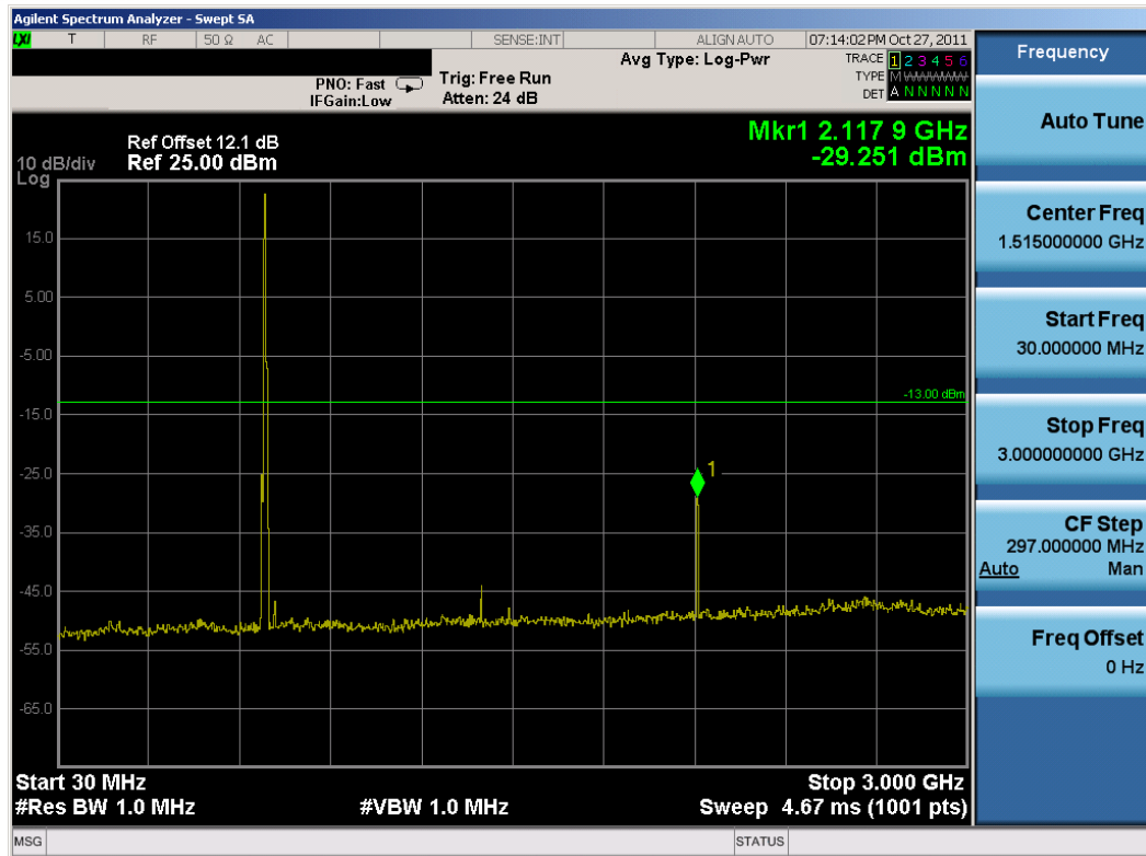
Plot 7-15. Conducted Spurious Plot (High Channel)
