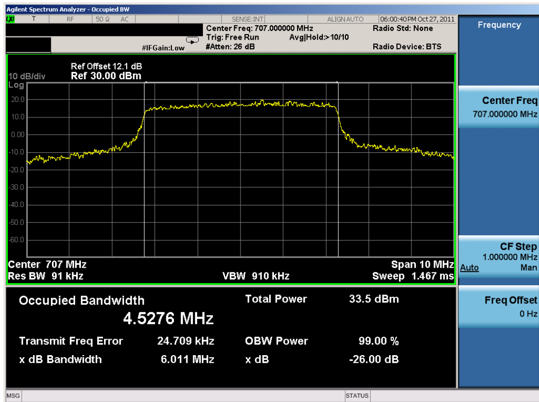
Plot 8-10. Occupied Bandwidth Plot (16-QAM, 25RB)
