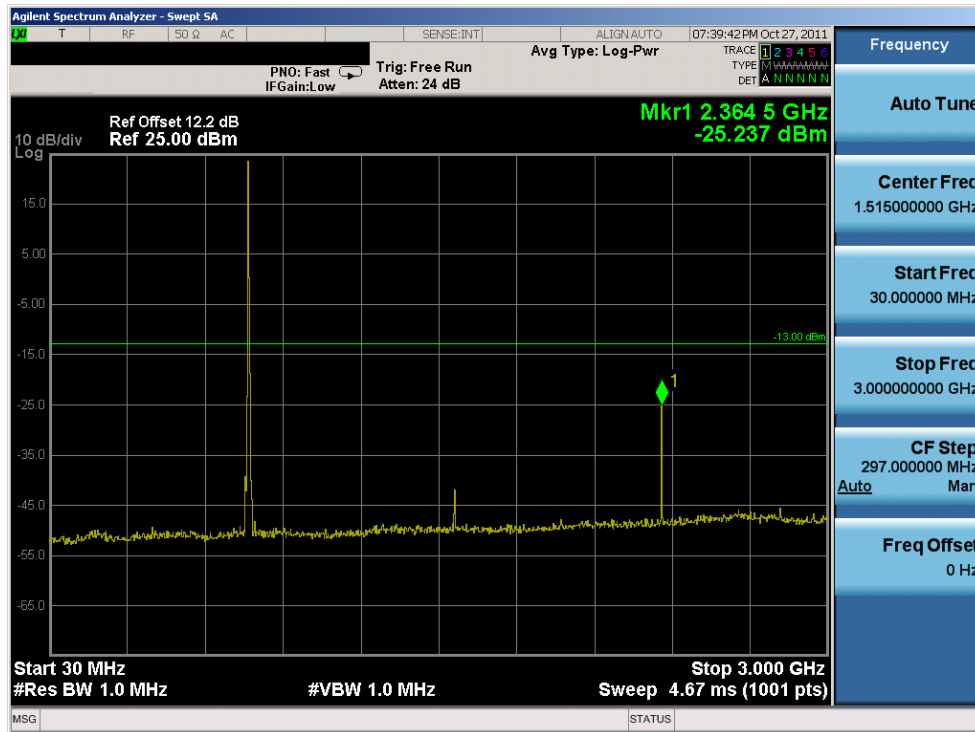
Plot 9-11. Conducted Spurious Plot (790.5MHz)
