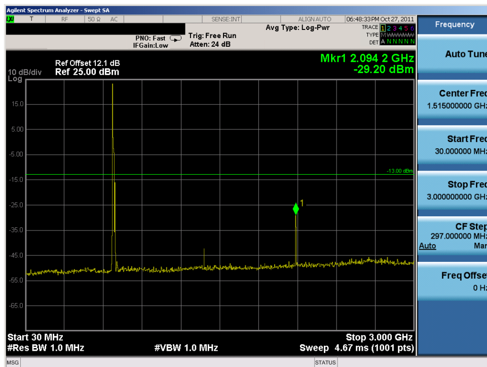
Plot 7-11. Conducted Spurious Plot (Low Channel)
