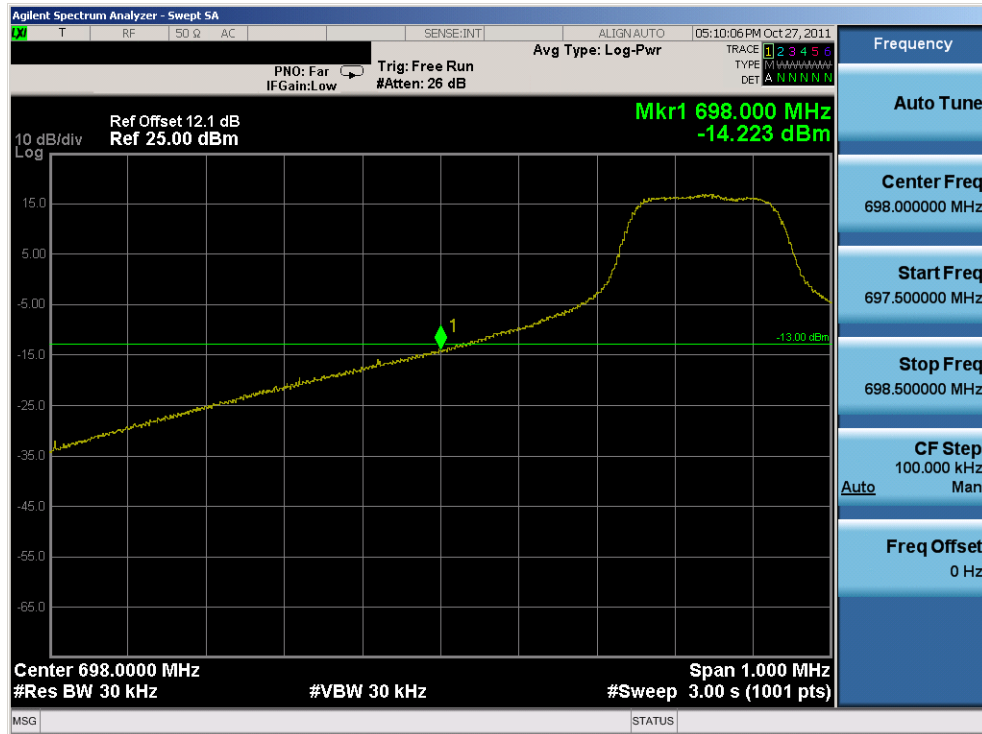
Plot 8-1. Lower Band Edge Plot (QPSK, 1RB, Offset 0)
