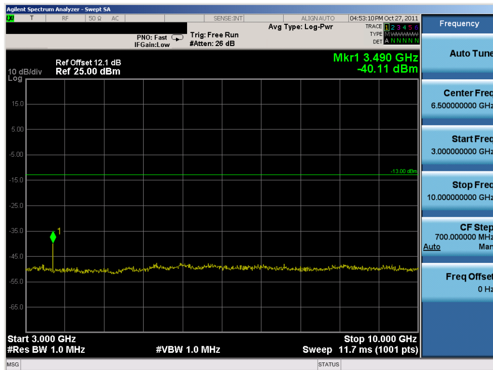
Plot 8-12. Conducted Spurious Plot (Low Channel)
