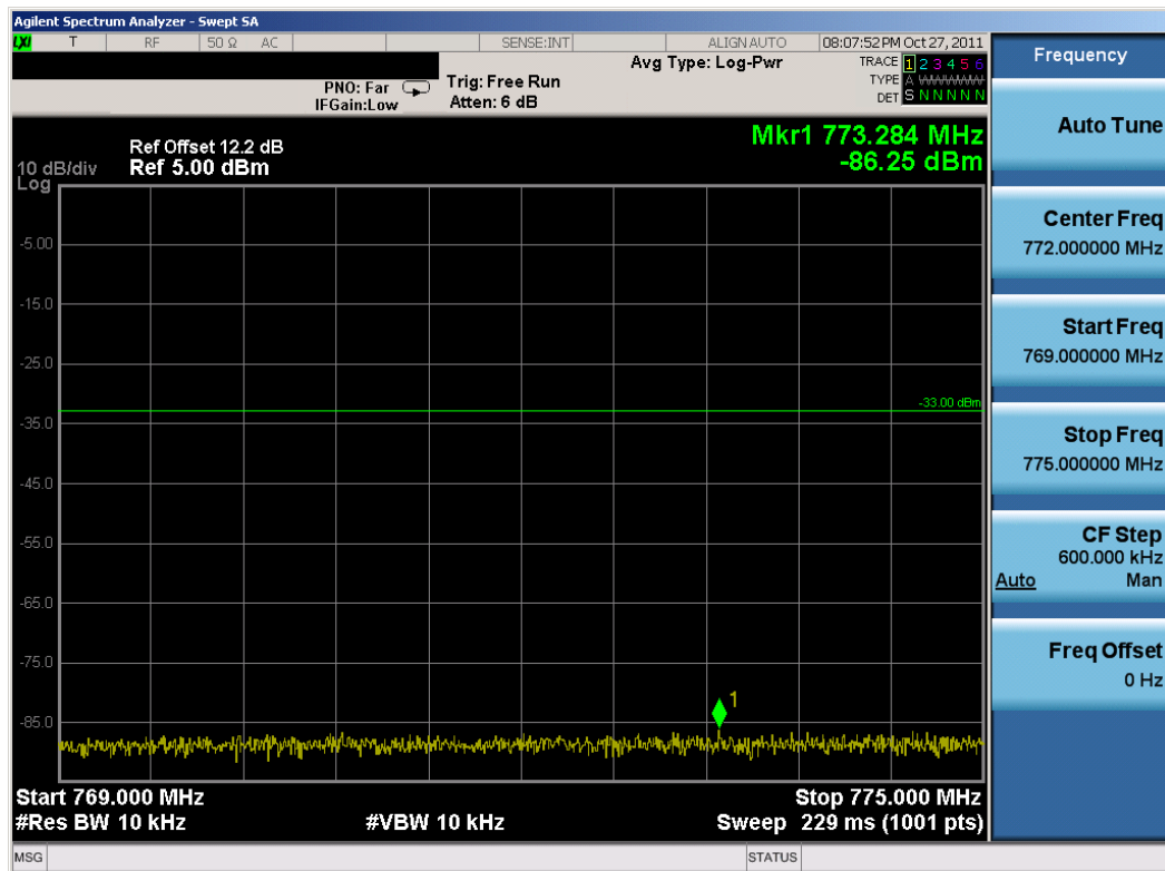
Plot 9-1. Lower Emission Mask 769-775MHz Plot (QPSK, 1RB, Offset 0)
