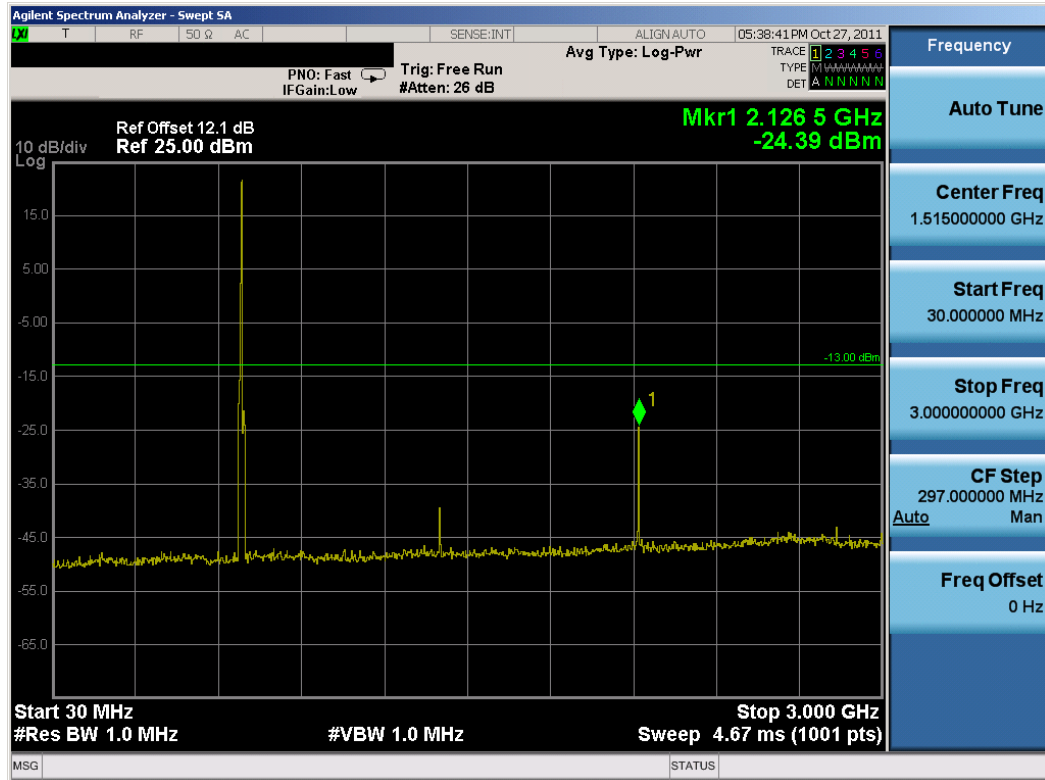
Plot 8-13. Conducted Spurious Plot (Mid Channel)
