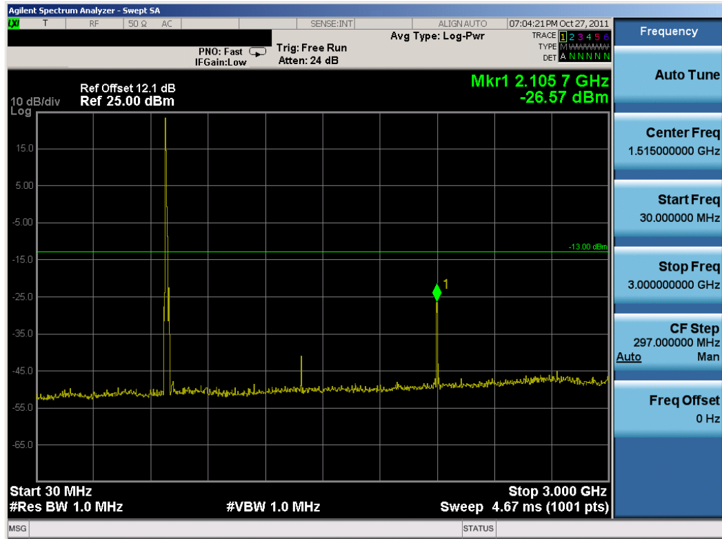
Plot 7-13. Conducted Spurious Plot (Mid Channel)
