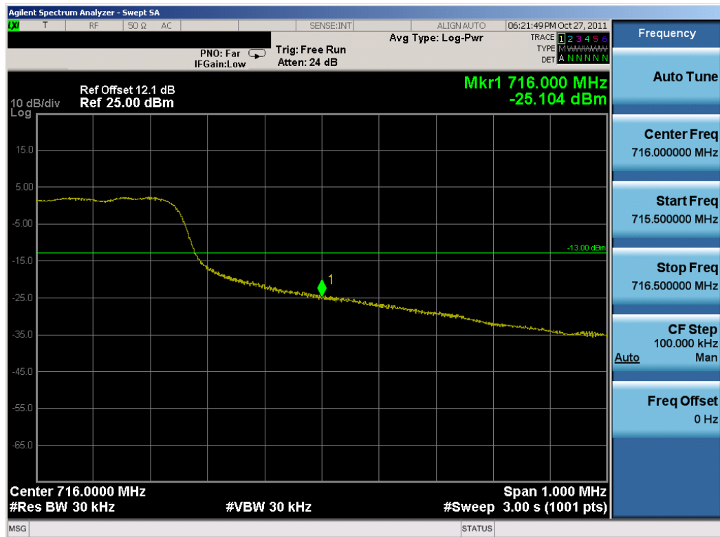
Plot 8-6. Upper Band Edge Plot (QPSK, 25RB)
