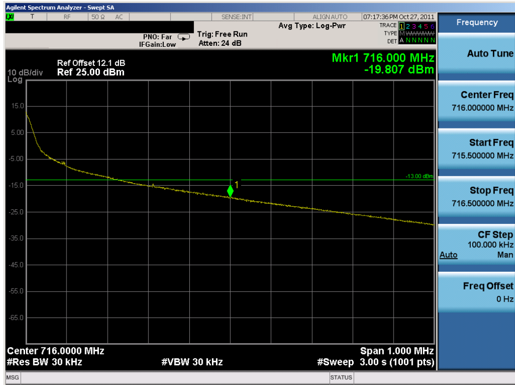
Plot 7-5. Upper Band Edge Plot (QPSK, 1RB, Offset49)
