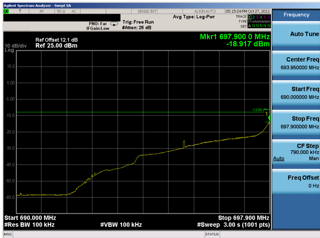
Plot 8-4. Lower Extended Band Edge Plot (QPSK, 25RB)
