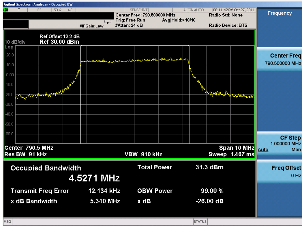
Plot 9-10. Occupied Bandwidth Plot (16QAM, 25RB)
