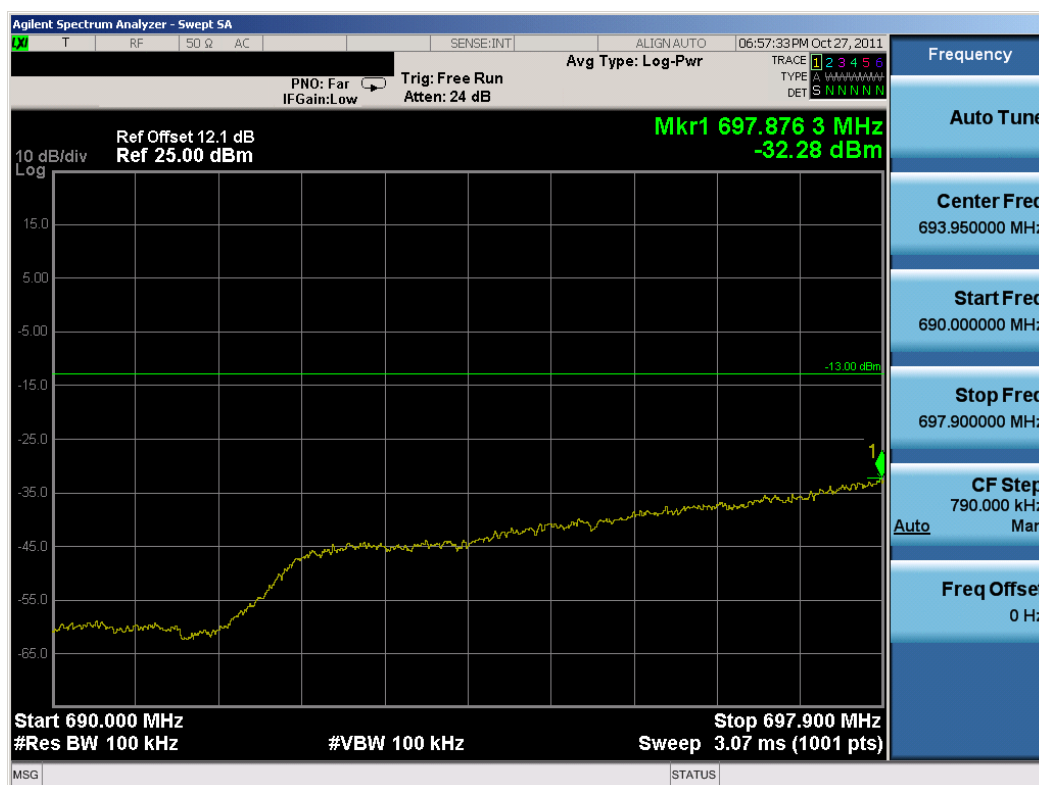
Plot 7-4. Lower Extended Band Edge Plot (QPSK, 50RB)
