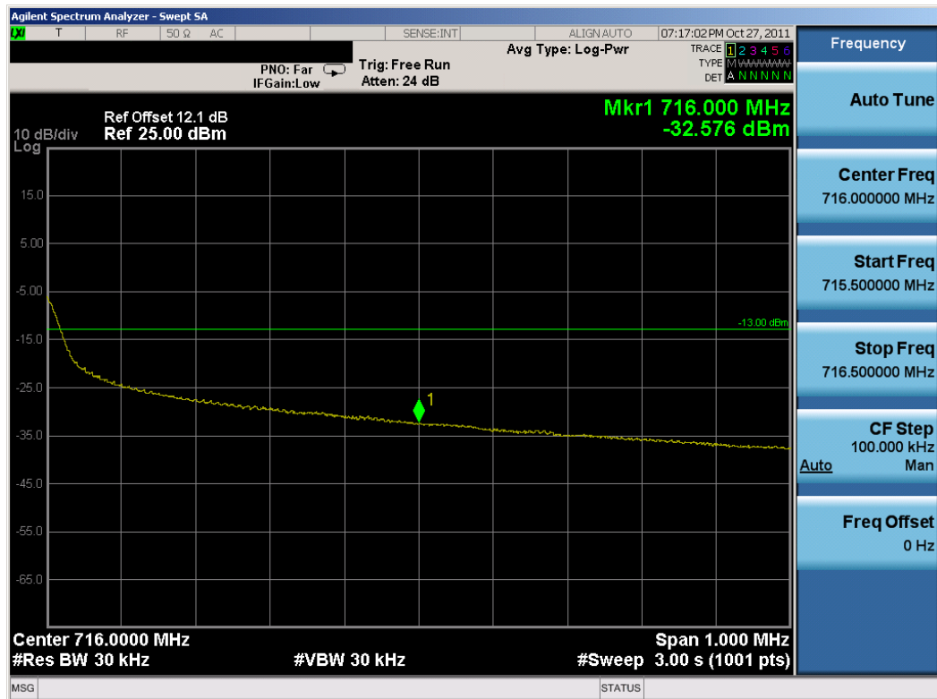
Plot 7-6. Upper Band Edge Plot (QPSK, 50RB)
