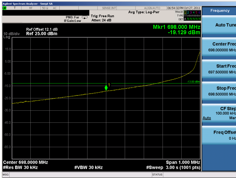
Plot 7-1. Lower Band Edge Plot (QPSK, 1RB, Offset 0)
