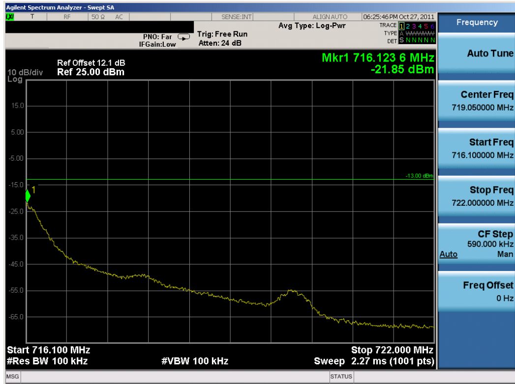
Plot 8-7. Upper Extended Band Edge Plot (QPSK, 1RB, Offset 24)
