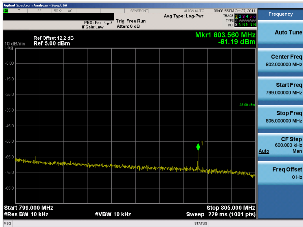
Plot 9-3. Upper Emission Mask 799-805MHz Plot (QPSK, 1RB, Offset 24)
