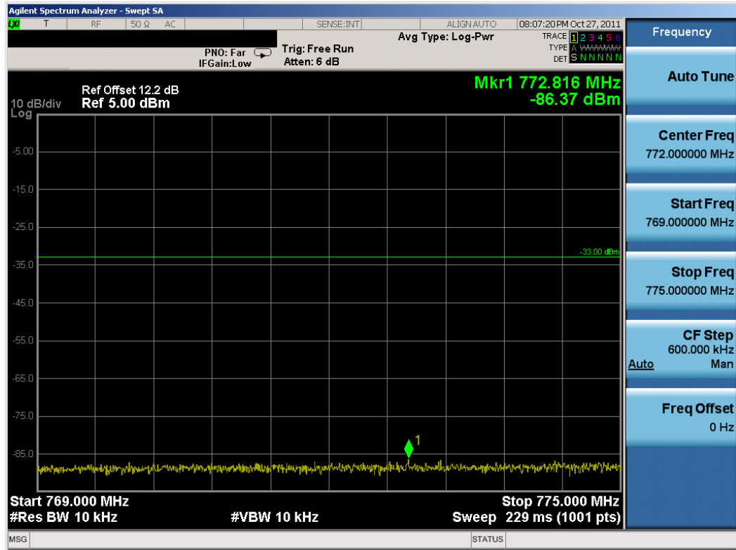
Plot 9-2. Lower Emission Mask 769-775MHz Plot (QPSK, 25RB)
