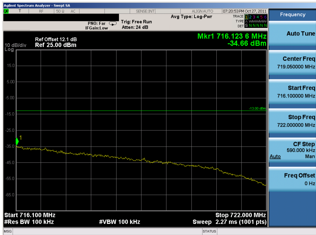
Plot 7-8. Upper Extended Band Edge Plot (QPSK, 50RB)
