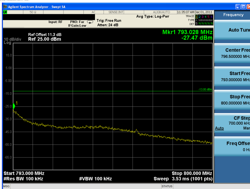
Plot 9-8. Upper Band Edge Plot (QPSK, 25RB)
