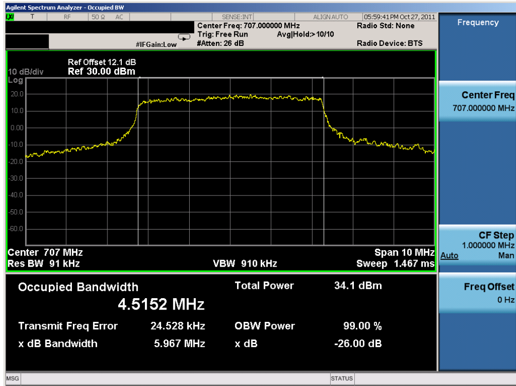
Plot 8-9. Occupied Bandwidth Plot (QPSK, 25RB)
