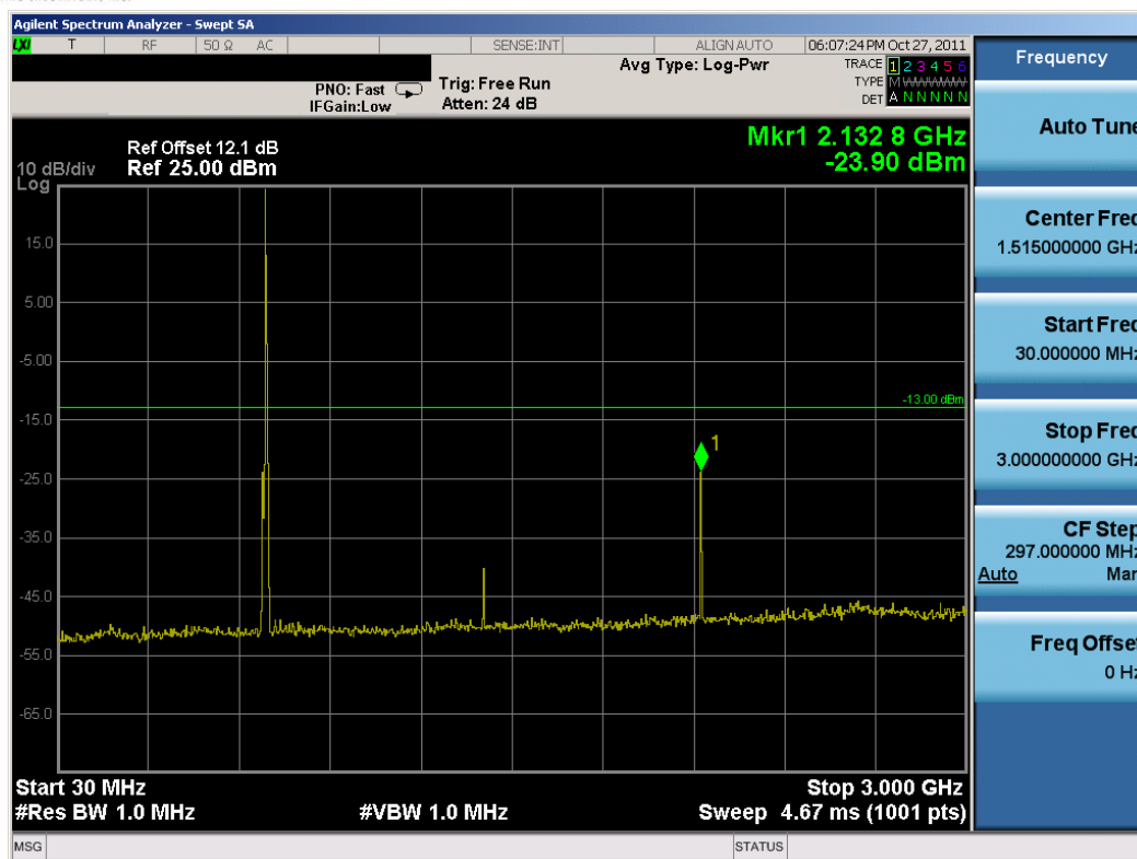
Plot 8-15. Conducted Spurious Plot (High Channel)
