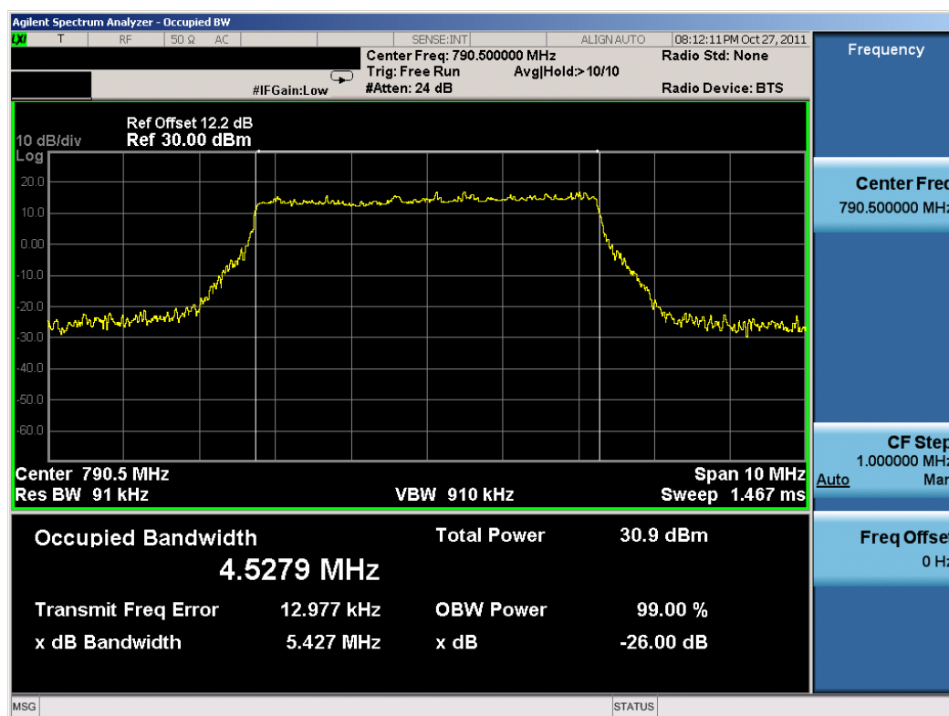
Plot 9-9. Occupied Bandwidth Plot (QPSK, 25RB)
