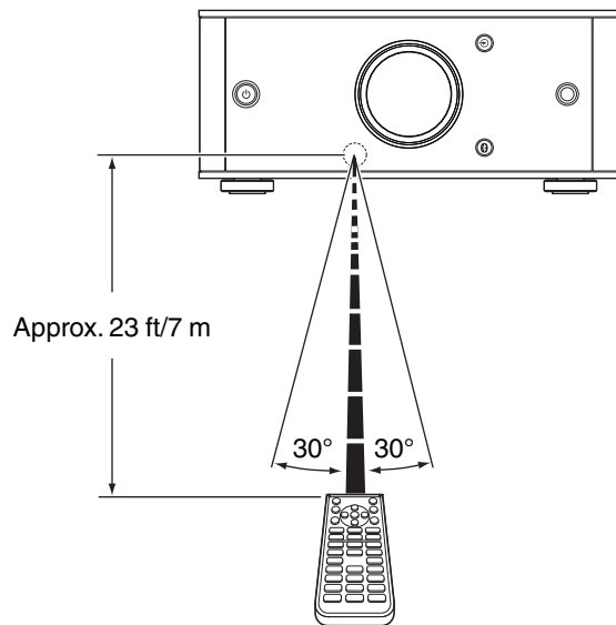
[Horizontal installation]
