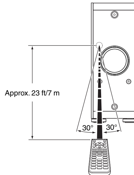
[Vertical installation]
