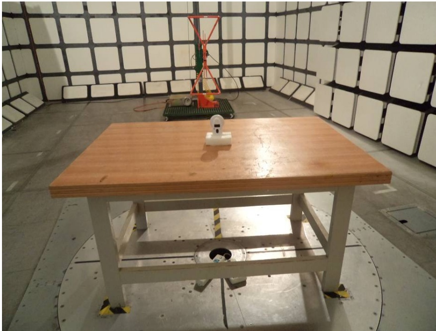
Radiated Emission View (30 MHz to 1 GHz)
