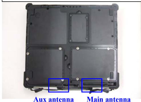
Bottom (Notebook type & Tablet type )
