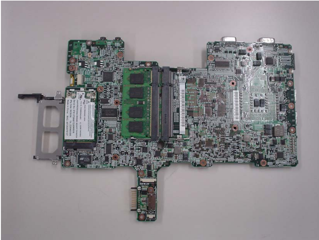
Mother Board (Rear)
