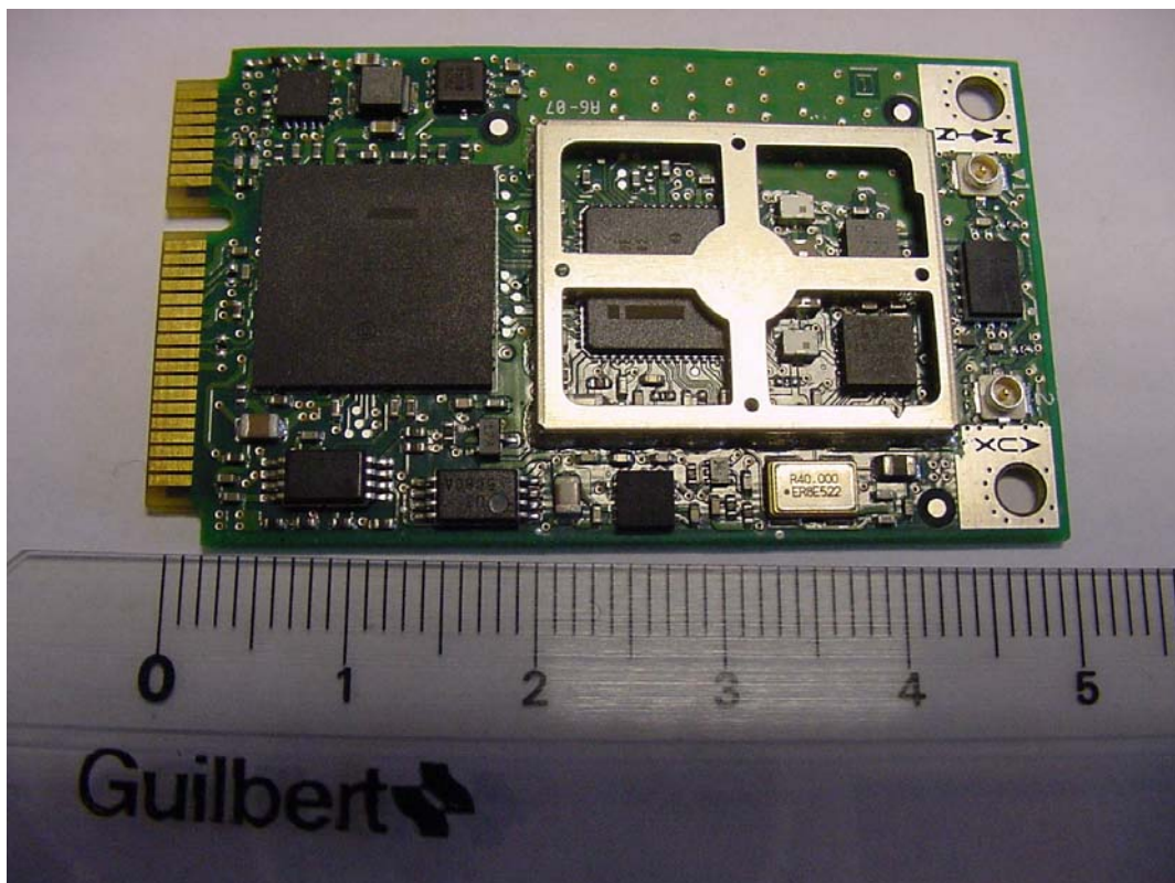
WLAN Board without shield (Front)
