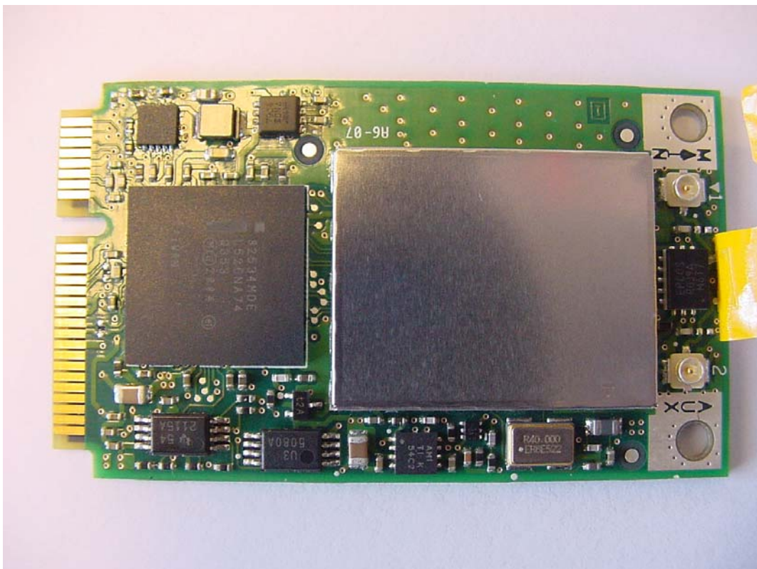
WLAN module (Front)
