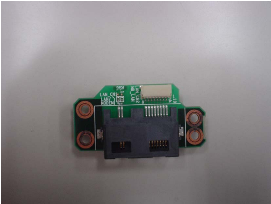
LAN Board (Front)
